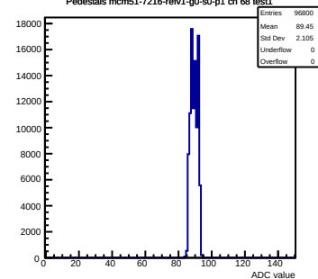
Pedestals mcm51-7216-refv1-g0-s0-p1 ch 68 test1
