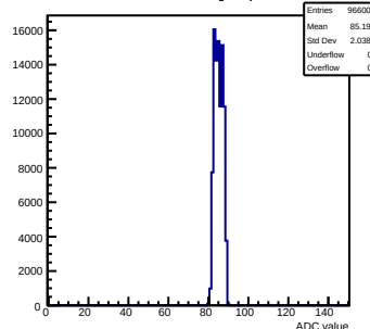
Pedestals mcm51-7216-refv1-g0-s0-p1 ch 107 test1
