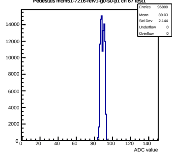
Pedestals mcm51-7216-refv1-g0-s0-p1 ch 67 test1
