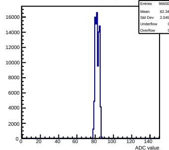
Pedestals mcm51-7216-refv1-g0-s0-p1 ch 99 test1
