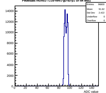
Pedestals mcm51-7216-refv1-g0-s0-p1 ch 64 test1
