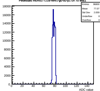
Pedestals mcm51-7216-refv1-g0-s0-p1 ch 70 test1
