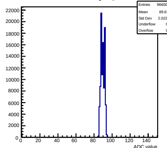
Pedestals mcm51-7216-refv1-g0-s0-p1 ch 111 test1
