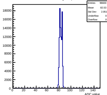
Pedestals mcm51-7216-refv1-g0-s0-p1 ch 106 test1
