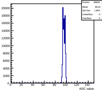
Pedestals mcm51-7216-refv1-g0-s0-p1 ch 97 test1
