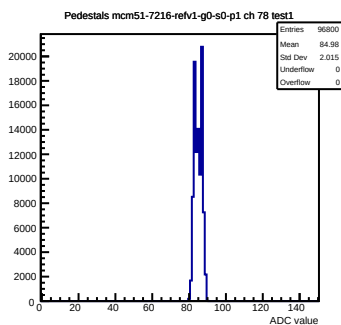
Pedestals mcm51-7216-refv1-g0-s0-p1 ch 78 test1
