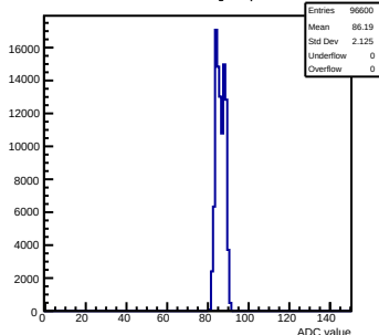
Pedestals mcm51-7216-refv1-g0-s0-p1 ch 104 test1
