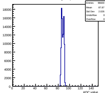
Pedestals mcm51-7216-refv1-g0-s0-p1 ch 110 test1
