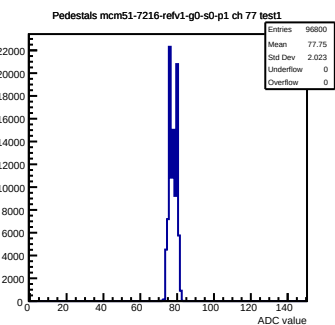
Pedestals mcm51-7216-refv1-g0-s0-p1 ch 77 test1
