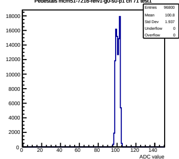
Pedestals mcm51-7216-refv1-g0-s0-p1 ch 71 test1
