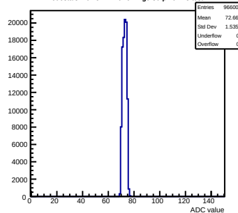
Pedestals mcm51-7216-refv2-g0-s0-p1 ch 43 test1
