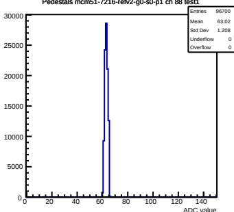
Pedestals mcm51-7216-refV2-g0-s0-p1 ch 88 test1
