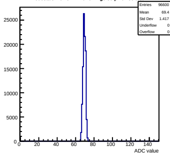
Pedestals mcm51-7216-refv2-g0-s0-p1 ch 38 test1
