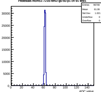
Pedestals mcm51-7216-refV2-g0-s0-p1 ch 91 test1
