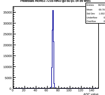
Pedestals mcm51-7216-refV2-g0-s0-p1 ch 89 test1
