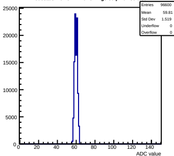
Pedestals mcm51-7216-refv2-g0-s0-p1 ch 36 test1
