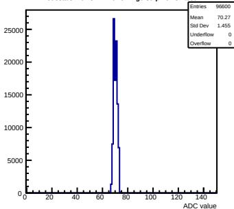
Pedestals mcm51-7216-refv2-g0-s0-p1 ch 32 test1
