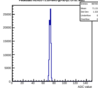
Pedestals mcm51-7216-refV2-g0-s0-p1 ch 81 test1
