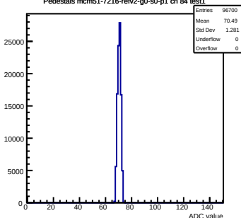
Pedestals mcm51-7216-refV2-g0-s0-p1 ch 84 test1
