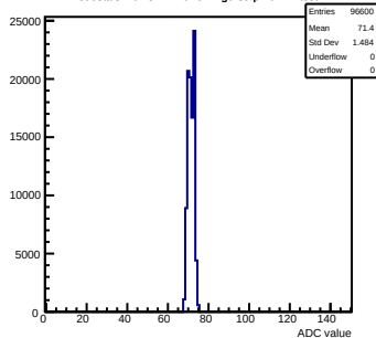
Pedestals mcm51-7216-refv2-g0-s0-p1 ch 41 test1
