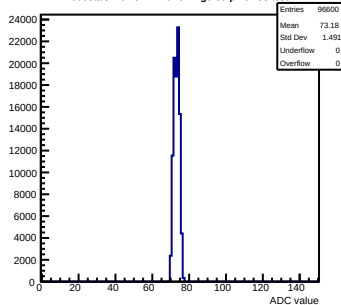
Pedestals mcm51-7216-refv2-g0-s0-p1 ch 33 test1
