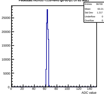
Pedestals mcm51-7216-refV2-g0-s0-p1 ch 83 test1
