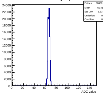
Pedestals mcm51-7216-refv2-g0-s0-p1 ch 42 test1
