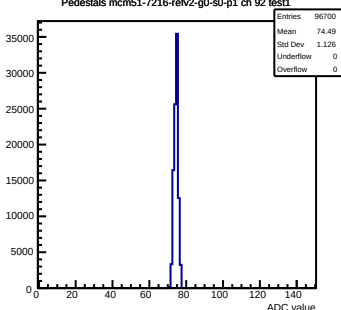
Pedestals mcm51-7216-refV2-g0-s0-p1 ch 92 test1
