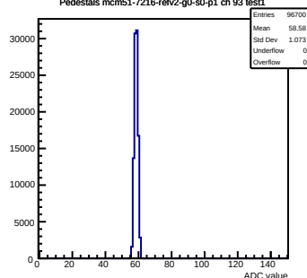
Pedestals mcm51-7216-refV2-g0-s0-p1 ch 93 test1
