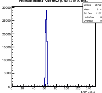
Pedestals mcm51-7216-refV2-g0-s0-p1 ch 90 test1
