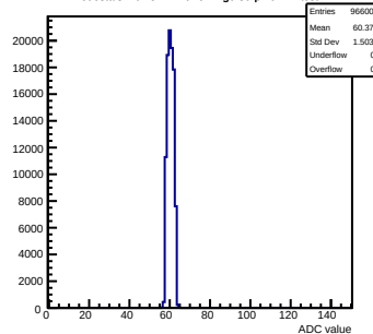
Pedestals mcm51-7216-refv2-g0-s0-p1 ch 47 test1
