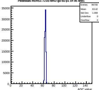
Pedestals mcm51-7216-refV2-g0-s0-p1 ch 95 test1
