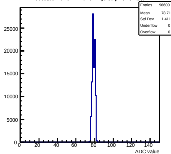
Pedestals mcm51-7216-refv2-g0-s0-p1 ch 34 test1
