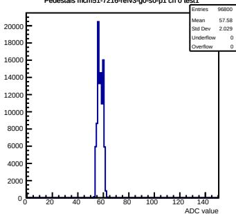
Pedestals mcm51-7216-refv3-g0-s0-p1 ch 0 test1
