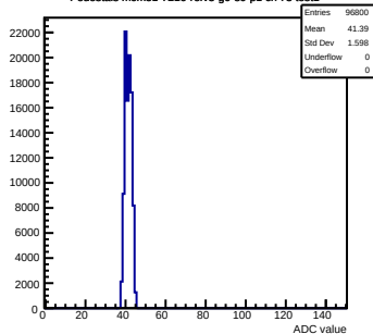
Pedestals mcm51-7216-refv3-g0-s0-p1 ch 73 test1
