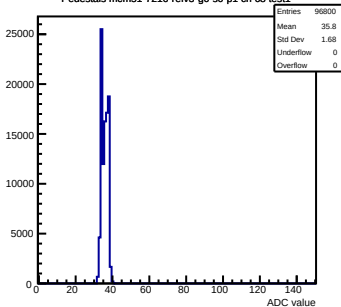
Pedestals mcm51-7216-refv3-g0-s0-p1 ch 68 test1
