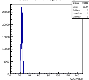
Pedestals mcm51-7216-refv3-g0-s0-p1 ch 77 test1
