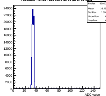
Pedestals mcm51-7216-refv3-g0-s0-p1 ch 66 test1
