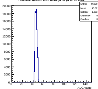
Pedestals mcm51-7216-refv3-g0-s0-p1 ch 10 test1
