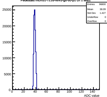
Pedestals mcm51-7216-refv3-g0-s0-p1 ch 1 test1
