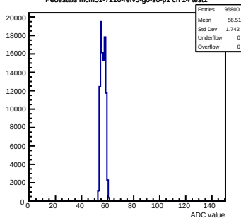
Pedestals mcm51-7216-refv3-g0-s0-p1 ch 14 test1
