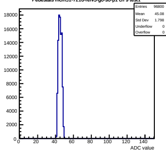
Pedestals mcm51-7216-refv3-g0-s0-p1 ch 9 test1
