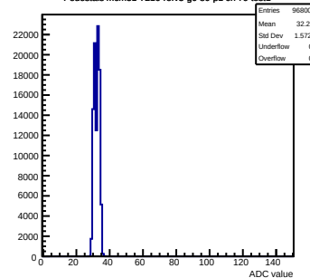
Pedestals mcm51-7216-refv3-g0-s0-p1 ch 79 test1
