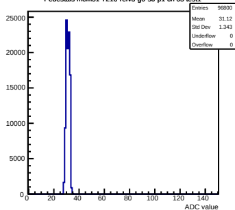
Pedestals mcm51-7216-refv3-g0-s0-p1 ch 65 test1
