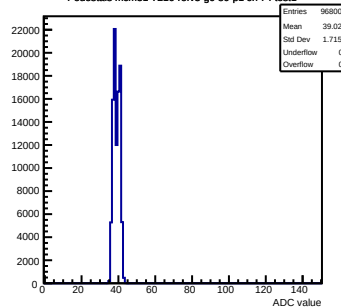
Pedestals mcm51-7216-refv3-g0-s0-p1 ch 74 test1
