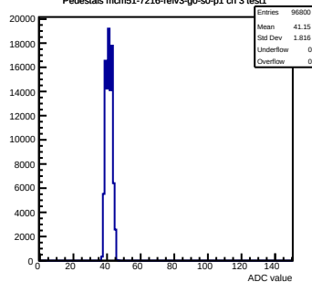
Pedestals mcm51-7216-refv3-g0-s0-p1 ch 3 test1
