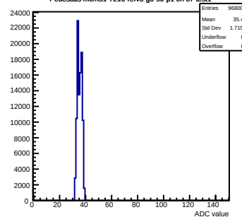
Pedestals mcm51-7216-refv3-g0-s0-p1 ch 67 test1
