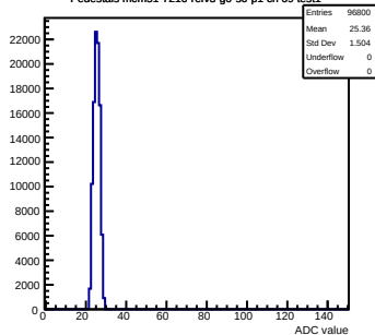
Pedestals mcm51-7216-refv3-g0-s0-p1 ch 69 test1
