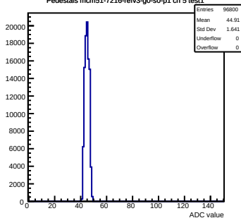
Pedestals mcm51-7216-refv3-g0-s0-p1 ch 5 test1
