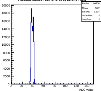
Pedestals mcm51-7216-refv3-g0-s0-p1 ch 64 test1
