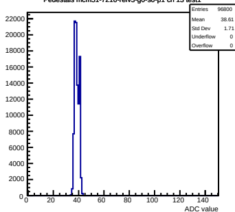
Pedestals mcm51-7216-refv3-g0-s0-p1 ch 13 test1
