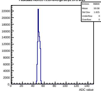
Pedestals mcm51-7216-refv3-g0-s0-p1 ch 8 test1
