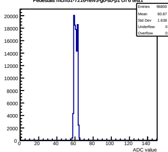
Pedestals mcm51-7216-refv3-g0-s0-p1 ch 6 test1
