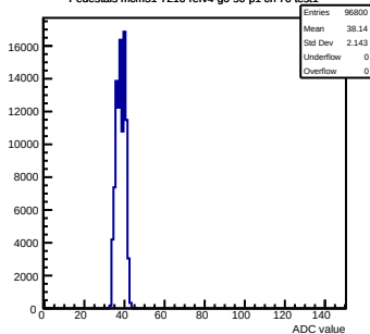
Pedestals mcm51-7216-refv4-g0-s0-p1 ch 70 test1
