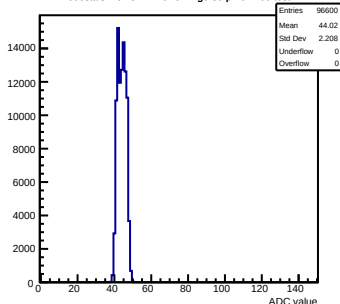
Pedestals mcm51-7216-refv4-g0-s0-p1 ch 106 test1
