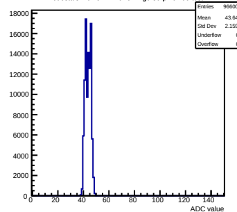
Pedestals mcm51-7216-refv4-g0-s0-p1 ch 99 test1
