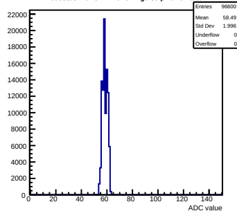
Pedestals mcm51-7216-refv4-g0-s0-p1 ch 97 test1
