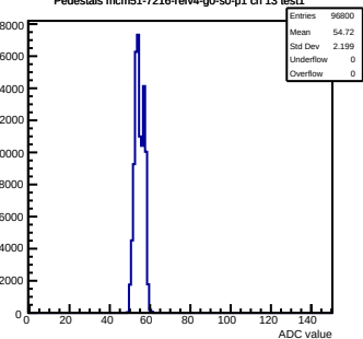
Pedestals mcm51-7216-refv4-g0-s0-p1 ch 13 test1
