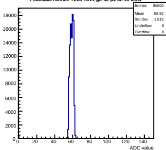
Pedestals mcm51-7216-refv4-g0-s0-p1 ch 49 test1
