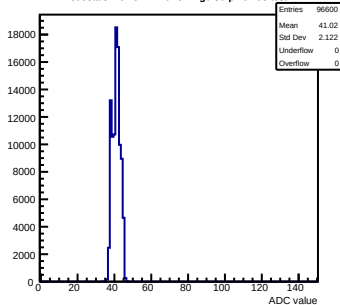
Pedestals mcm51-7216-refv4-g0-s0-p1 ch 98 test1
