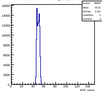
Pedestals mcm51-7216-refv4-g0-s0-p1 ch 108 test1
