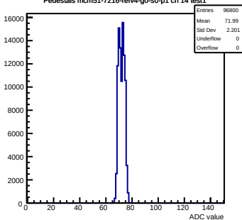
Pedestals mcm51-7216-refv4-g0-s0-p1 ch 14 test1
