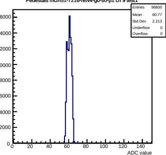
Pedestals mcm51-7216-refv4-g0-s0-p1 ch 9 test1
