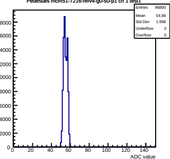
Pedestals mcm51-7216-refv4-g0-s0-p1 ch 1 test1
