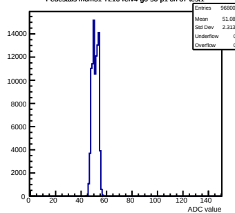
Pedestals mcm51-7216-refv4-g0-s0-p1 ch 67 test1
