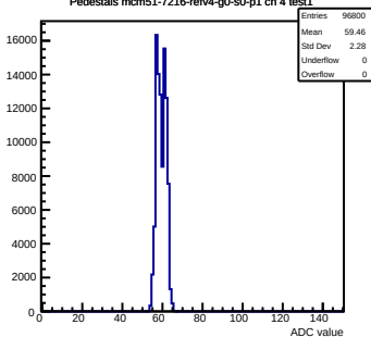
Pedestals mcm51-7216-refv4-g0-s0-p1 ch 4 test1
