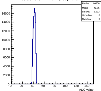
Pedestals mcm51-7216-refv4-g0-s0-p1 ch 60 test1
