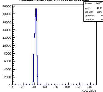
Pedestals mcm51-7216-refv4-g0-s0-p1 ch 51 test1
