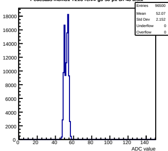
Pedestals mcm51-7216-refv4-g0-s0-p1 ch 48 test1
