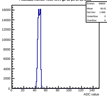
Pedestals mcm51-7216-refv4-g0-s0-p1 ch 65 test1
