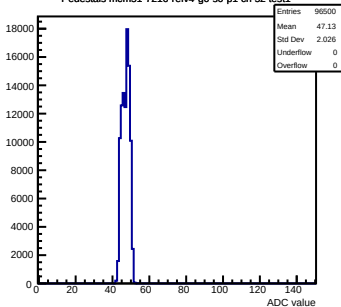
Pedestals mcm51-7216-refv4-g0-s0-p1 ch 52 test1
