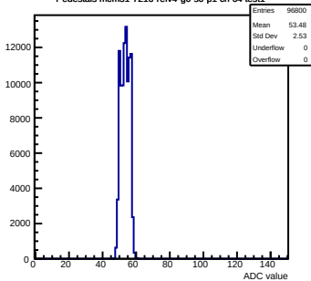
Pedestals mcm51-7216-refv4-g0-s0-p1 ch 64 test1
