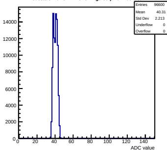
Pedestals mcm51-7216-refv4-g0-s0-p1 ch 100 test1
