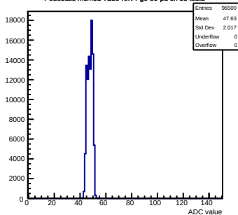
Pedestals mcm51-7216-refv4-g0-s0-p1 ch 58 test1
