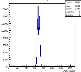
Pedestals mcm51-7216-refv4-g0-s0-p1 ch 96 test1
