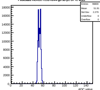
Pedestals mcm51-7216-refv4-g0-s0-p1 ch 72 test1
