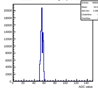
Pedestals mcm51-7216-refv4-g0-s0-p1 ch 103 test1
