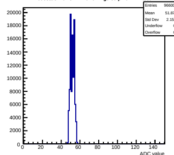
Pedestals mcm51-7216-refv4-g0-s0-p1 ch 111 test1
