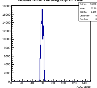
Pedestals mcm51-7216-refv4-g0-s0-p1 ch 11 test1
