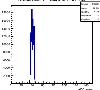
Pedestals mcm51-7216-refv4-g0-s0-p1 ch 77 test1
