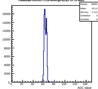
Pedestals mcm51-7216-refv4-g0-s0-p1 ch 15 test1
