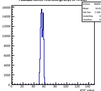
Pedestals mcm51-7216-refv4-g0-s0-p1 ch 74 test1
