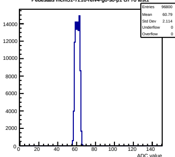
Pedestals mcm51-7216-refv4-g0-s0-p1 ch 76 test1
