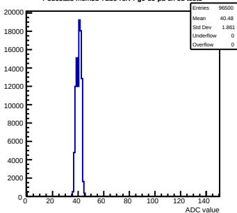
Pedestals mcm51-7216-refv4-g0-s0-p1 ch 61 test1
