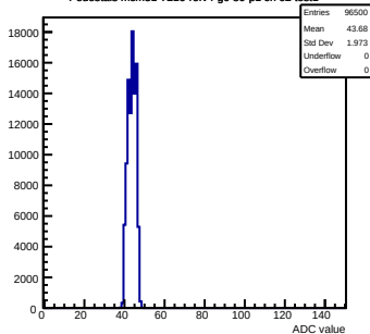
Pedestals mcm51-7216-refv4-g0-s0-p1 ch 62 test1
