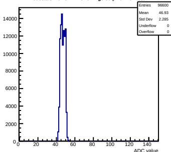
Pedestals mcm51-7216-refv4-g0-s0-p1 ch 104 test1
