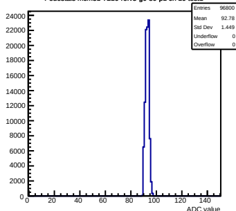
Pedestals mcm51-7216-refv5-g0-s0-p1 ch 10 test1
