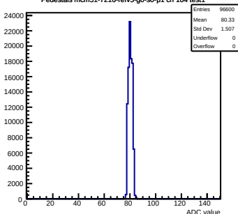
Pedestals mcm51-7216-refV5-g0-s0-p1 ch 104 test1
