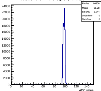
Pedestals mcm51-7216-refv5-g0-s0-p1 ch 8 test1
