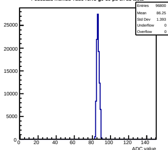
Pedestals mcm51-7216-refv5-g0-s0-p1 ch 13 test1
