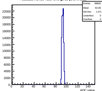
Pedestals mcm51-7216-refv5-g0-s0-p1 ch 9 test1
