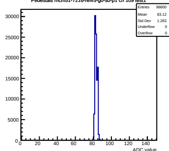
Pedestals mcm51-7216-refV5-g0-s0-p1 ch 109 test1
