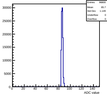
Pedestals mcm51-7216-refv5-g0-s0-p1 ch 1 test1
