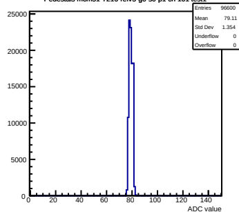
Pedestals mcm51-7216-refV5-g0-s0-p1 ch 101 test1
