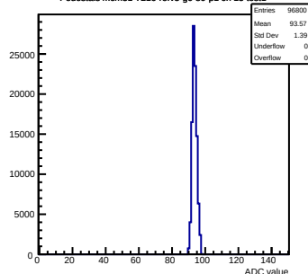
Pedestals mcm51-7216-refv5-g0-s0-p1 ch 15 test1
