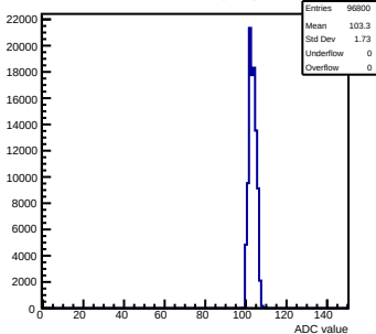
Pedestals mcm51-7216-refv5-g0-s0-p1 ch 0 test1
