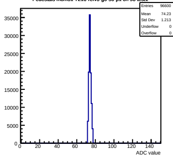
Pedestals mcm51-7216-refV5-g0-s0-p1 ch 98 test1
