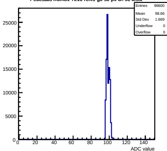
Pedestals mcm51-7216-refV5-g0-s0-p1 ch 96 test1
