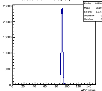
Pedestals mcm51-7216-refv5-g0-s0-p1 ch 11 test1
