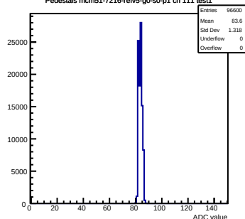
Pedestals mcm51-7216-refV5-g0-s0-p1 ch 111 test1
