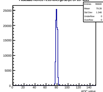
Pedestals mcm51-7216-refV5-g0-s0-p1 ch 107 test1
