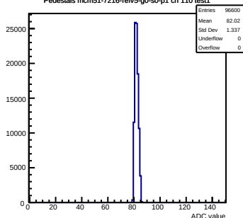
Pedestals mcm51-7216-refV5-g0-s0-p1 ch 110 test1
