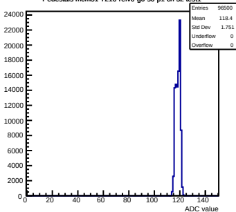
Pedestals mcm51-7216-refv6-g0-s0-p1 ch 52 test1
