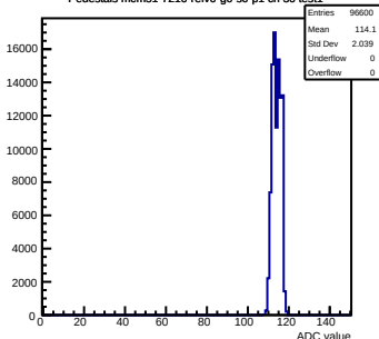
Pedestals mcm51-7216-rlv6-g0-s0-p1 ch 36 test1
