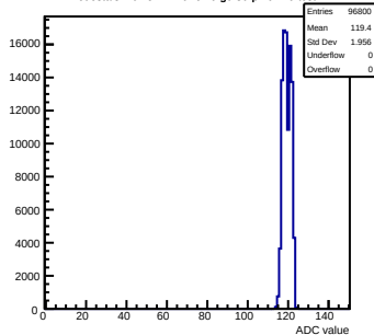
Pedestals mcm51-7216-rlv6-g0-s0-p1 ch 79 test1
