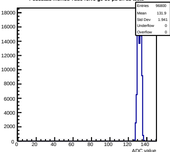
Pedestals mcm51-7216-rlv6-g0-s0-p1 ch 15 test1
