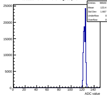
Pedestals mcm51-7216-refv6-g0-s0-p1 ch 117 test1
