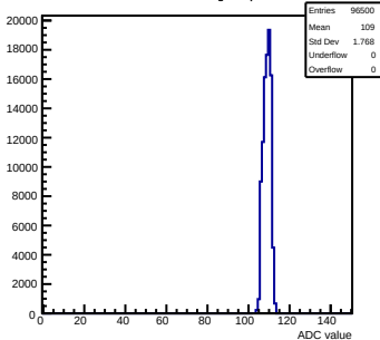
Pedestals mcm51-7216-refv6-g0-s0-p1 ch 124 test1
