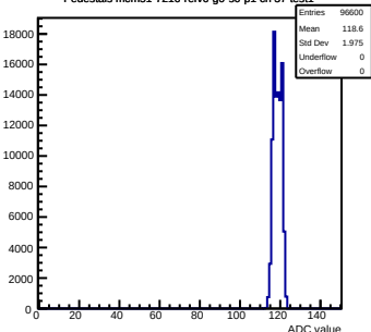
Pedestals mcm51-7216-rlv6-g0-s0-p1 ch 37 test1
