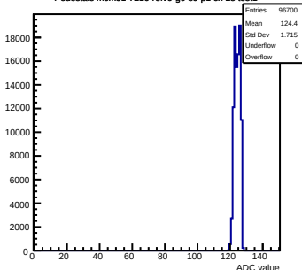
Pedestals mcm51-7216- rev6-g0-s0-p1 ch 28 test1
