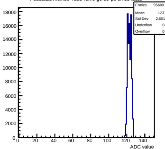
Pedestals mcm51-7216-rlv6-g0-s0-p1 ch 35 test1
