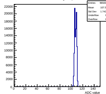
Pedestals mcm51-7216-refv6-g0-s0-p1 ch 126 test1
