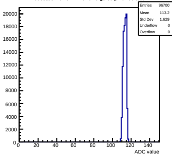
Pedestals mcm51-7216-refv6-g0-s0-p1 ch 93 test1
