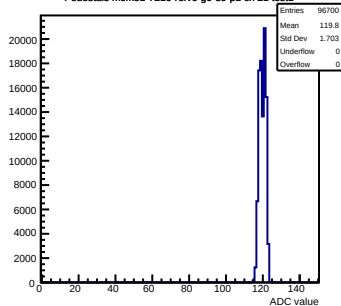
Pedestals mcm51-7216- rev6-g0-s0-p1 ch 21 test1
