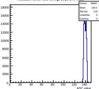
Pedestals mcm51-7216-rlv6-g0-s0-p1 ch 14 test1
