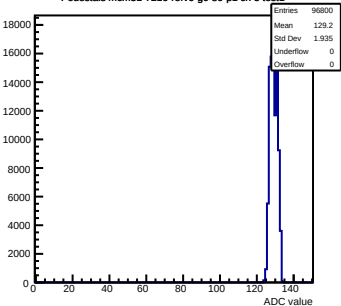
Pedestals mcm51-7216-rlv6-g0-s0-p1 ch 5 test1
