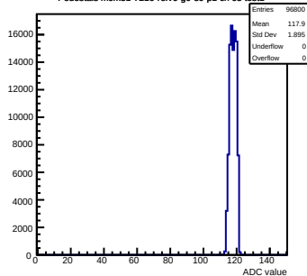
Pedestals mcm51-7216-rlv6-g0-s0-p1 ch 65 test1
