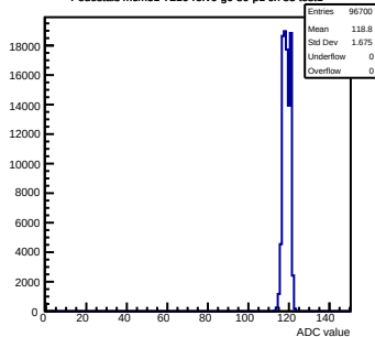
Pedestals mcm51-7216-refv6-g0-s0-p1 ch 83 test1
