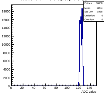
Pedestals mcm51-7216-rlv6-g0-s0-p1 ch 32 test1
