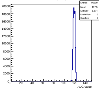
Pedestals mcm51-7216-refv6-g0-s0-p1 ch 120 test1
