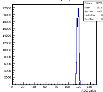
Pedestals mcm51-7216-refv6-g0-s0-p1 ch 95 test1
