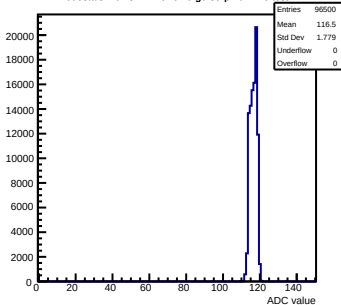
Pedestals mcm51-7216-refv6-g0-s0-p1 ch 116 test1
