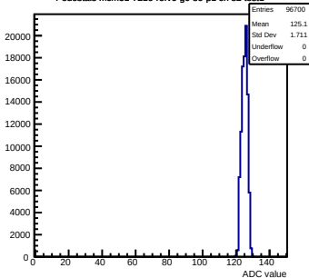
Pedestals mcm51-7216-refv6-g0-s0-p1 ch 82 test1
