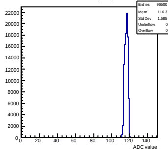
Pedestals mcm51-7216-refv6-g0-s0-p1 ch 121 test1
