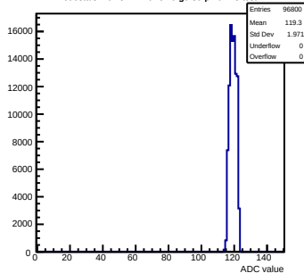
Pedestals mcm51-7216-rlv6-g0-s0-p1 ch 75 test1
