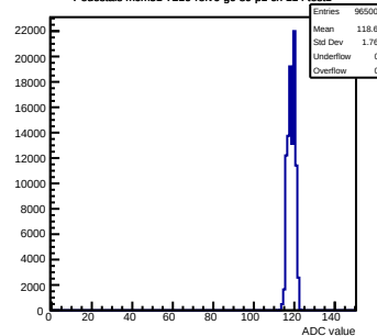
Pedestals mcm51-7216-refv6-g0-s0-p1 ch 114 test1
