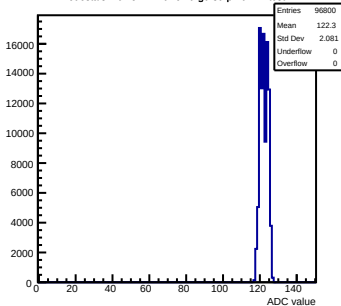
Pedestals mcm51-7216-rlv6-g0-s0-p1 ch 72 test1
