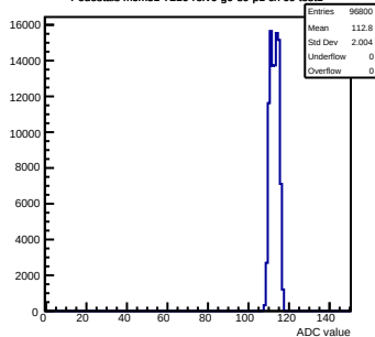
Pedestals mcm51-7216-rlv6-g0-s0-p1 ch 69 test1
