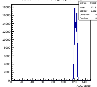
Pedestals mcm51-7216-rlv6-g0-s0-p1 ch 67 test1
