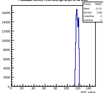
Pedestals mcm51-7216-rlv6-g0-s0-p1 ch 44 test1
