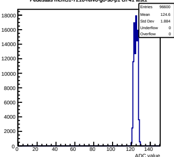
Pedestals mcm51-7216-rlv6-g0-s0-p1 ch 41 test1
