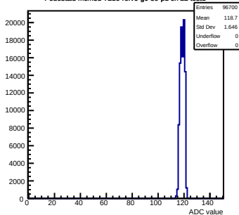
Pedestals mcm51-7216- rev6-g0-s0-p1 ch 22 test1
