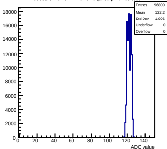
Pedestals mcm51-7216-rlv6-g0-s0-p1 ch 68 test1
