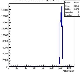
Pedestals mcm51-7216- rev6-g0-s0-p1 ch 20 test1
