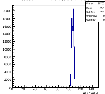
Pedestals mcm51-7216- rev6-g0-s0-p1 ch 29 test1
