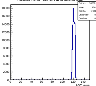
Pedestals mcm51-7216-rlv6-g0-s0-p1 ch 39 test1
