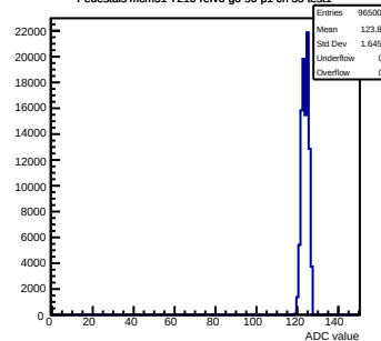
Pedestals mcm51-7216-refv6-g0-s0-p1 ch 55 test1
