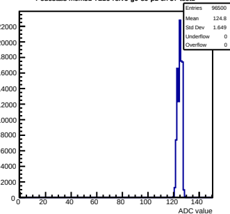
Pedestals mcm51-7216-refv6-g0-s0-p1 ch 57 test1
