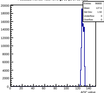
Pedestals mcm51-7216-rlv6-g0-s0-p1 ch 11 test1
