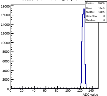
Pedestals mcm51-7216-rlv6-g0-s0-p1 ch 1 test1
