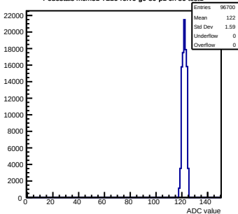
Pedestals mcm51-7216-refv6-g0-s0-p1 ch 86 test1
