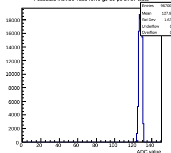
Pedestals mcm51-7216- rev6-g0-s0-p1 ch 27 test1
