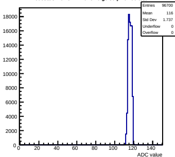
Pedestals mcm51-7216-refv6-g0-s0-p1 ch 90 test1
