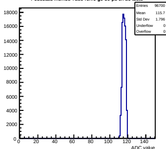
Pedestals mcm51-7216- rev6-g0-s0-p1 ch 26 test1
