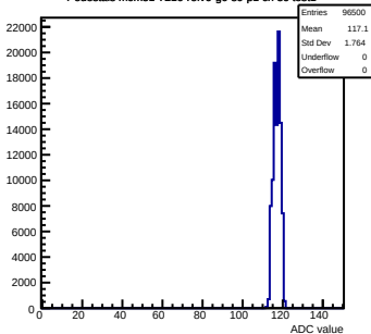
Pedestals mcm51-7216-refv6-g0-s0-p1 ch 56 test1
