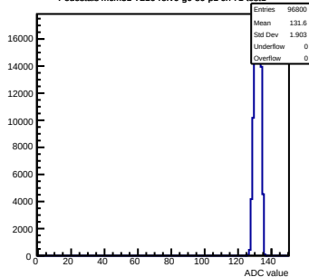
Pedestals mcm51-7216-rlv6-g0-s0-p1 ch 71 test1
