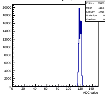
Pedestals mcm51-7216-rlv6-g0-s0-p1 ch 78 test1
