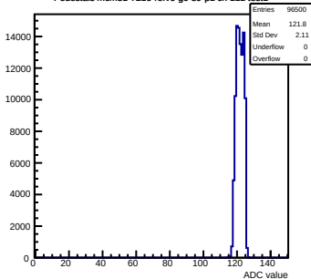
Pedestals mcm51-7216-refv6-g0-s0-p1 ch 112 test1
