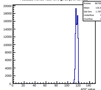
Pedestals mcm51-7216- rev6-g0-s0-p1 ch 31 test1
