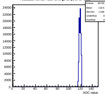
Pedestals mcm51-7216-refv6-g0-s0-p1 ch 87 test1
