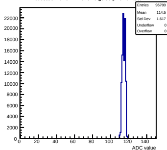
Pedestals mcm51-7216-refv6-g0-s0-p1 ch 91 test1
