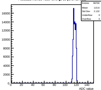
Pedestals mcm51-7216-refv6-g0-s0-p1 ch 80 test1
