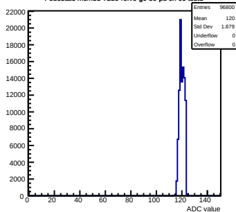
Pedestals mcm51-7216-rlv6-g0-s0-p1 ch 66 test1
