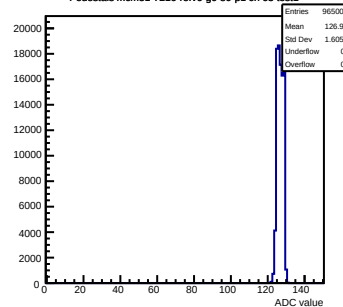
Pedestals mcm51-7216-refv6-g0-s0-p1 ch 63 test1
