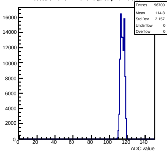
Pedestals mcm51-7216- rev6-g0-s0-p1 ch 16 test1
