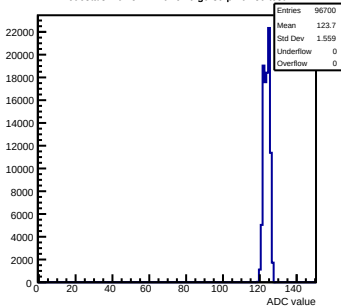
Pedestals mcm51-7216-refv6-g0-s0-p1 ch 89 test1
