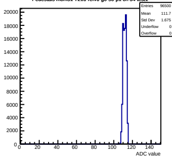
Pedestals mcm51-7216-refv6-g0-s0-p1 ch 54 test1
