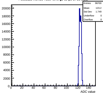
Pedestals mcm51-7216-refv6-g0-s0-p1 ch 81 test1
