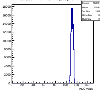
Pedestals mcm51-7216-rlv6-g0-s0-p1 ch 70 test1
