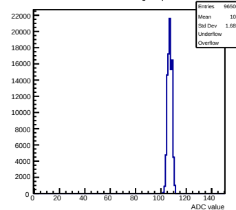
Pedestals mcm51-7216-refv6-g0-s0-p1 ch 127 test1
