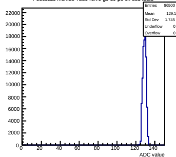
Pedestals mcm51-7216-refv6-g0-s0-p1 ch 113 test1
