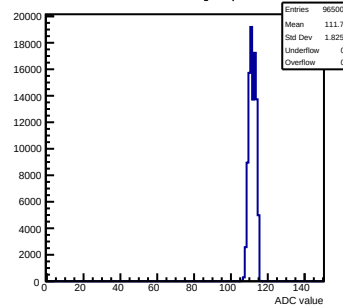
Pedestals mcm51-7216-refv6-g0-s0-p1 ch 122 test1
