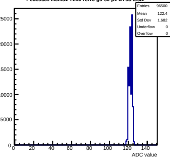
Pedestals mcm51-7216-refv6-g0-s0-p1 ch 53 test1
