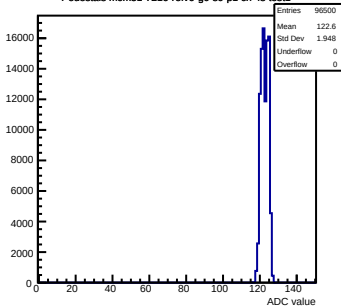
Pedestals mcm51-7216-refv6-g0-s0-p1 ch 48 test1
