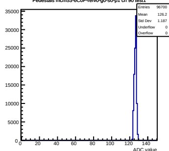
Pedestals mcm53-6C0F-rev0-g0-s0-p1 ch 90 test1
