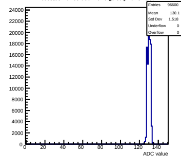
Pedestals mcm53-6C0F-rev0-g0-s0-p1 ch 32 test1
