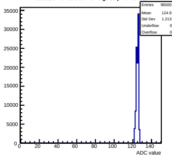
Pedestals mcm53-6C0F-rev0-g0-s0-p1 ch 50 test1
