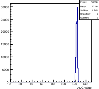
Pedestals mcm53-6C0F-rev0-g0-s0-p1 ch 60 test1
