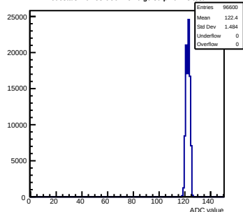
Pedestals mcm53-6C0F-rev0-g0-s0-p1 ch 43 test1
