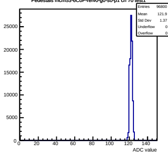
Pedestals mcm53-6CDF-rev0-g0-s0-p1 ch 70 test1
