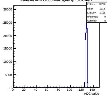
Pedestals mcm53-6C0F-rev0-g0-s0-p1 ch 85 test1
