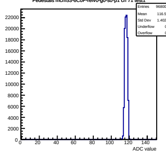
Pedestals mcm53-6CDF-rev0-g0-s0-p1 ch 71 test1
