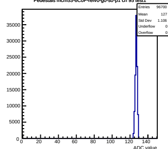
Pedestals mcm53-6C0F-rev0-g0-s0-p1 ch 95 test1
