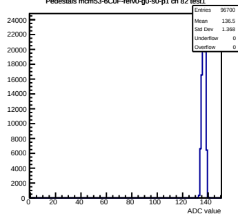
Pedestals mcm53-6C0F-rev0-g0-s0-p1 ch 82 test1
