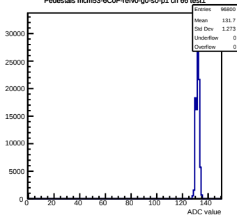
Pedestals mcm53-6CDF-rev0-g0-s0-p1 ch 66 test1
