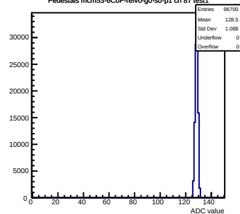
Pedestals mcm53-6C0F-rev0-g0-s0-p1 ch 87 test1
