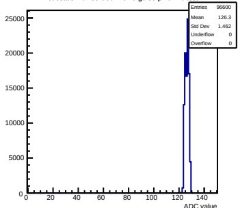
Pedestals mcm53-6C0F-rev0-g0-s0-p1 ch 46 test1
