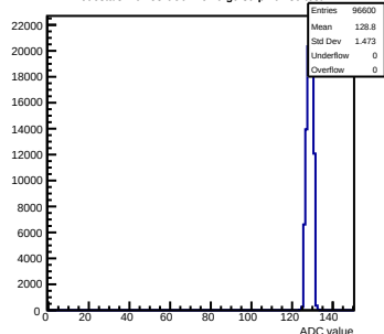
Pedestals mcm53-6C0F-rev0-g0-s0-p1 ch 39 test1
