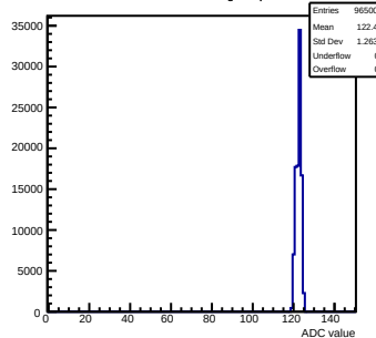
Pedestals mcm53-6C0F-rev0-g0-s0-p1 ch 59 test1
