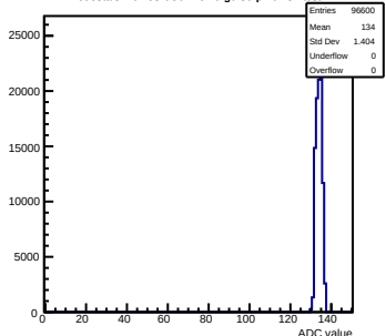
Pedestals mcm53-6C0F-rev0-g0-s0-p1 ch 37 test1
