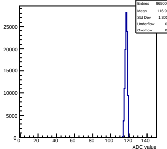
Pedestals mcm53-6C0F-rev0-g0-s0-p1 ch 54 test1
