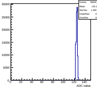
Pedestals mcm53-6C0F-rev0-g0-s0-p1 ch 53 test1
