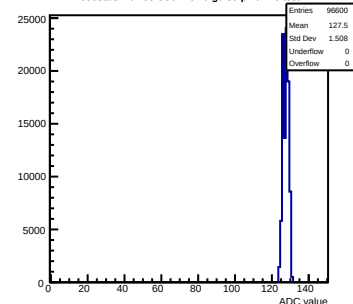
Pedestals mcm53-6C0F-rev0-g0-s0-p1 ch 40 test1
