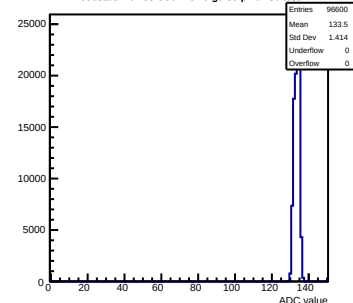
Pedestals mcm53-6C0F-rev0-g0-s0-p1 ch 36 test1
