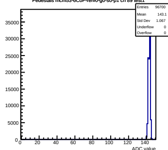
Pedestals mcm53-6C0F-rev0-g0-s0-p1 ch 89 test1
