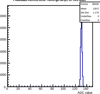
Pedestals mcm53-6C0F-refV0-g0-s0-p1 ch 126 test1
