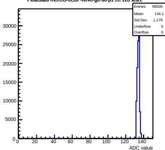
Pedestals mcm53-6C0F-refV0-g0-s0-p1 ch 120 test1
