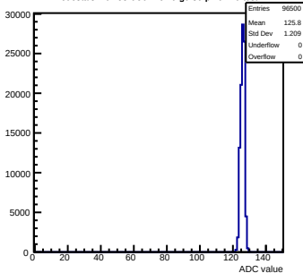
Pedestals mcm53-6C0F-rev0-g0-s0-p1 ch 49 test1
