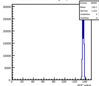
Pedestals mcm53-6C0F-rev0-g0-s0-p1 ch 47 test1
