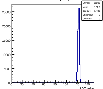
Pedestals mcm53-6C0F-rev0-g0-s0-p1 ch 38 test1
