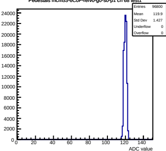
Pedestals mcm53-6CDF-rev0-g0-s0-p1 ch 68 test1
