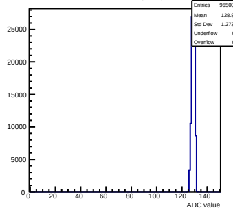
Pedestals mcm53-6C0F-rev0-g0-s0-p1 ch 55 test1
