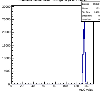
Pedestals mcm53-6CDF-rev0-g0-s0-p1 ch 78 test1
