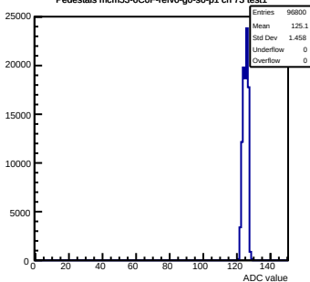
Pedestals mcm53-6CDF-rev0-g0-s0-p1 ch 73 test1
