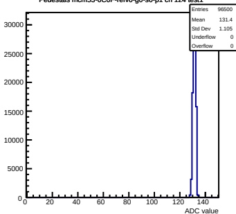
Pedestals mcm53-6C0F-refV0-g0-s0-p1 ch 124 test1
