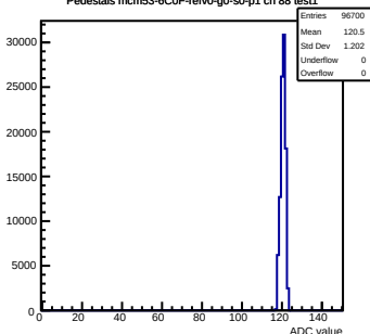
Pedestals mcm53-6C0F-rev0-g0-s0-p1 ch 88 test1
