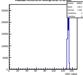
Pedestals mcm53-6CDF-rev0-g0-s0-p1 ch 69 test1
