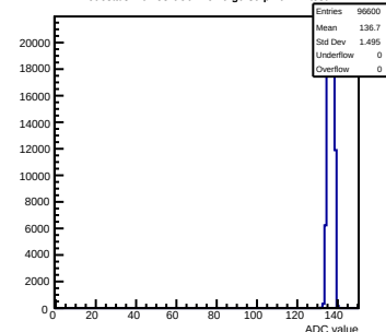
Pedestals mcm53-6C0F-rev0-g0-s0-p1 ch 44 test1
