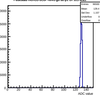
Pedestals mcm53-6C0F-refV0-g0-s0-p1 ch 123 test1
