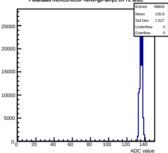
Pedestals mcm53-6CDF-rev0-g0-s0-p1 ch 72 test1
