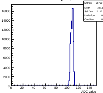
Pedestals mcm53-6C0F-refv1-g0-s0-p1 ch 82 test1
