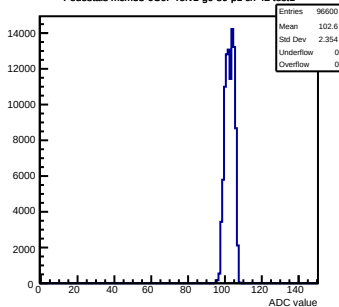
Pedestals mcm53-6C0F-refv1-g0-s0-p1 ch 42 test1
