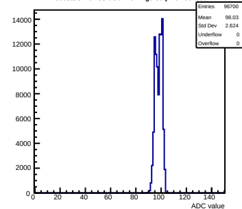
Pedestals mcm53-6C0F-refv1-g0-s0-p1 ch 80 test1
