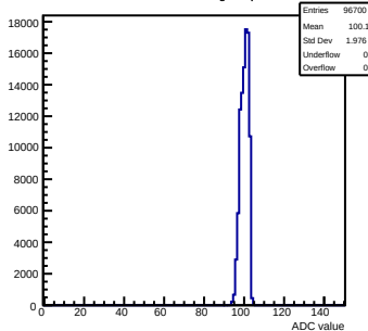
Pedestals mcm53-6C0F-refv1-g0-s0-p1 ch 91 test1
