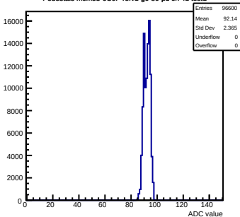
Pedestals mcm53-6C0F-refv1-g0-s0-p1 ch 41 test1
