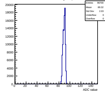
Pedestals mcm53-6C0F-refv1-g0-s0-p1 ch 88 test1
