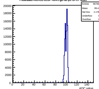
Pedestals mcm53-6C0F-refV1-g0-s0-p1 ch 27 test1
