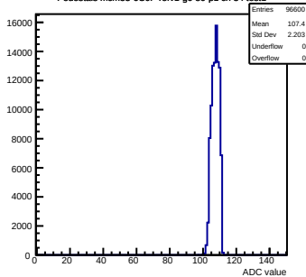
Pedestals mcm53-6C0F-refv1-g0-s0-p1 ch 34 test1
