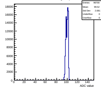
Pedestals mcm53-6C0F-refv1-g0-s0-p1 ch 92 test1
