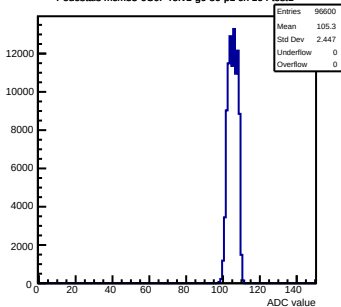
Pedestals mcm53-6C0F-refV1-g0-s0-p1 ch 104 test1
