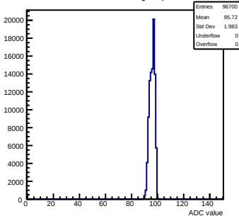
Pedestals mcm53-6C0F-refv1-g0-s0-p1 ch 90 test1
