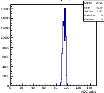
Pedestals mcm53-6C0F-refv1-g0-s0-p1 ch 81 test1
