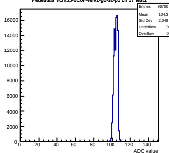
Pedestals mcm53-6C0F-refV1-g0-s0-p1 ch 17 test1
