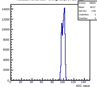
Pedestals mcm53-6C0F-refV1-g0-s0-p1 ch 96 test1
