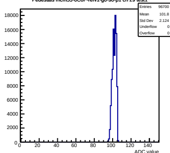
Pedestals mcm53-6C0F-refV1-g0-s0-p1 ch 29 test1
