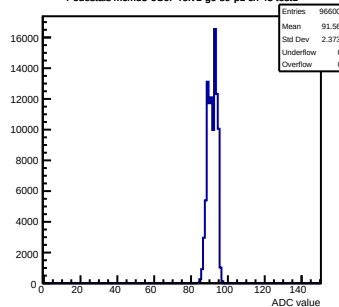
Pedestals mcm53-6C0F-refv1-g0-s0-p1 ch 43 test1
