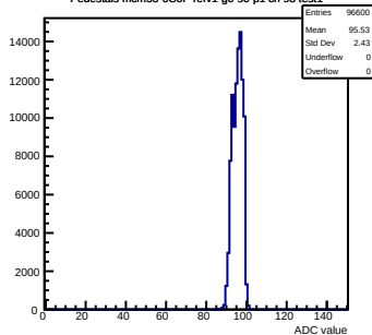
Pedestals mcm53-6C0F-refV1-g0-s0-p1 ch 98 test1
