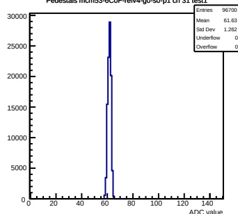
Pedestals mcm53-6CDF-refv4-g0-s0-p1 ch 31 test1
