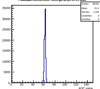
Pedestals mcm53-6CDF-refv4-g0-s0-p1 ch 25 test1
