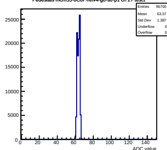
Pedestals mcm53-6CDF-refv4-g0-s0-p1 ch 27 test1
