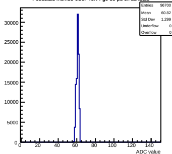
Pedestals mcm53-6CDF-refv4-g0-s0-p1 ch 22 test1
