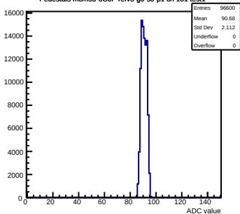
Pedestals mcm53-6C0F-refV5-g0-s0-p1 ch 101 test1
