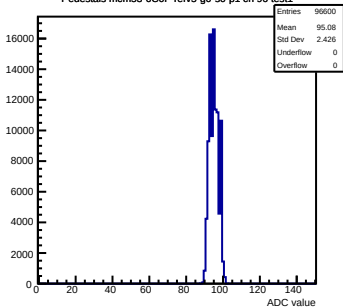
Pedestals mcm53-6C0F-refV5-g0-s0-p1 ch 96 test1
