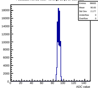
Pedestals mcm53-6C0F-refV5-g0-s0-p1 ch 106 test1
