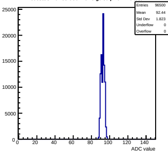
Pedestals mcm53-6C0F-refV5-g0-s0-p1 ch 126 test1
