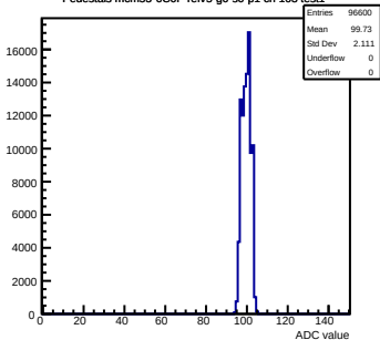
Pedestals mcm53-6C0F-refV5-g0-s0-p1 ch 103 test1
