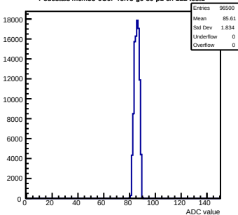
Pedestals mcm53-6C0F-refV5-g0-s0-p1 ch 122 test1
