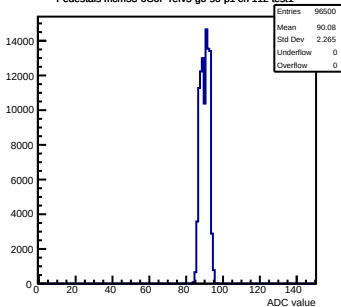
Pedestals mcm53-6C0F-refV5-g0-s0-p1 ch 112 test1
