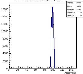
Pedestals mcm53-6C0F-refV5-g0-s0-p1 ch 111 test1
