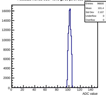
Pedestals mcm53-6C0F-refV5-g0-s0-p1 ch 108 test1
