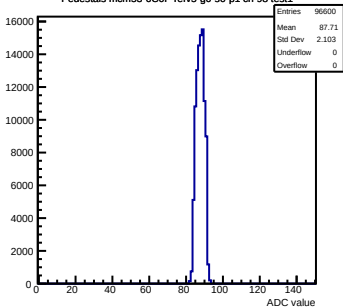
Pedestals mcm53-6C0F-refV5-g0-s0-p1 ch 98 test1
