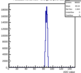
Pedestals mcm53-6C0F-refV5-g0-s0-p1 ch 118 test1
