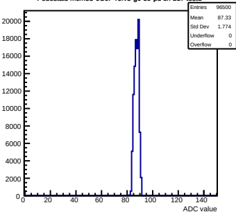
Pedestals mcm53-6C0F-refV5-g0-s0-p1 ch 117 test1
