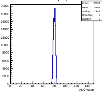
Pedestals mcm53-6C0F-refV5-g0-s0-p1 ch 125 test1
