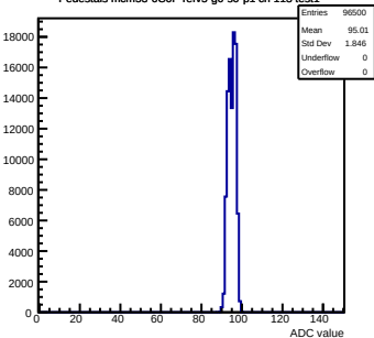
Pedestals mcm53-6C0F-refV5-g0-s0-p1 ch 113 test1
