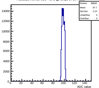
Pedestals mcm53-6C0F-refV5-g0-s0-p1 ch 104 test1
