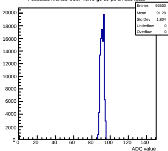
Pedestals mcm53-6C0F-refV5-g0-s0-p1 ch 123 test1
