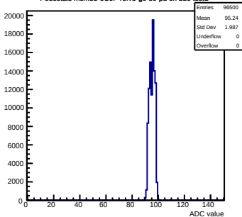
Pedestals mcm53-6C0F-refV5-g0-s0-p1 ch 116 test1
