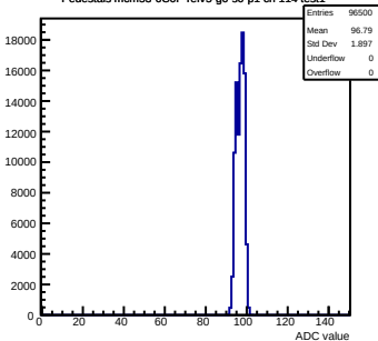
Pedestals mcm53-6C0F-refV5-g0-s0-p1 ch 114 test1
