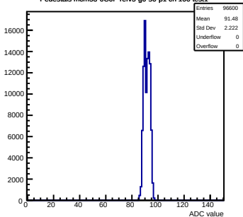
Pedestals mcm53-6C0F-refV5-g0-s0-p1 ch 100 test1
