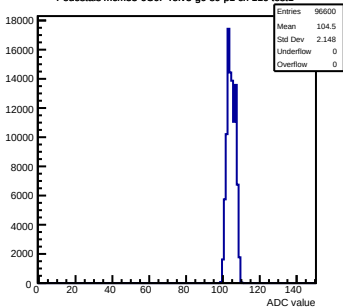
Pedestals mcm53-6C0F-refV5-g0-s0-p1 ch 110 test1
