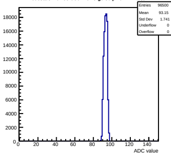
Pedestals mcm53-6C0F-refV5-g0-s0-p1 ch 124 test1
