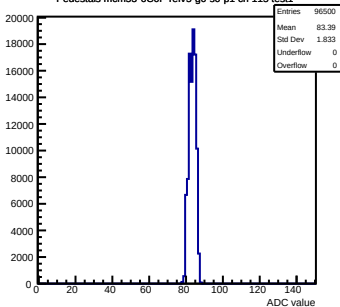
Pedestals mcm53-6C0F-refV5-g0-s0-p1 ch 115 test1
