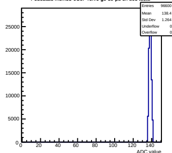
Pedestals mcm53-6C0F-refv6-g0-s0-p1 ch 105 test1
