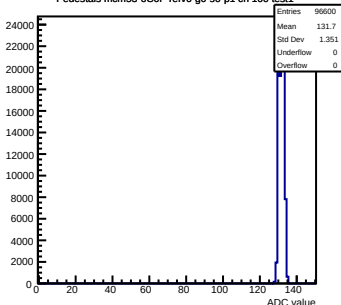
Pedestals mcm53-6C0F-refv6-g0-s0-p1 ch 100 test1
