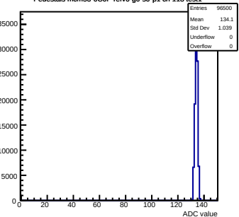
Pedestals mcm53-6C0F-refV6-g0-s0-p1 ch 113 test1
