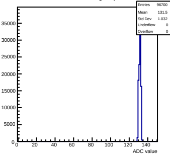
Pedestals mcm53-6C0F-relv6-g0-s0-p1 ch 92 test1
