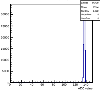
Pedestals mcm53-6C0F-relv6-g0-s0-p1 ch 93 test1
