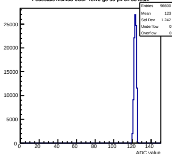
Pedestals mcm53-6C0F-refv6-g0-s0-p1 ch 38 test1
