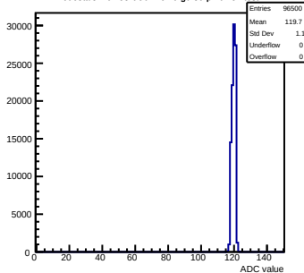
Pedestals mcm53-6C0F-relv6-g0-s0-p1 ch 54 test1
