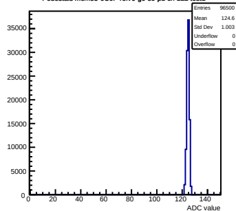
Pedestals mcm53-6C0F-refV6-g0-s0-p1 ch 122 test1
