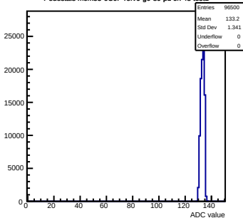
Pedestals mcm53-6C0F-relv6-g0-s0-p1 ch 48 test1
