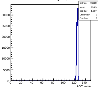
Pedestals mcm53-6C0F-relv6-g0-s0-p1 ch 56 test1
