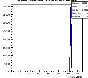
Pedestals mcm53-6C0F-refV6-g0-s0-p1 ch 118 test1
