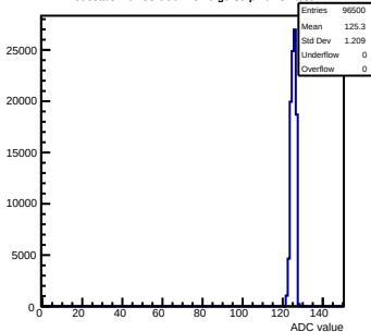
Pedestals mcm53-6C0F-relv6-g0-s0-p1 ch 52 test1
