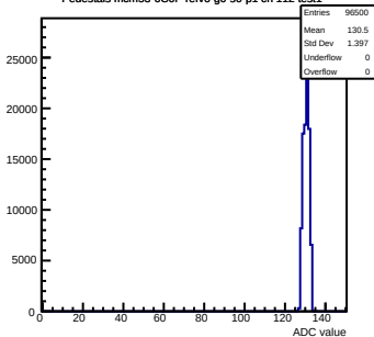
Pedestals mcm53-6C0F-refV6-g0-s0-p1 ch 112 test1
