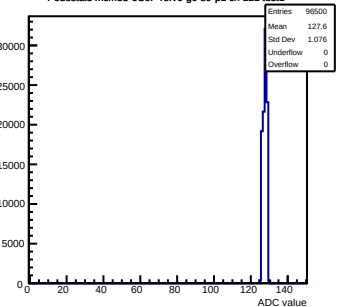
Pedestals mcm53-6C0F-refV6-g0-s0-p1 ch 121 test1
