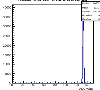
Pedestals mcm53-6C0F-refV6-g0-s0-p1 ch 119 test1
