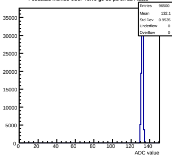
Pedestals mcm53-6C0F-refV6-g0-s0-p1 ch 124 test1
