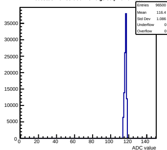
Pedestals mcm53-6C0F-relv6-g0-s0-p1 ch 61 test1
