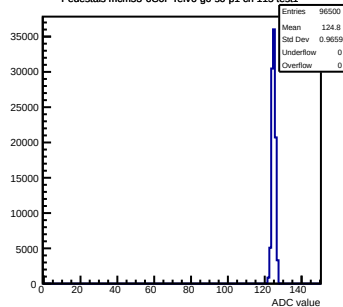
Pedestals mcm53-6C0F-refV6-g0-s0-p1 ch 115 test1
