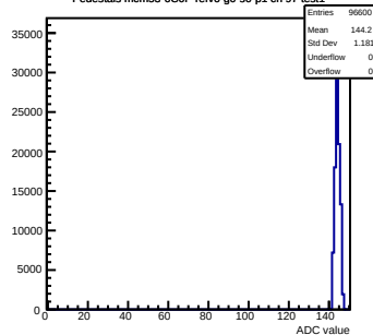
Pedestals mcm53-6C0F-refv6-g0-s0-p1 ch 97 test1
