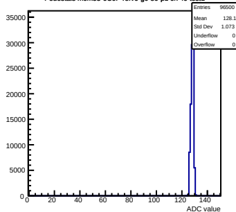
Pedestals mcm53-6C0F-relv6-g0-s0-p1 ch 49 test1
