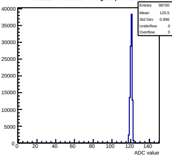
Pedestals mcm53-6C0F-relv6-g0-s0-p1 ch 88 test1
