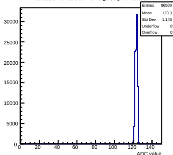
Pedestals mcm53-6C0F-relv6-g0-s0-p1 ch 58 test1
