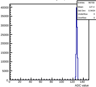
Pedestals mcm53-6C0F-relv6-g0-s0-p1 ch 95 test1
