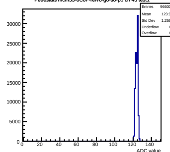
Pedestals mcm53-6C0F-refv6-g0-s0-p1 ch 43 test1
