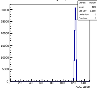
Pedestals mcm53-6C0F-relv6-g0-s0-p1 ch 84 test1
