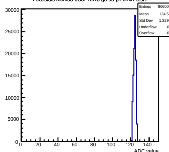
Pedestals mcm53-6C0F-refv6-g0-s0-p1 ch 41 test1
