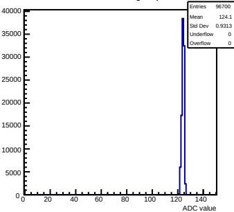
Pedestals mcm53-6C0F-relv6-g0-s0-p1 ch 94 test1
