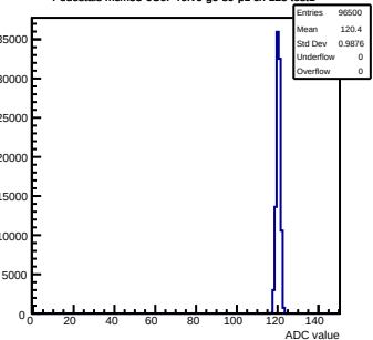
Pedestals mcm53-6C0F-refV6-g0-s0-p1 ch 125 test1
