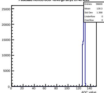
Pedestals mcm53-6C0F-refv6-g0-s0-p1 ch 40 test1
