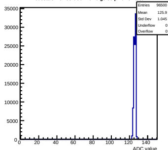
Pedestals mcm53-6C0F-relv6-g0-s0-p1 ch 57 test1
