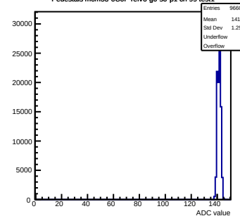
Pedestals mcm53-6C0F-refv6-g0-s0-p1 ch 99 test1
