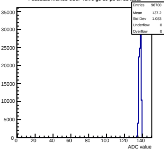
Pedestals mcm53-6C0F-relv6-g0-s0-p1 ch 83 test1
