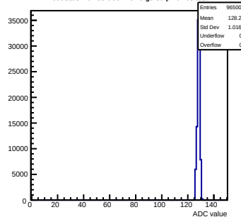
Pedestals mcm53-6C0F-relv6-g0-s0-p1 ch 63 test1
