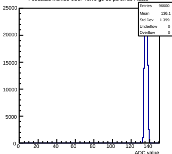
Pedestals mcm53-6C0F-refv6-g0-s0-p1 ch 104 test1
