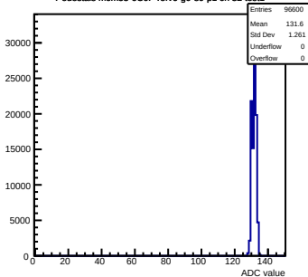
Pedestals mcm53-6C0F-refv6-g0-s0-p1 ch 32 test1
