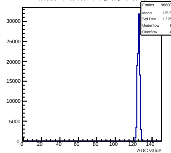
Pedestals mcm53-6C0F-refv6-g0-s0-p1 ch 35 test1
