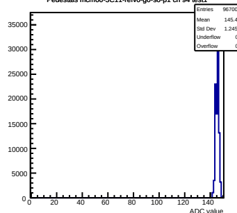
Pedestals mcm60-3C11-refV0-g0-s0-p1 ch 94 test1
