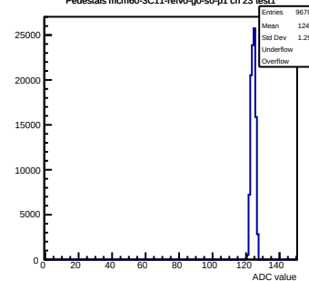
Pedestals mcm60-3C11-refV0-g0-s0-p1 ch 23 test1
