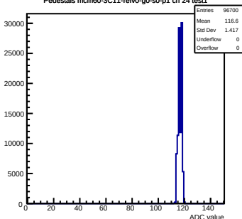
Pedestals mcm60-3C11-refV0-g0-s0-p1 ch 24 test1
