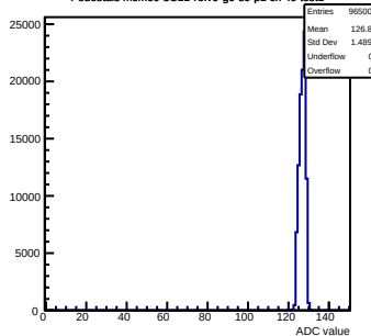
Pedestals mcm60-3C11-refV0-g0-s0-p1 ch 49 test1
