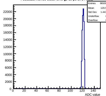
Pedestals mcm60-3C11-refV0-g0-s0-p1 ch 54 test1
