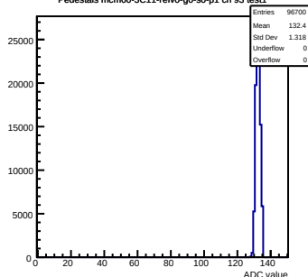
Pedestals mcm60-3C11-refV0-g0-s0-p1 ch 93 test1
