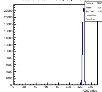
Pedestals mcm60-3C11-refV0-g0-s0-p1 ch 55 test1
