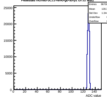
Pedestals mcm60-3C11-refV0-g0-s0-p1 ch 22 test1
