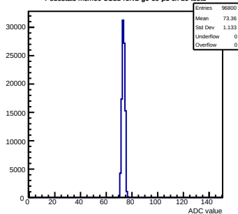
Pedestals mcm60-3C11-refv2-g0-s0-p1 ch 10 test1
