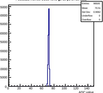
Pedestals mcm60-3C11-refv2-g0-s0-p1 ch 61 test1
