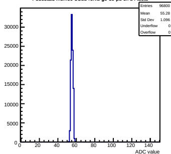
Pedestals mcm60-3C11-refv2-g0-s0-p1 ch 14 test1
