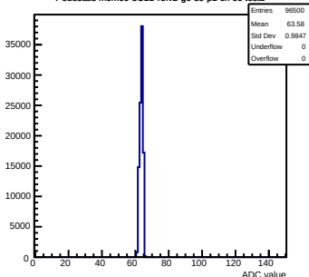
Pedestals mcm60-3C11-refv2-g0-s0-p1 ch 60 test1
