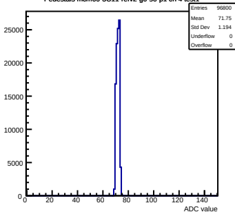
Pedestals mcm60-3C11-refv2-g0-s0-p1 ch 4 test1
