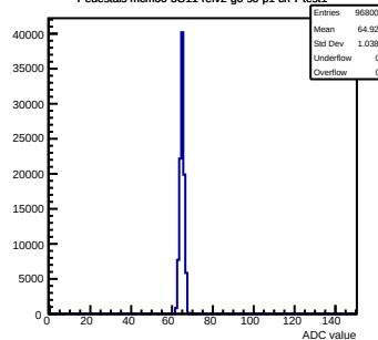
Pedestals mcm60-3C11-refv2-g0-s0-p1 ch 7 test1
