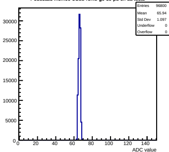
Pedestals mcm60-3C11-refv2-g0-s0-p1 ch 12 test1
