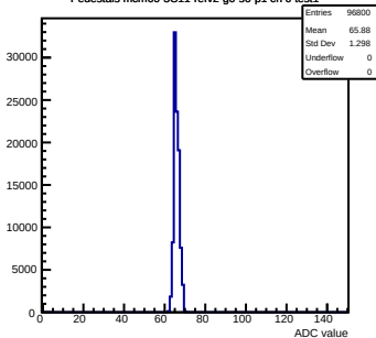
Pedestals mcm60-3C11-refv2-g0-s0-p1 ch 0 test1
