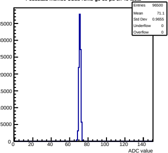
Pedestals mcm60-3C11-refv2-g0-s0-p1 ch 49 test1
