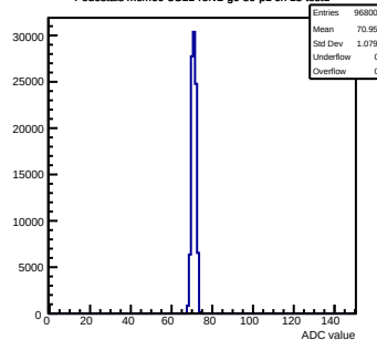
Pedestals mcm60-3C11-refv2-g0-s0-p1 ch 15 test1
