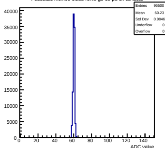
Pedestals mcm60-3C11-refv2-g0-s0-p1 ch 62 test1
