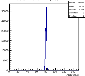
Pedestals mcm60-3C11-refv2-g0-s0-p1 ch 48 test1
