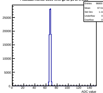
Pedestals mcm60-3C11-refv2-g0-s0-p1 ch 6 test1
