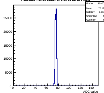
Pedestals mcm60-3C11-refv2-g0-s0-p1 ch 3 test1
