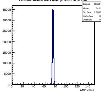
Pedestals mcm60-3C11-refv2-g0-s0-p1 ch 58 test1
