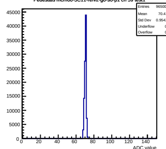
Pedestals mcm60-3C11-refv2-g0-s0-p1 ch 59 test1
