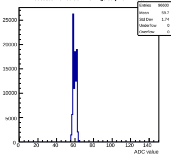
Pedestals mcm60-3C11-refV4-g0-s0-p1 ch 47 test1
