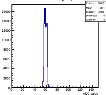
Pedestals mcm60-3C11-refV4-g0-s0-p1 ch 44 test1
