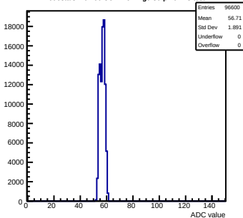
Pedestals mcm60-3C11-refV4-g0-s0-p1 ch 43 test1
