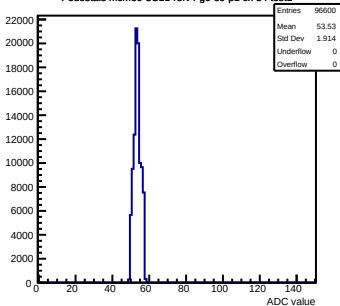
Pedestals mcm60-3C11-refV4-g0-s0-p1 ch 34 test1
