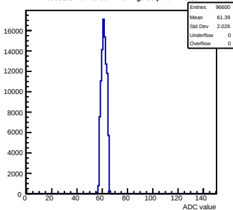
Pedestals mcm60-3C11-refV4-g0-s0-p1 ch 42 test1
