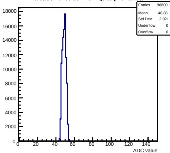
Pedestals mcm60-3C11-refV4-g0-s0-p1 ch 35 test1
