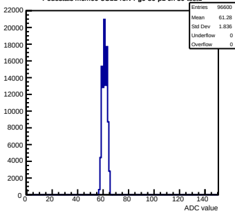
Pedestals mcm60-3C11-refV4-g0-s0-p1 ch 39 test1
