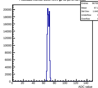
Pedestals mcm60-3C11-refv4-g0-s0-p1 ch 123 test1
