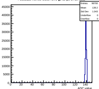
Pedestals mcm60-3C11-refV6-g0-s0-p1 ch 89 test1
