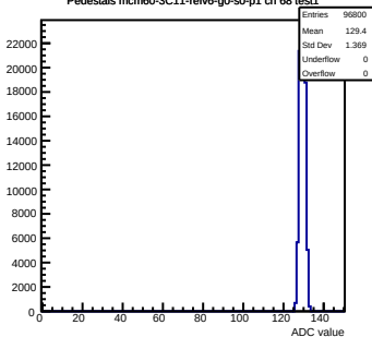
Pedestals mcm60-3C11-refV6-g0-s0-p1 ch 68 test1
