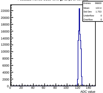
Pedestals mcm60-3C11-relv6-g0-s0-p1 ch 96 test1
