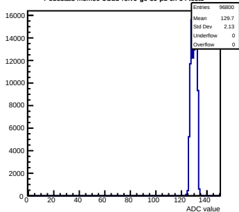
Pedestals mcm60-3C11-refV0-g0-s0-p1 ch 64 test1
