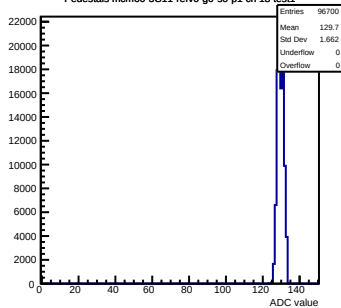
Pedestals mcm60-3C11-refV0-g0-s0-p1 ch 18 test1
