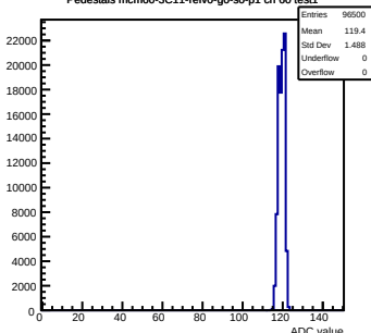
Pedestals mcm60-3C11-refV0-g0-s0-p1 ch 60 test1
