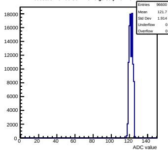
Pedestals mcm60-3C11-reV0-g0-s0-p1 ch 102 test1
