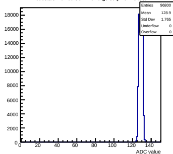
Pedestals mcm60-3C11-refV0-g0-s0-p1 ch 73 test1
