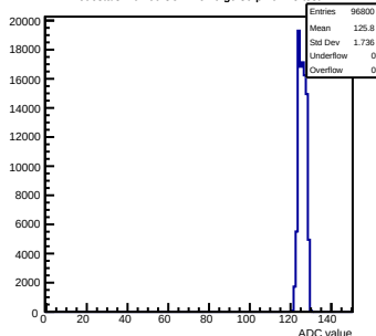
Pedestals mcm60-3C11-refV0-g0-s0-p1 ch 15 test1
