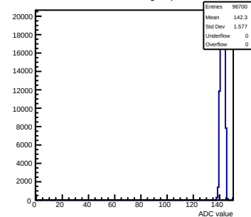
Pedestals mcm60-3C11-refV0-g0-s0-p1 ch 88 test1
