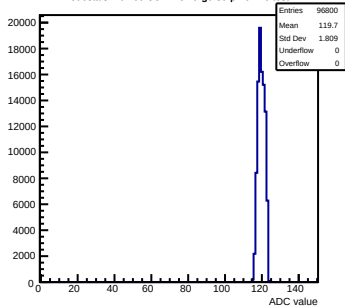
Pedestals mcm60-3C11-refV0-g0-s0-p1 ch 76 test1
