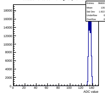
Pedestals mcm60-3C11-refV0-g0-s0-p1 ch 78 test1
