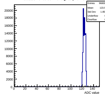
Pedestals mcm60-3C11-refV0-g0-s0-p1 ch 75 test1
