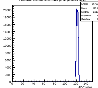
Pedestals mcm60-3C11-refV0-g0-s0-p1 ch 27 test1
