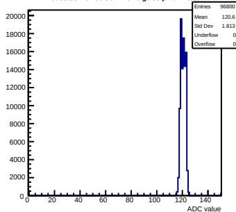
Pedestals mcm60-3C11-refV0-g0-s0-p1 ch 7 test1
