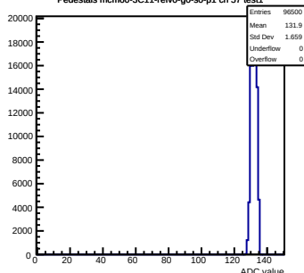
Pedestals mcm60-3C11-refV0-g0-s0-p1 ch 57 test1
