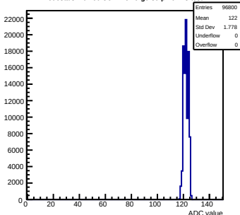
Pedestals mcm60-3C11-refV0-g0-s0-p1 ch 13 test1
