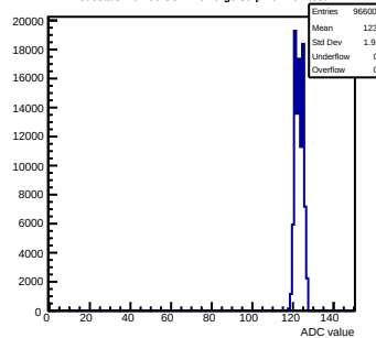
Pedestals mcm60-3C11-reV0-g0-s0-p1 ch 107 test1
