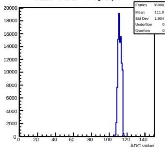
Pedestals mcm60-3C11-refV0-g0-s0-p1 ch 14 test1
