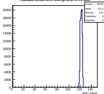
Pedestals mcm60-3C11-refV0-g0-s0-p1 ch 29 test1
