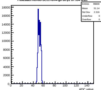
Pedestals mcm60-3C11-refV4-g0-s0-p1 ch 104 test1
