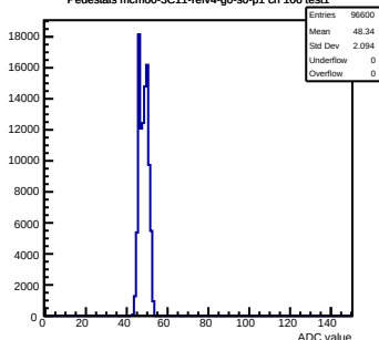
Pedestals mcm60-3C11-refV4-g0-s0-p1 ch 106 test1
