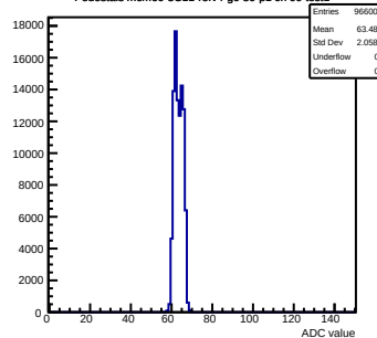
Pedestals mcm60-3C11-refV4-g0-s0-p1 ch 99 test1
