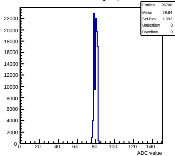
Pedestals mcm60-3C11-refv4-g0-s0-p1 ch 94 test1
