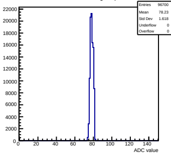
Pedestals mcm60-3C11-refv4-g0-s0-p1 ch 84 test1
