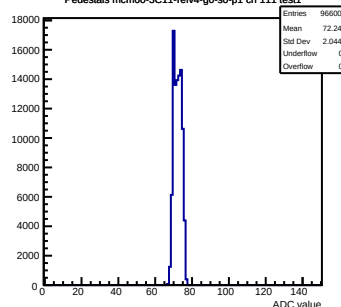
Pedestals mcm60-3C11-refV4-g0-s0-p1 ch 111 test1
