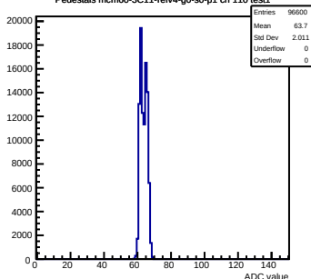
Pedestals mcm60-3C11-refV4-g0-s0-p1 ch 110 test1
