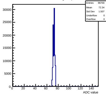
Pedestals mcm60-3C11-refv4-g0-s0-p1 ch 85 test1
