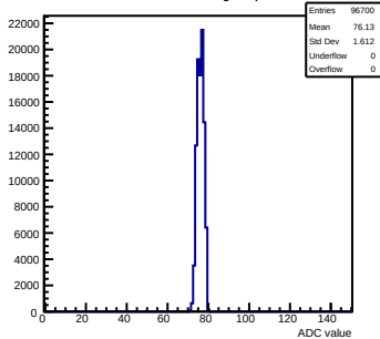
Pedestals mcm60-3C11-refv4-g0-s0-p1 ch 90 test1
