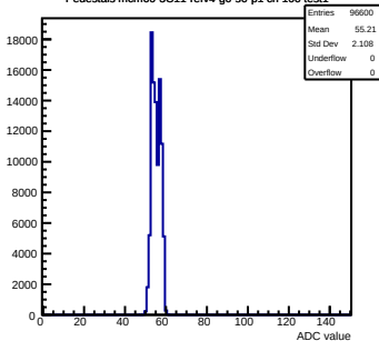
Pedestals mcm60-3C11-refV4-g0-s0-p1 ch 100 test1
