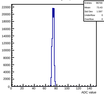
Pedestals mcm60-3C11-refv4-g0-s0-p1 ch 92 test1
