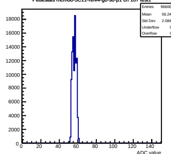
Pedestals mcm60-3C11-refV4-g0-s0-p1 ch 107 test1
