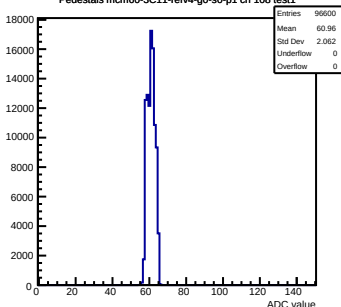
Pedestals mcm60-3C11-refV4-g0-s0-p1 ch 108 test1
