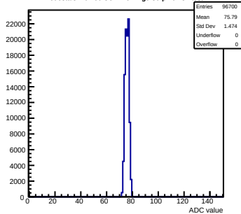
Pedestals mcm60-3C11-refv4-g0-s0-p1 ch 87 test1
