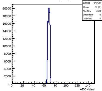
Pedestals mcm60-3C11-refv4-g0-s0-p1 ch 93 test1
