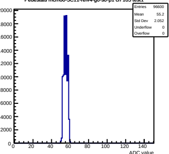
Pedestals mcm60-3C11-refV4-g0-s0-p1 ch 105 test1
