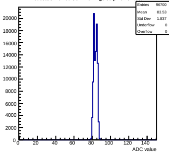
Pedestals mcm60-3C11-refv4-g0-s0-p1 ch 80 test1
