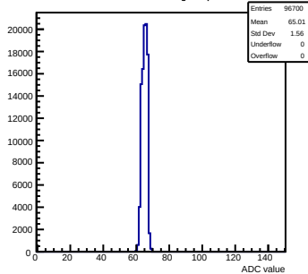
Pedestals mcm60-3C11-refv4-g0-s0-p1 ch 95 test1
