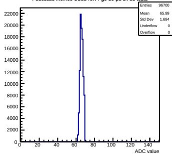
Pedestals mcm60-3C11-refv4-g0-s0-p1 ch 83 test1
