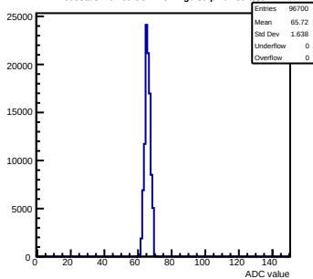
Pedestals mcm60-3C11-refv4-g0-s0-p1 ch 86 test1
