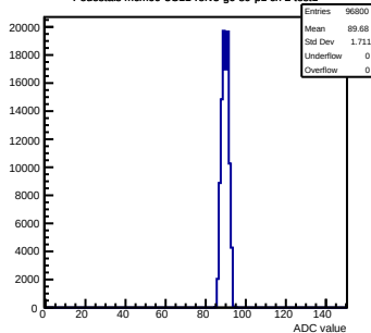
Pedestals mcm60-3C11-refV5-g0-s0-p1 ch 2 test1
