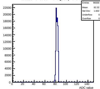
Pedestals mcm60-3C11-refV5-g0-s0-p1 ch 51 test1
