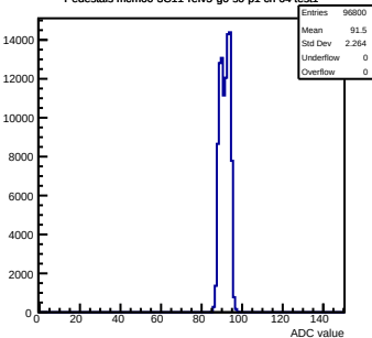
Pedestals mcm60-3C11-refV5-g0-s0-p1 ch 64 test1
