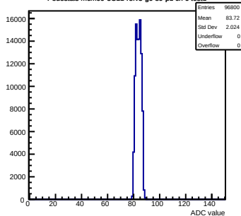
Pedestals mcm60-3C11-refV5-g0-s0-p1 ch 6 test1
