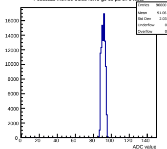
Pedestals mcm60-3C11-refV5-g0-s0-p1 ch 3 test1
