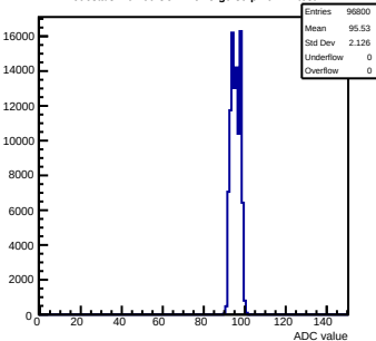
Pedestals mcm60-3C11-refV5-g0-s0-p1 ch 72 test1
