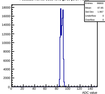
Pedestals mcm60-3C11-refV5-g0-s0-p1 ch 4 test1
