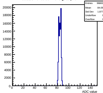
Pedestals mcm60-3C11-refV5-g0-s0-p1 ch 77 test1
