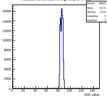
Pedestals mcm60-3C11-refV5-g0-s0-p1 ch 5 test1
