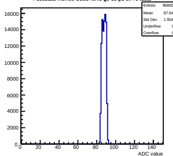
Pedestals mcm60-3C11-refV5-g0-s0-p1 ch 70 test1
