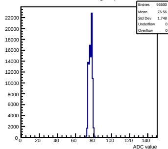
Pedestals mcm60-3C11-refV5-g0-s0-p1 ch 63 test1
