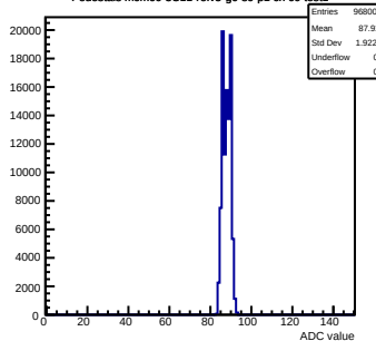
Pedestals mcm60-3C11-refV5-g0-s0-p1 ch 69 test1
