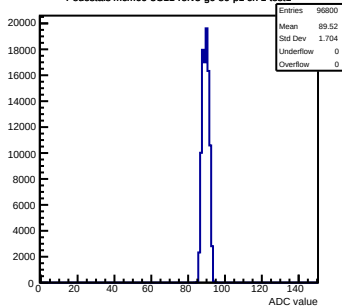
Pedestals mcm60-3C11-refV5-g0-s0-p1 ch 1 test1
