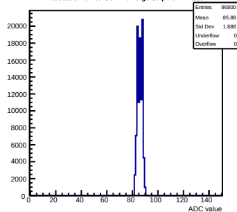
Pedestals mcm60-3C11-refV5-g0-s0-p1 ch 11 test1
