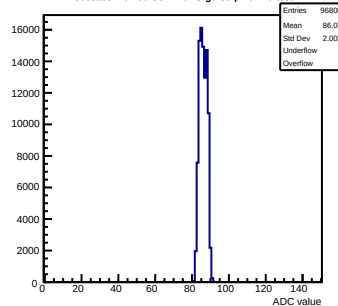
Pedestals mcm60-3C11-refV5-g0-s0-p1 ch 79 test1
