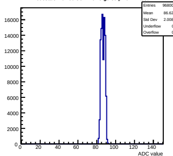
Pedestals mcm60-3C11-refV5-g0-s0-p1 ch 74 test1
