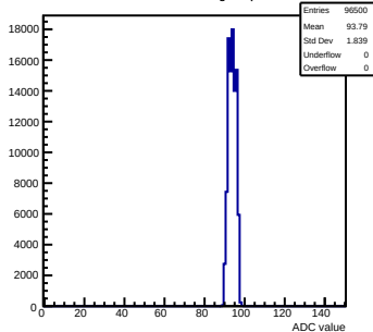
Pedestals mcm60-3C11-refV5-g0-s0-p1 ch 57 test1
