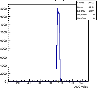
Pedestals mcm60-3C11-reV5-g0-s0-p1 ch 98 test1
