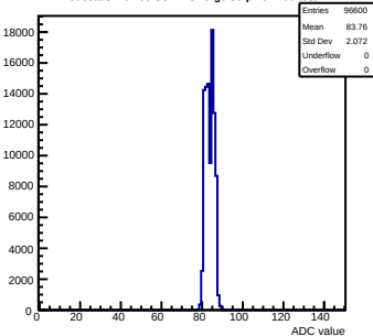
Pedestals mcm60-3C11-reV5-g0-s0-p1 ch 96 test1
