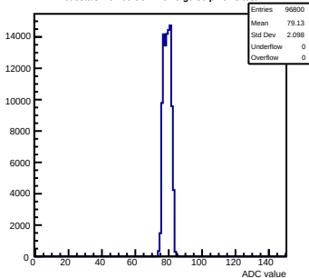
Pedestals mcm60-3C11-refV5-g0-s0-p1 ch 8 test1
