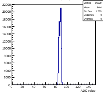
Pedestals mcm60-3C11-refV5-g0-s0-p1 ch 61 test1
