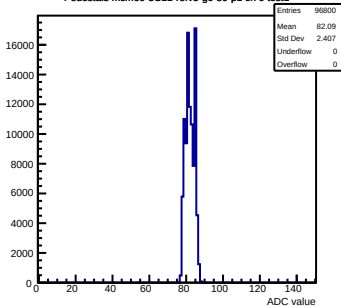
Pedestals mcm60-3C11-refV5-g0-s0-p1 ch 0 test1
