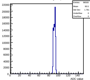
Pedestals mcm60-3C11-refV5-g0-s0-p1 ch 58 test1
