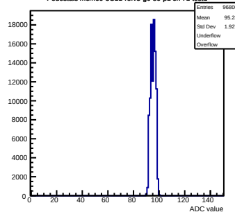
Pedestals mcm60-3C11-refV5-g0-s0-p1 ch 71 test1
