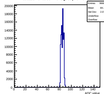
Pedestals mcm60-3C11-reV5-g0-s0-p1 ch 103 test1
