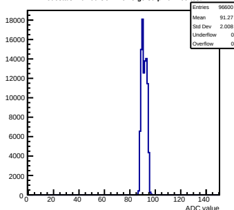
Pedestals mcm60-3C11-reV5-g0-s0-p1 ch 109 test1
