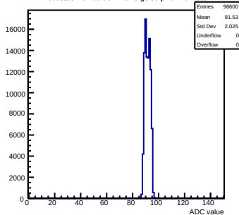
Pedestals mcm60-3C11-reV5-g0-s0-p1 ch 97 test1
