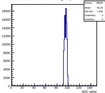
Pedestals mcm60-3C11-refV5-g0-s0-p1 ch 48 test1
