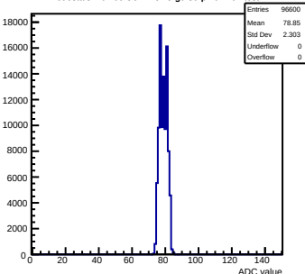
Pedestals mcm60-3C11-reV5-g0-s0-p1 ch 100 test1
