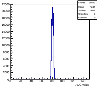
Pedestals mcm60-3C11-refV5-g0-s0-p1 ch 60 test1
