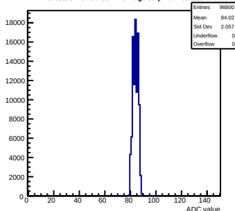
Pedestals mcm60-3C11-reV5-g0-s0-p1 ch 101 test1
