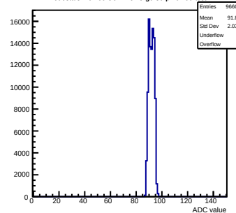
Pedestals mcm60-3C11-reV5-g0-s0-p1 ch 99 test1
