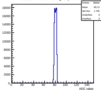
Pedestals mcm60-3C11-refV5-g0-s0-p1 ch 54 test1
