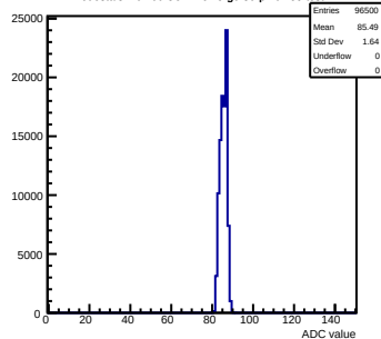
Pedestals mcm60-3C11-refV5-g0-s0-p1 ch 55 test1
