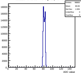
Pedestals mcm60-3C11-refV5-g0-s0-p1 ch 76 test1
