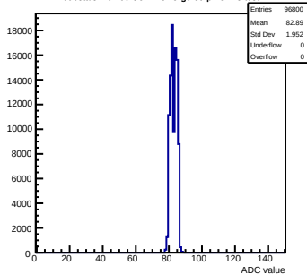
Pedestals mcm60-3C11-refV5-g0-s0-p1 ch 13 test1
