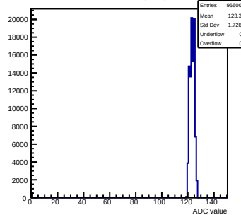
Pedestals mcm60-3C11-relv6-g0-s0-p1 ch 102 test1
