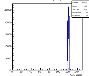
Pedestals mcm60-3C11-refv6-g0-s0-p1 ch 28 test1
