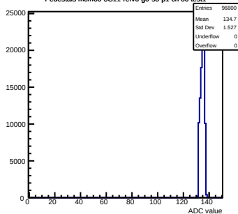
Pedestals mcm60-3C11-refv6-g0-s0-p1 ch 66 test1
