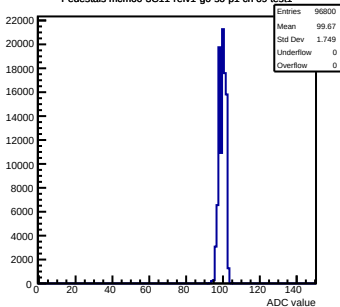
Pedestals mcm60-3C11-refv1-g0-s0-p1 ch 69 test1
