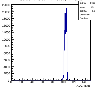
Pedestals mcm60-3C11-reV1-g0-s0-p1 ch 103 test1
