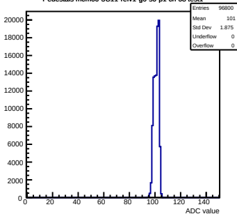
Pedestals mcm60-3C11-refv1-g0-s0-p1 ch 68 test1
