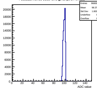
Pedestals mcm60-3C11-refv1-g0-s0-p1 ch 79 test1
