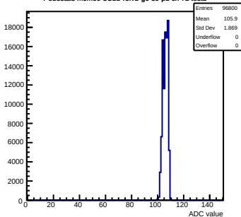
Pedestals mcm60-3C11-refv1-g0-s0-p1 ch 72 test1
