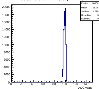
Pedestals mcm60-3C11-refv1-g0-s0-p1 ch 74 test1
