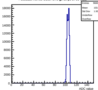
Pedestals mcm60-3C11-reV1-g0-s0-p1 ch 99 test1
