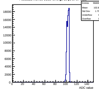
Pedestals mcm60-3C11-refv1-g0-s0-p1 ch 67 test1
