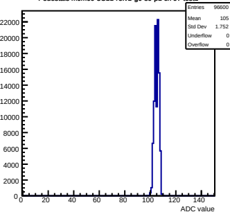
Pedestals mcm60-3C11-reV1-g0-s0-p1 ch 97 test1
