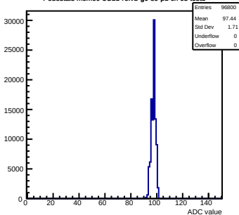
Pedestals mcm60-3C11-refv1-g0-s0-p1 ch 65 test1
