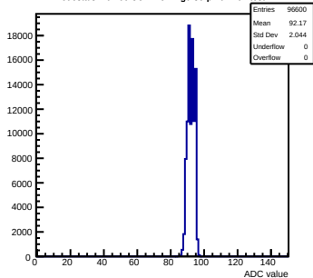
Pedestals mcm60-3C11-reV1-g0-s0-p1 ch 100 test1
