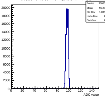
Pedestals mcm60-3C11-reV1-g0-s0-p1 ch 102 test1
