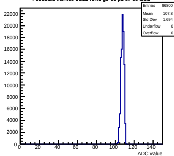
Pedestals mcm60-3C11-refv1-g0-s0-p1 ch 66 test1
