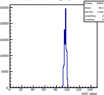
Pedestals mcm60-3C11-reV1-g0-s0-p1 ch 105 test1
