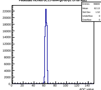
Pedestals mcm60-3C11-refv4-g0-s0-p1 ch 69 test1
