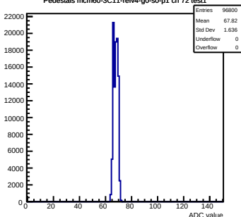
Pedestals mcm60-3C11-refv4-g0-s0-p1 ch 72 test1
