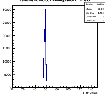
Pedestals mcm60-3C11-refv4-g0-s0-p1 ch 77 test1
