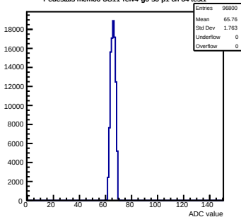
Pedestals mcm60-3C11-refv4-g0-s0-p1 ch 64 test1
