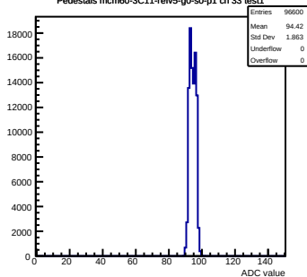
Pedestals mcm60-3C11-refV5-g0-s0-p1 ch 33 test1
