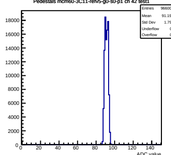
Pedestals mcm60-3C11-refV5-g0-s0-p1 ch 42 test1
