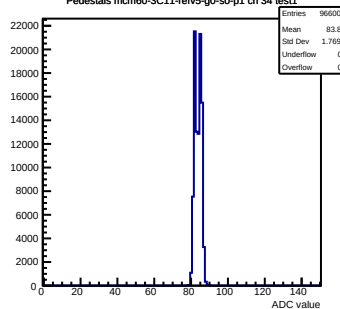
Pedestals mcm60-3C11-refV5-g0-s0-p1 ch 34 test1
