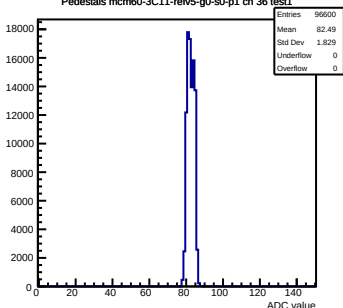
Pedestals mcm60-3C11-refV5-g0-s0-p1 ch 36 test1
