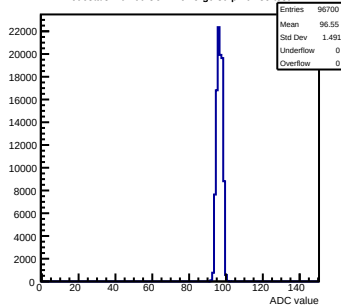
Pedestals mcm60-3C11-refV5-g0-s0-p1 ch 81 test1
