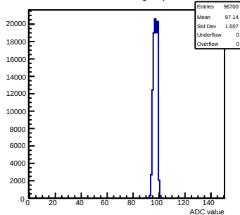
Pedestals mcm60-3C11-refV5-g0-s0-p1 ch 93 test1
