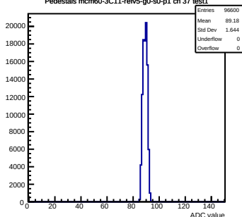
Pedestals mcm60-3C11-refV5-g0-s0-p1 ch 37 test1
