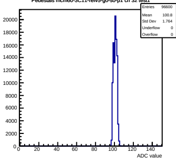
Pedestals mcm60-3C11-refV5-g0-s0-p1 ch 32 test1
