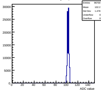
Pedestals mcm60-3C11-refV5-g0-s0-p1 ch 85 test1
