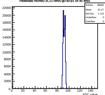
Pedestals mcm60-3C11-refV5-g0-s0-p1 ch 45 test1
