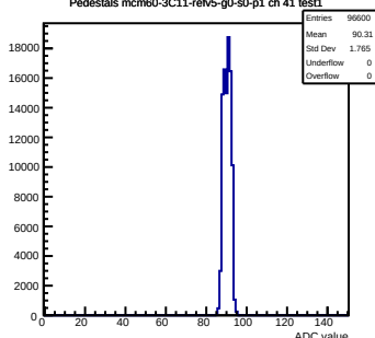
Pedestals mcm60-3C11-refV5-g0-s0-p1 ch 41 test1
