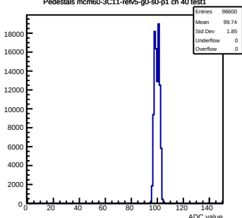
Pedestals mcm60-3C11-refV5-g0-s0-p1 ch 40 test1
