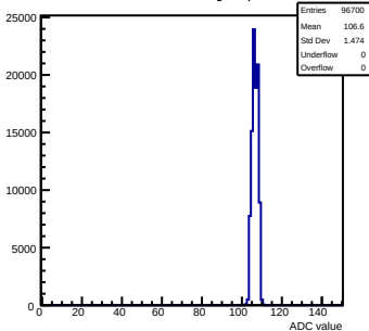
Pedestals mcm60-3C11-refV5-g0-s0-p1 ch 87 test1
