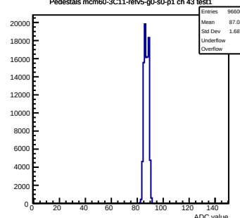
Pedestals mcm60-3C11-refV5-g0-s0-p1 ch 43 test1
