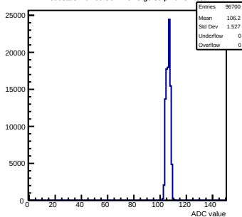
Pedestals mcm60-3C11-refV5-g0-s0-p1 ch 82 test1
