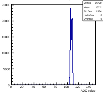
Pedestals mcm60-3C11-refV5-g0-s0-p1 ch 84 test1
