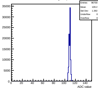
Pedestals mcm60-3C11-refV5-g0-s0-p1 ch 94 test1
