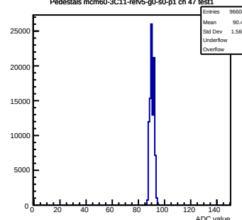
Pedestals mcm60-3C11-refV5-g0-s0-p1 ch 47 test1
