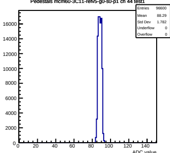
Pedestals mcm60-3C11-refV5-g0-s0-p1 ch 44 test1
