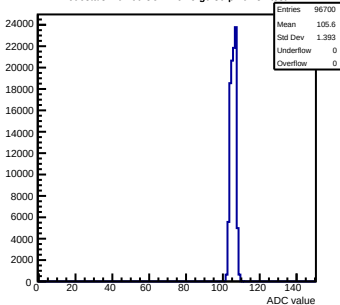
Pedestals mcm60-3C11-refV5-g0-s0-p1 ch 83 test1
