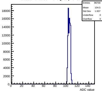
Pedestals mcm60-3C11-refV5-g0-s0-p1 ch 80 test1
