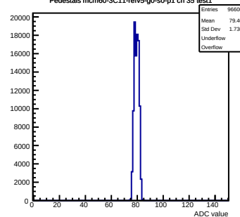
Pedestals mcm60-3C11-refV5-g0-s0-p1 ch 35 test1
