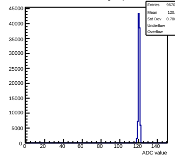
Pedestals mcm60-3C11-refV1-g0-s0-p1 ch 91 test1
