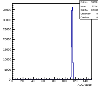
Pedestals mcm60-3C11-refV1-g0-s0-p1 ch 85 test1
