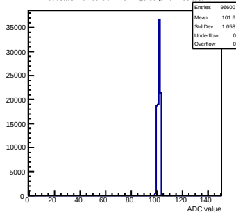
Pedestals mcm60-3C11-reV1-g0-s0-p1 ch 105 test1
