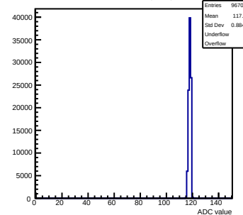
Pedestals mcm60-3C11-refV1-g0-s0-p1 ch 87 test1
