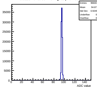
Pedestals mcm60-3C11-reV1-g0-s0-p1 ch 106 test1
