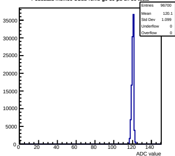
Pedestals mcm60-3C11-refV1-g0-s0-p1 ch 80 test1
