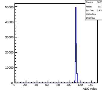
Pedestals mcm60-3C11-refV1-g0-s0-p1 ch 95 test1
