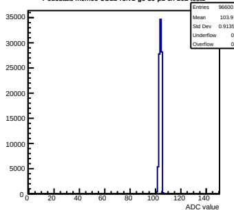
Pedestals mcm60-3C11-reV1-g0-s0-p1 ch 102 test1
