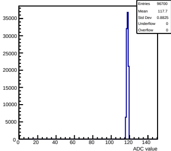
Pedestals mcm60-3C11-refV1-g0-s0-p1 ch 92 test1
