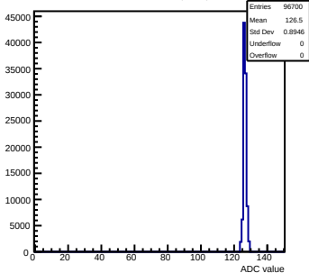
Pedestals mcm60-3C11-refV1-g0-s0-p1 ch 84 test1
