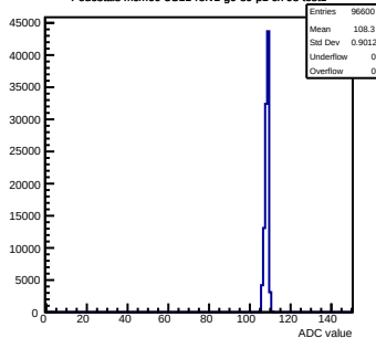
Pedestals mcm60-3C11-reV1-g0-s0-p1 ch 98 test1
