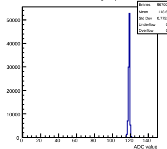
Pedestals mcm60-3C11-refV1-g0-s0-p1 ch 90 test1
