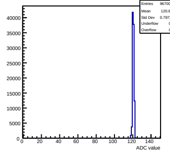
Pedestals mcm60-3C11-refV1-g0-s0-p1 ch 94 test1
