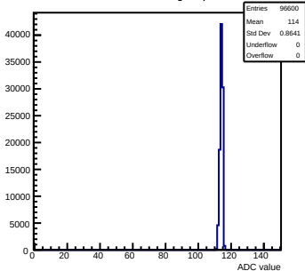
Pedestals mcm60-3C11-refv1-g0-s0-p1 ch 40 test1
