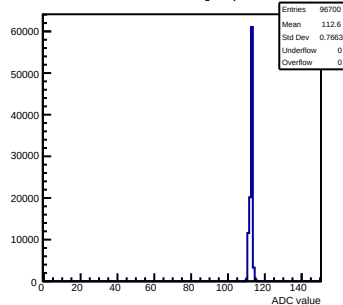
Pedestals mcm60-3C11-refV1-g0-s0-p1 ch 89 test1
