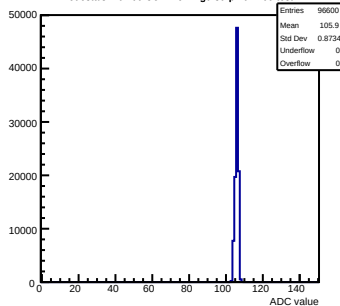
Pedestals mcm60-3C11-reV1-g0-s0-p1 ch 109 test1
