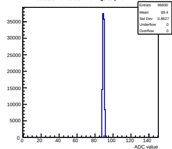
Pedestals mcm60-3C11-reV2-g0-s0-p1 ch 111 test1
