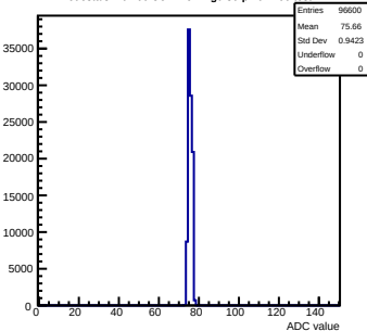
Pedestals mcm60-3C11-reV2-g0-s0-p1 ch 100 test1
