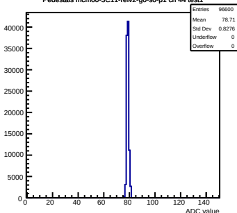
Pedestals mcm60-3C11-ref2-g0-s0-p1 ch 44 test1
