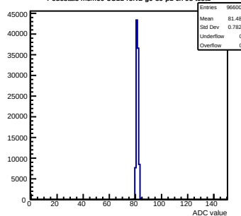
Pedestals mcm60-3C11-reV2-g0-s0-p1 ch 98 test1
