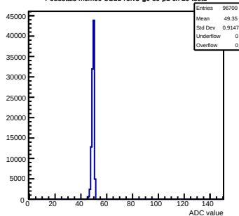
Pedestals mcm60-3C11-refv3-g0-s0-p1 ch 29 test1
