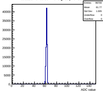
Pedestals mcm60-3C11-refv3-g0-s0-p1 ch 85 test1
