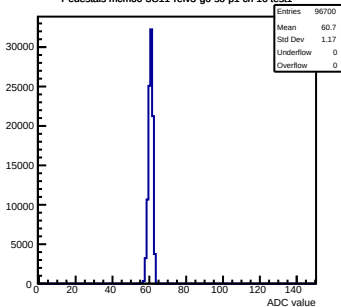
Pedestals mcm60-3C11-refv3-g0-s0-p1 ch 16 test1
