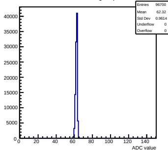
Pedestals mcm60-3C11-refv3-g0-s0-p1 ch 93 test1
