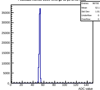
Pedestals mcm60-3C11-refv3-g0-s0-p1 ch 22 test1
