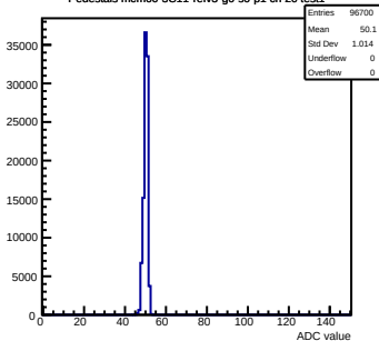
Pedestals mcm60-3C11-refv3-g0-s0-p1 ch 20 test1
