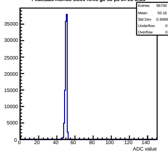
Pedestals mcm60-3C11-refv3-g0-s0-p1 ch 23 test1
