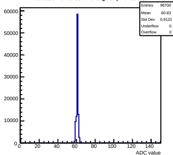
Pedestals mcm60-3C11-refv3-g0-s0-p1 ch 89 test1
