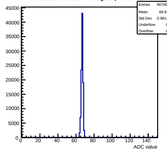
Pedestals mcm60-3C11-refv3-g0-s0-p1 ch 87 test1
