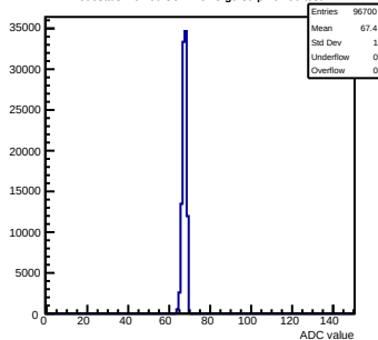
Pedestals mcm60-3C11-refv3-g0-s0-p1 ch 90 test1
