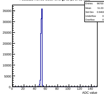
Pedestals mcm60-3C11-refv3-g0-s0-p1 ch 25 test1
