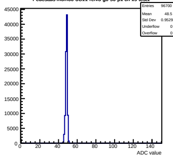
Pedestals mcm60-3C11-refv3-g0-s0-p1 ch 19 test1
