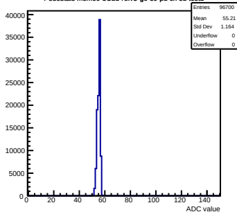
Pedestals mcm60-3C11-refv3-g0-s0-p1 ch 81 test1
