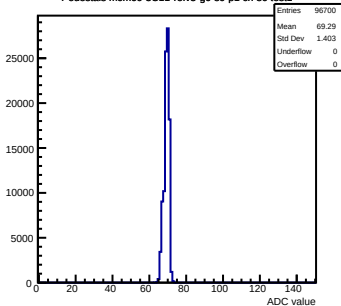
Pedestals mcm60-3C11-refv3-g0-s0-p1 ch 80 test1
