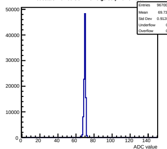
Pedestals mcm60-3C11-refv3-g0-s0-p1 ch 91 test1
