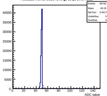
Pedestals mcm60-3C11-refv3-g0-s0-p1 ch 27 test1
