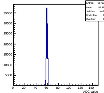
Pedestals mcm60-3C11-refv3-g0-s0-p1 ch 95 test1
