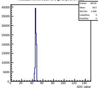
Pedestals mcm60-3C11-refv3-g0-s0-p1 ch 24 test1
