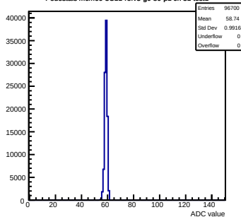
Pedestals mcm60-3C11-refv3-g0-s0-p1 ch 31 test1
