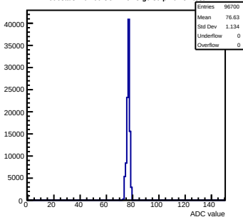
Pedestals mcm60-3C11-refv3-g0-s0-p1 ch 84 test1
