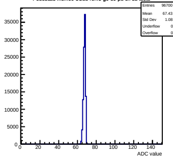
Pedestals mcm60-3C11-refv3-g0-s0-p1 ch 82 test1
