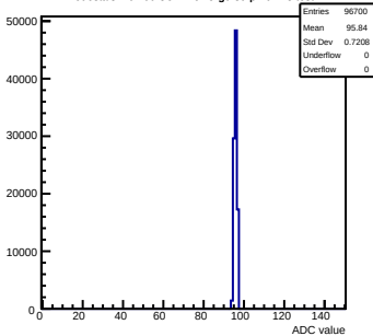
Pedestals mcm60-3C11-refV5-g0-s0-p1 ch 28 test1
