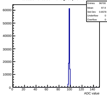
Pedestals mcm60-3C11-refV5-g0-s0-p1 ch 29 test1
