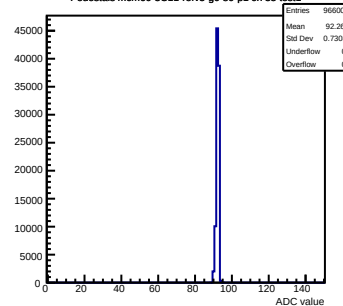
Pedestals mcm60-3C11-refV5-g0-s0-p1 ch 35 test1
