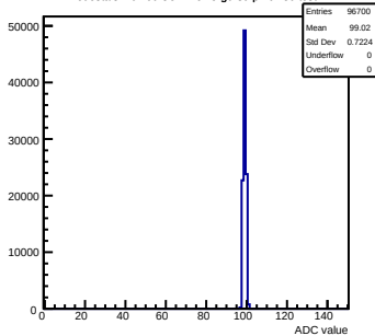
Pedestals mcm60-3C11-refV5-g0-s0-p1 ch 30 test1
