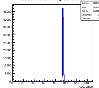
Pedestals mcm60-3C11-refV5-g0-s0-p1 ch 38 test1
