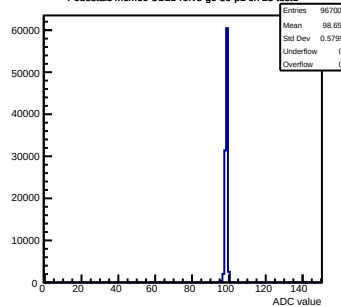
Pedestals mcm60-3C11-refV5-g0-s0-p1 ch 23 test1
