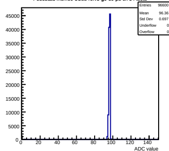
Pedestals mcm60-3C11-refV5-g0-s0-p1 ch 34 test1
