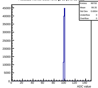
Pedestals mcm60-3C11-refV5-g0-s0-p1 ch 25 test1
