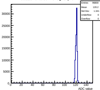
Pedestals mcm60-3C11-refv6-g0-s0-p1 ch 4 test1
