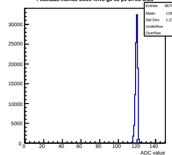
Pedestals mcm60-3C11-refV6-g0-s0-p1 ch 23 test1
