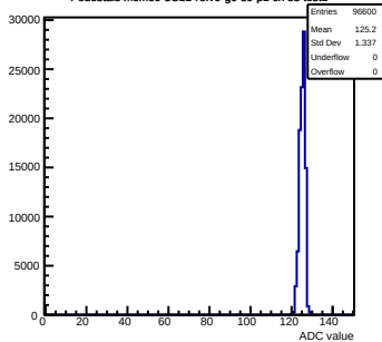
Pedestals mcm60-3C11-refV6-g0-s0-p1 ch 33 test1
