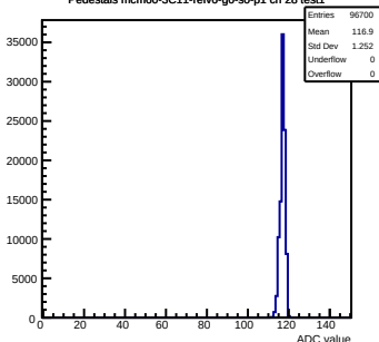
Pedestals mcm60-3C11-refV6-g0-s0-p1 ch 28 test1
