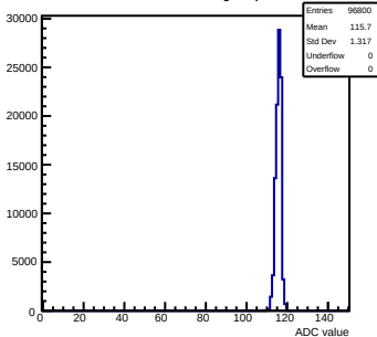
Pedestals mcm60-3C11-refv6-g0-s0-p1 ch 8 test1
