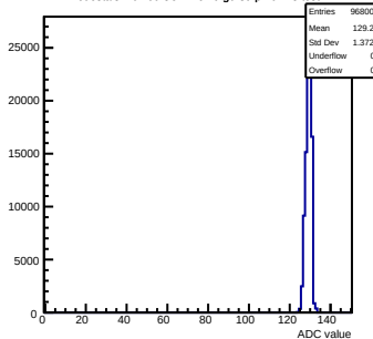
Pedestals mcm60-3C11-refv6-g0-s0-p1 ch 78 test1
