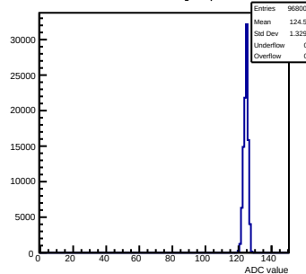
Pedestals mcm60-3C11-refv6-g0-s0-p1 ch 10 test1
