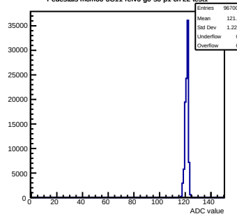
Pedestals mcm60-3C11-refV6-g0-s0-p1 ch 22 test1
