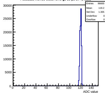
Pedestals mcm60-3C11-refV6-g0-s0-p1 ch 43 test1
