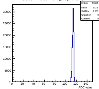
Pedestals mcm60-3C11-refV6-g0-s0-p1 ch 35 test1
