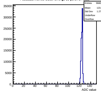
Pedestals mcm60-3C11-refv6-g0-s0-p1 ch 67 test1
