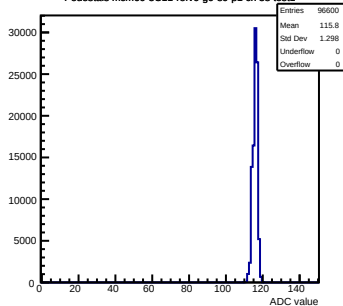
Pedestals mcm60-3C11-refV6-g0-s0-p1 ch 38 test1
