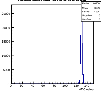
Pedestals mcm60-3C11-refV6-g0-s0-p1 ch 16 test1
