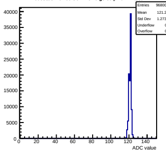
Pedestals mcm60-3C11-refv6-g0-s0-p1 ch 74 test1
