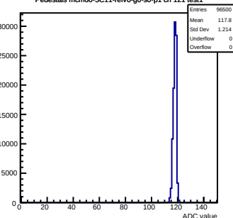
Pedestals mcm60-3C11-relv6-g0-s0-p1 ch 121 test1
