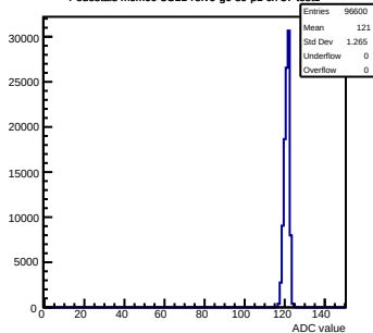
Pedestals mcm60-3C11-refV6-g0-s0-p1 ch 37 test1
