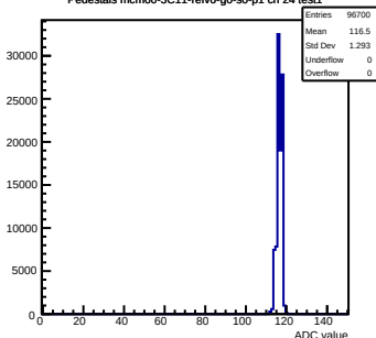
Pedestals mcm60-3C11-refV6-g0-s0-p1 ch 24 test1
