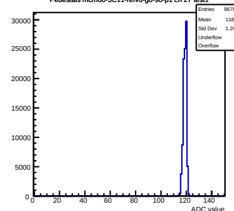
Pedestals mcm60-3C11-refV6-g0-s0-p1 ch 27 test1
