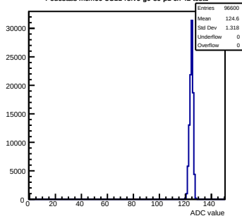
Pedestals mcm60-3C11-refV6-g0-s0-p1 ch 42 test1
