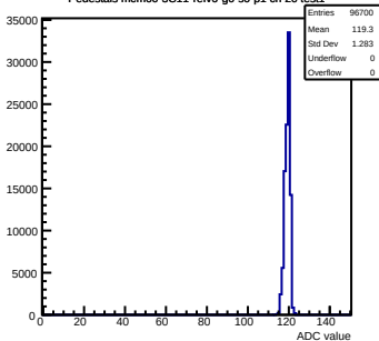
Pedestals mcm60-3C11-refV6-g0-s0-p1 ch 20 test1
