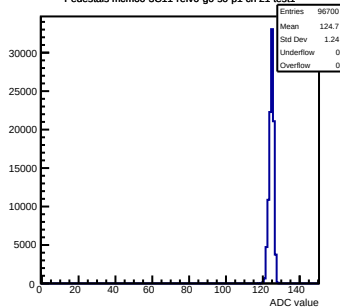
Pedestals mcm60-3C11-refV6-g0-s0-p1 ch 21 test1
