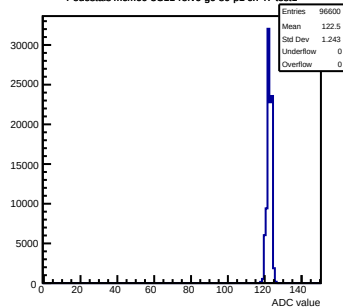
Pedestals mcm60-3C11-refV6-g0-s0-p1 ch 47 test1
