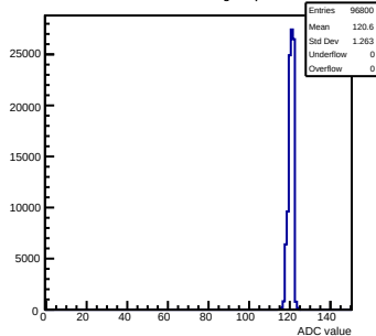
Pedestals mcm60-3C11-refv6-g0-s0-p1 ch 13 test1
