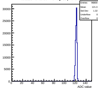
Pedestals mcm60-3C11-refv6-g0-s0-p1 ch 5 test1
