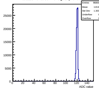
Pedestals mcm60-3C11-refv6-g0-s0-p1 ch 6 test1
