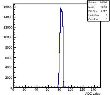
Pedestals mcm61-3214-rfv1-g0-s0-p1 ch 51 test1
