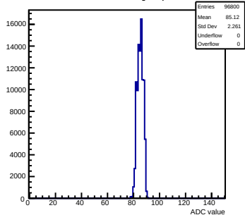
Pedestals mcm61-3214-refv1-g0-s0-p1 ch 73 test1
