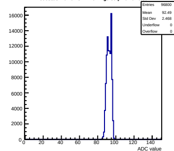
Pedestals mcm61-3214-refv1-g0-s0-p1 ch 64 test1
