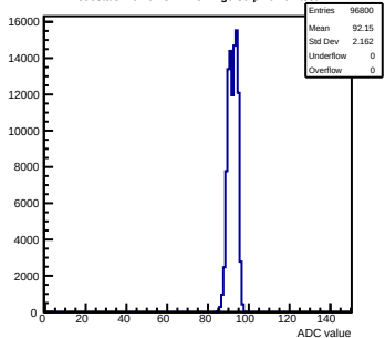
Pedestals mcm61-3214-refv1-g0-s0-p1 ch 67 test1
