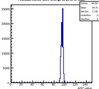
Pedestals mcm61-3214-refv1-g0-s0-p1 ch 87 test1
