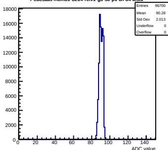
Pedestals mcm61-3214-refv1-g0-s0-p1 ch 84 test1
