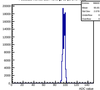
Pedestals mcm61-3214-refv1-g0-s0-p1 ch 97 test1
