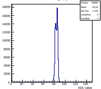
Pedestals mcm61-3214-refv1-g0-s0-p1 ch 71 test1
