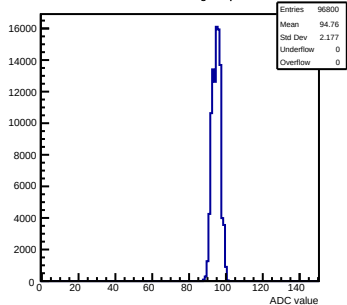
Pedestals mcm61-3214-refv1-g0-s0-p1 ch 78 test1
