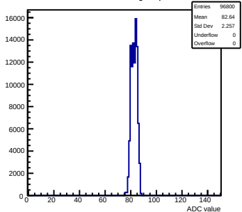
Pedestals mcm61-3214-refv1-g0-s0-p1 ch 75 test1
