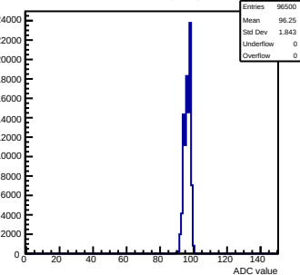
Pedestals mcm61-3214-rfv1-g0-s0-p1 ch 50 test1
