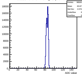
Pedestals mcm61-3214-rfv1-g0-s0-p1 ch 49 test1
