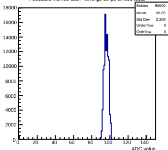
Pedestals mcm61-3214-refv1-g0-s0-p1 ch 108 test1
