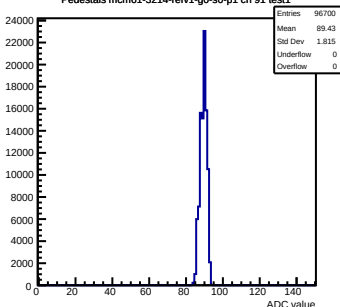
Pedestals mcm61-3214-refv1-g0-s0-p1 ch 91 test1
