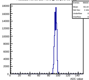
Pedestals mcm61-3214-refv1-g0-s0-p1 ch 98 test1
