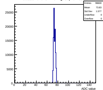
Pedestals mcm61-3214-refv2-g0-s0-p1 ch 108 test1
