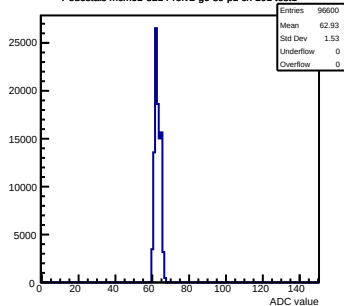
Pedestals mcm61-3214-refv2-g0-s0-p1 ch 101 test1
