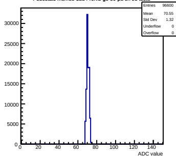
Pedestals mcm61-3214-refv2-g0-s0-p1 ch 98 test1
