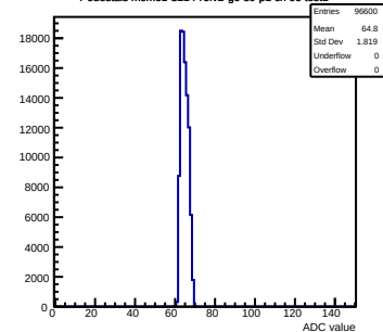
Pedestals mcm61-3214-refv2-g0-s0-p1 ch 96 test1
