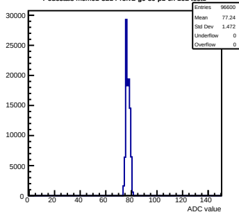
Pedestals mcm61-3214-refv2-g0-s0-p1 ch 102 test1
