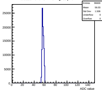
Pedestals mcm61-3214-refv2-g0-s0-p1 ch 111 test1
