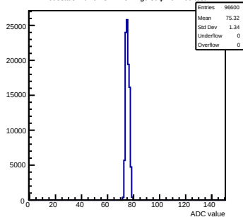
Pedestals mcm61-3214-refv2-g0-s0-p1 ch 109 test1
