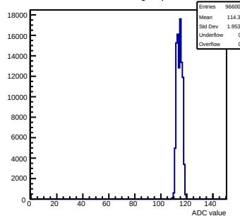
Pedestals mcm61-3214-rlv6-g0-s0-p1 ch 111 test1
