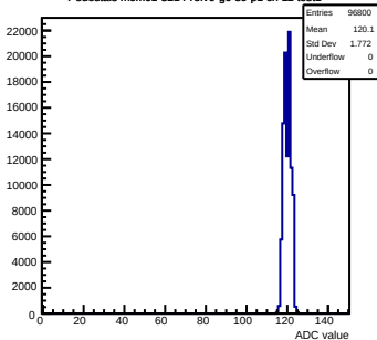
Pedestals mcm61-3214-rlv6-g0-s0-p1 ch 12 test1
