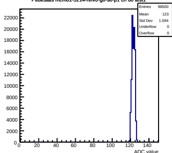
Pedestals mcm61-3214- rev6 -g0-s0-p1 ch 60 test1
