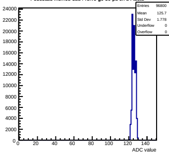
Pedestals mcm61-3214-rlv6-g0-s0-p1 ch 14 test1
