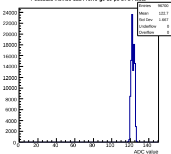
Pedestals mcm61-3214- rev6-g0-s0-p1 ch 24 test1
