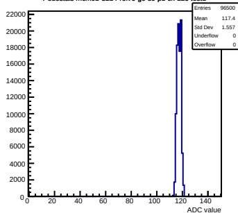
Pedestals mcm61-3214-refv6-g0-s0-p1 ch 125 test1
