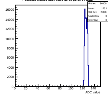
Pedestals mcm61-3214-refv6-g0-s0-p1 ch 64 test1
