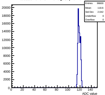
Pedestals mcm61-3214-rlv6-g0-s0-p1 ch 104 test1
