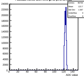
Pedestals mcm61-3214- rev6-g0-s0-p1 ch 22 test1
