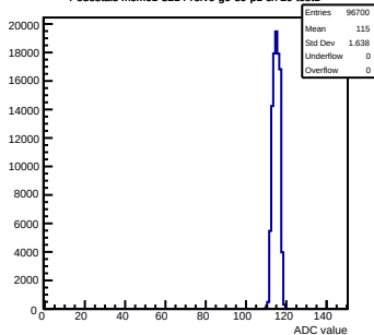
Pedestals mcm61-3214- rev6-g0-s0-p1 ch 29 test1
