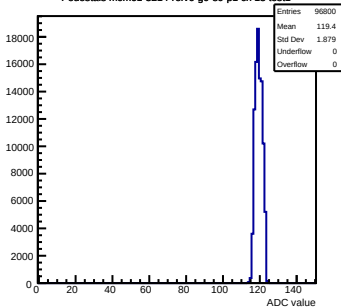
Pedestals mcm61-3214-rlv6-g0-s0-p1 ch 13 test1
