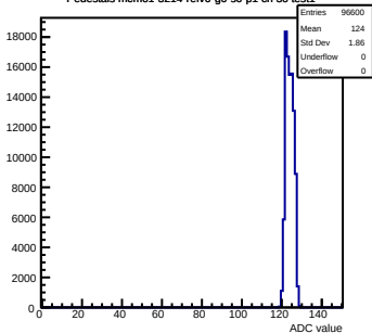
Pedestals mcm61-3214-rlv6-g0-s0-p1 ch 36 test1
