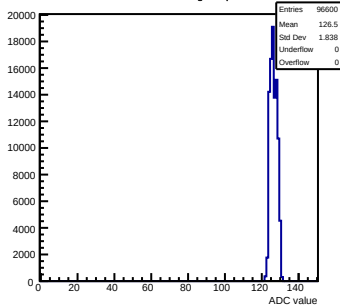
Pedestals mcm61-3214-rlv6-g0-s0-p1 ch 110 test1
