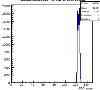
Pedestals mcm61-3214-refv6-g0-s0-p1 ch 65 test1
