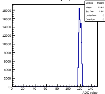
Pedestals mcm61-3214-rlv6-g0-s0-p1 ch 101 test1
