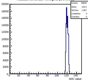
Pedestals mcm61-3214-rlv6-g0-s0-p1 ch 8 test1
