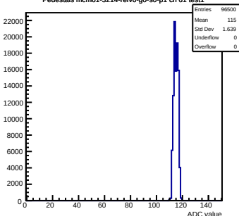
Pedestals mcm61-3214- rev6 -g0-s0-p1 ch 61 test1
