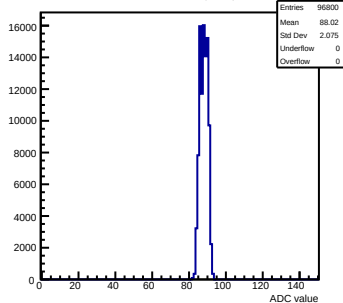
Pedestals mcm61-3214-refv1-g0-s0-p1 ch 7 test1
