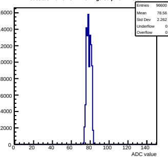
Pedestals mcm61-3214-refv1-g0-s0-p1 ch 41 test1
