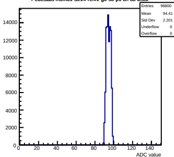
Pedestals mcm61-3214-refv1-g0-s0-p1 ch 68 test1
