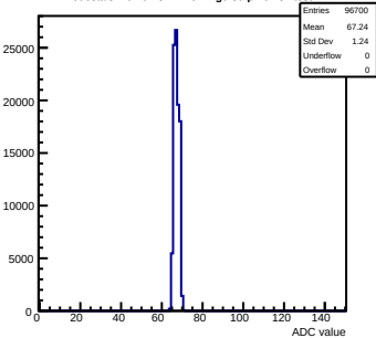
Pedestals mcm61-3214-refv2-g0-s0-p1 ch 84 test1
