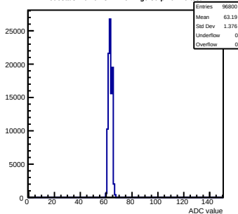
Pedestals mcm61-3214-refv2-g0-s0-p1 ch 70 test1
