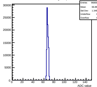
Pedestals mcm61-3214-refv2-g0-s0-p1 ch 79 test1
