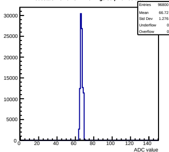
Pedestals mcm61-3214-refv2-g0-s0-p1 ch 66 test1
