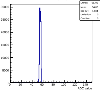
Pedestals mcm61-3214-refv2-g0-s0-p1 ch 92 test1
