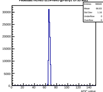
Pedestals mcm61-3214-refv2-g0-s0-p1 ch 53 test1
