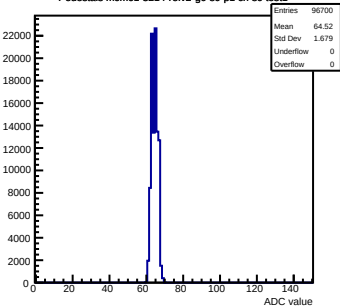
Pedestals mcm61-3214-refv2-g0-s0-p1 ch 80 test1
