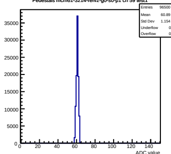
Pedestals mcm61-3214-refv2-g0-s0-p1 ch 59 test1
