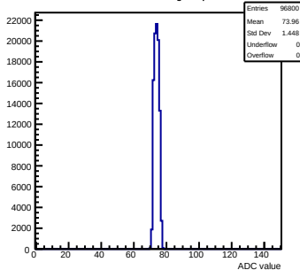
Pedestals mcm61-3214-refv2-g0-s0-p1 ch 74 test1
