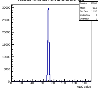
Pedestals mcm61-3214-refv2-g0-s0-p1 ch 17 test1
