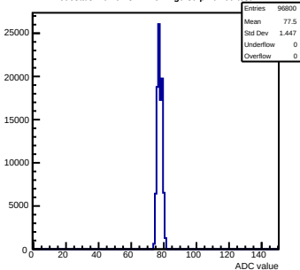
Pedestals mcm61-3214-refv2-g0-s0-p1 ch 69 test1
