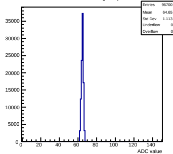
Pedestals mcm61-3214-refv2-g0-s0-p1 ch 94 test1
