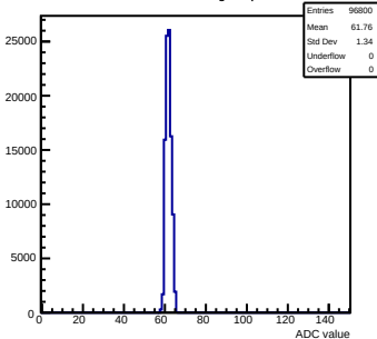
Pedestals mcm61-3214-refv2-g0-s0-p1 ch 73 test1
