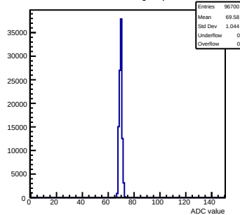
Pedestals mcm61-3214-refv2-g0-s0-p1 ch 90 test1
