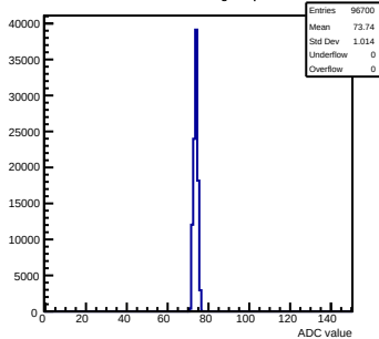
Pedestals mcm61-3214-refv2-g0-s0-p1 ch 93 test1
