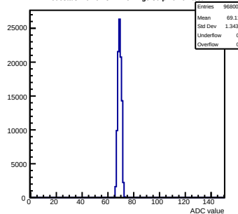
Pedestals mcm61-3214-refv2-g0-s0-p1 ch 67 test1
