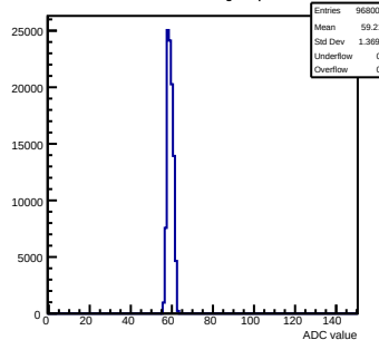
Pedestals mcm61-3214-refv2-g0-s0-p1 ch 75 test1
