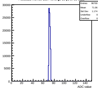
Pedestals mcm61-3214-refv2-g0-s0-p1 ch 30 test1
