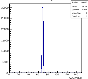
Pedestals mcm61-3214-refv2-g0-s0-p1 ch 65 test1
