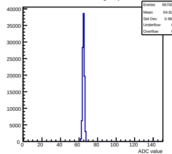
Pedestals mcm61-3214-refv2-g0-s0-p1 ch 95 test1
