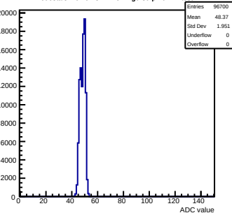
Pedestals mcm61-3214-refv4-g0-s0-p1 ch 21 test1
