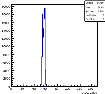
Pedestals mcm61-3214-refv4-g0-s0-p1 ch 31 test1
