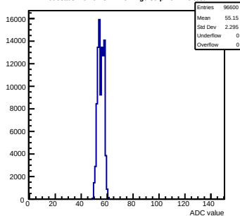
Pedestals mcm61-3214-refv4-g0-s0-p1 ch 110 test1
