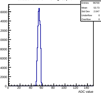
Pedestals mcm61-3214-refv4-g0-s0-p1 ch 17 test1
