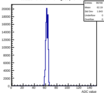
Pedestals mcm61-3214-refv4-g0-s0-p1 ch 23 test1
