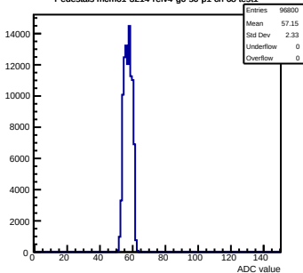
Pedestals mcm61-3214-refv4-g0-s0-p1 ch 68 test1
