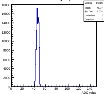
Pedestals mcm61-3214-refv4-g0-s0-p1 ch 19 test1
