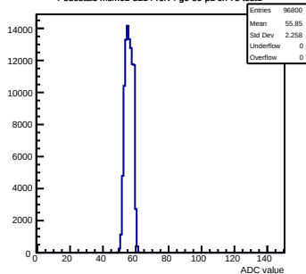
Pedestals mcm61-3214-refv4-g0-s0-p1 ch 78 test1
