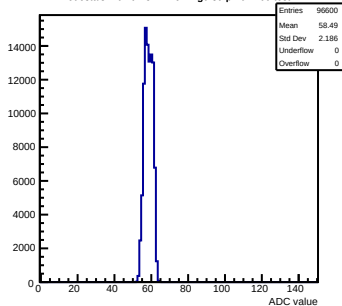
Pedestals mcm61-3214-refv4-g0-s0-p1 ch 109 test1
