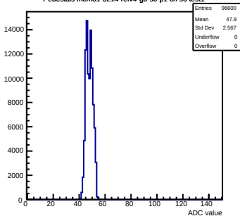
Pedestals mcm61-3214-refv4-g0-s0-p1 ch 96 test1
