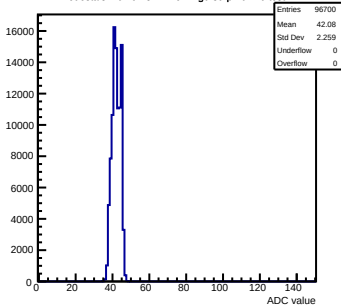
Pedestals mcm61-3214-refv4-g0-s0-p1 ch 20 test1
