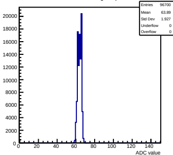
Pedestals mcm61-3214-refv4-g0-s0-p1 ch 27 test1
