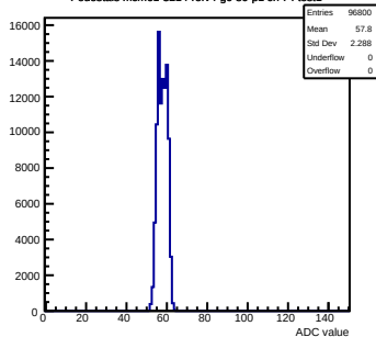
Pedestals mcm61-3214-refv4-g0-s0-p1 ch 74 test1
