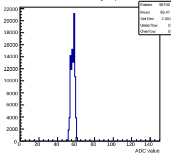
Pedestals mcm61-3214-refv4-g0-s0-p1 ch 26 test1
