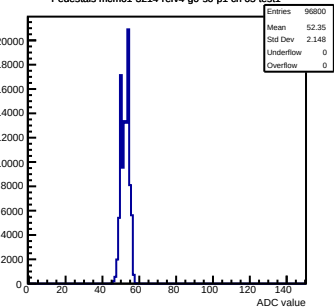
Pedestals mcm61-3214-refv4-g0-s0-p1 ch 65 test1
