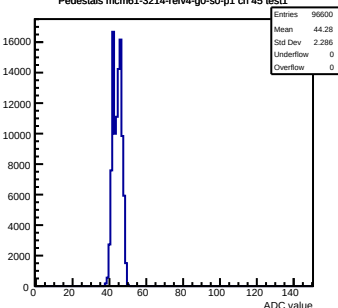
Pedestals mcm61-3214-4rfv4-g0-s0-p1 ch 45 test1
