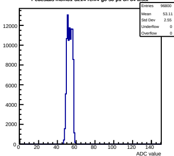
Pedestals mcm61-3214-refv4-g0-s0-p1 ch 64 test1
