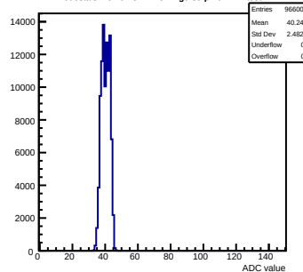
Pedestals mcm61-3214-refv4-g0-s0-p1 ch 111 test1
