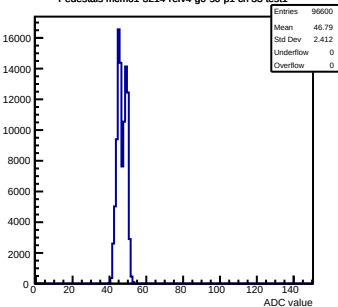
Pedestals mcm61-3214-4rfv4-g0-s0-p1 ch 33 test1
