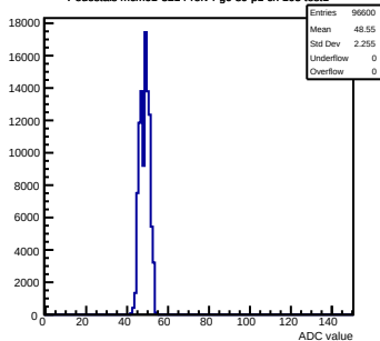
Pedestals mcm61-3214-refv4-g0-s0-p1 ch 105 test1
