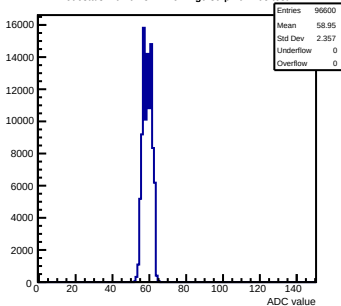
Pedestals mcm61-3214-refv4-g0-s0-p1 ch 108 test1
