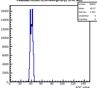
Pedestals mcm61-3214-4rfv4-g0-s0-p1 ch 41 test1
