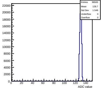
Pedestals mcm61-3214-rlv6-g0-s0-p1 ch 57 test1
