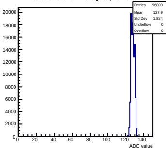
Pedestals mcm61-3214- rev6-g0-s0-p1 ch 76 test1
