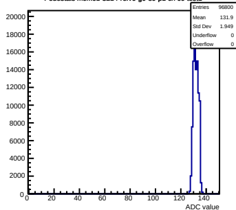
Pedestals mcm61-3214- rev6-g0-s0-p1 ch 69 test1
