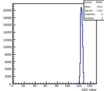
Pedestals mcm61-3214-rlv6-g0-s0-p1 ch 63 test1
