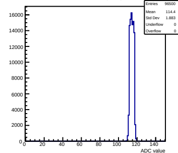
Pedestals mcm61-3214-rlv6-g0-s0-p1 ch 48 test1
