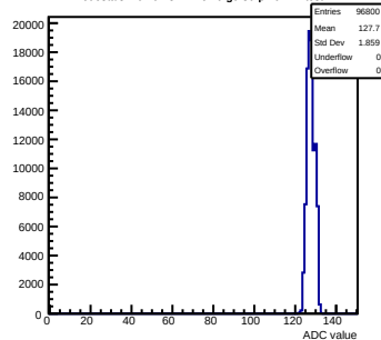
Pedestals mcm61-3214- rev6-g0-s0-p1 ch 74 test1
