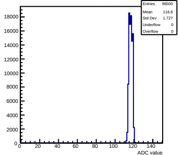
Pedestals mcm61-3214-rlv6-g0-s0-p1 ch 49 test1
