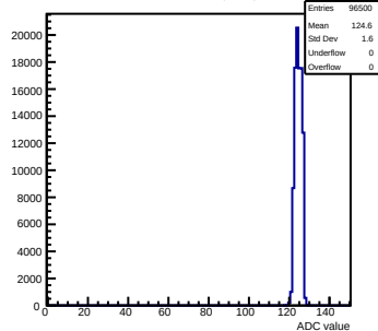
Pedestals mcm61-3214-rlv6-g0-s0-p1 ch 51 test1
