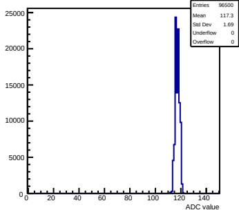
Pedestals mcm61-3214-rlv6-g0-s0-p1 ch 62 test1
