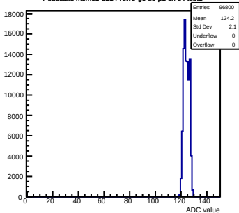
Pedestals mcm61-3214- rev6-g0-s0-p1 ch 64 test1
