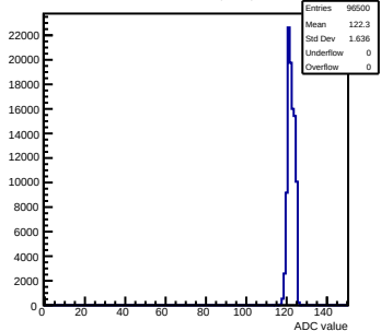
Pedestals mcm61-3214-rlv6-g0-s0-p1 ch 53 test1
