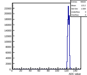
Pedestals mcm61-3214-rlv6-g0-s0-p1 ch 56 test1
