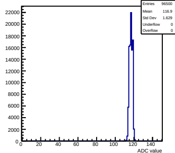
Pedestals mcm61-3214-rlv6-g0-s0-p1 ch 59 test1
