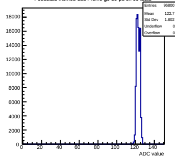
Pedestals mcm61-3214- rev6-g0-s0-p1 ch 66 test1
