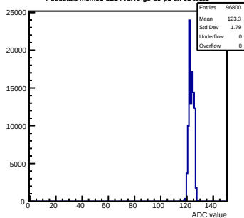
Pedestals mcm61-3214- rev6-g0-s0-p1 ch 65 test1
