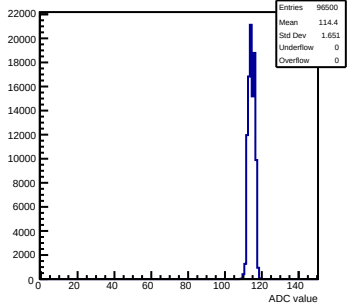
Pedestals mcm61-3214-rlv6-g0-s0-p1 ch 61 test1
