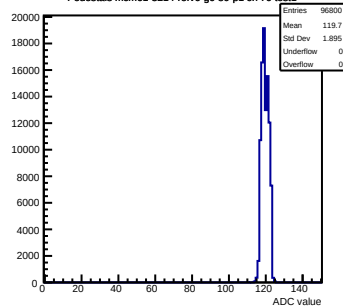
Pedestals mcm61-3214- rev6-g0-s0-p1 ch 70 test1
