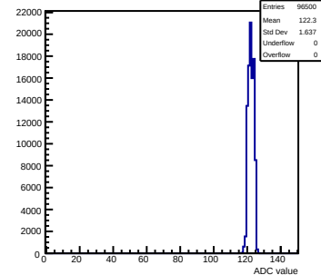
Pedestals mcm61-3214-rlv6-g0-s0-p1 ch 60 test1
