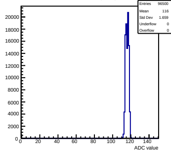
Pedestals mcm61-3214-rlv6-g0-s0-p1 ch 55 test1
