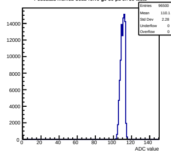
Pedestals mcm62-5612-refV0-g0-s0-p1 ch 59 test1
