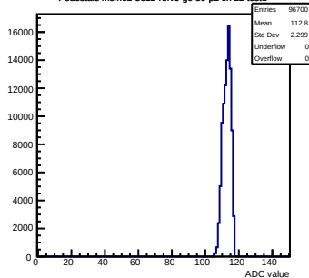
Pedestals mcm62-5612-refv0-g0-s0-p1 ch 22 test1
