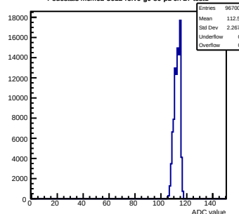
Pedestals mcm62-5612-refv0-g0-s0-p1 ch 27 test1
