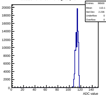
Pedestals mcm62-5612-refv0-g0-s0-p1 ch 124 test1
