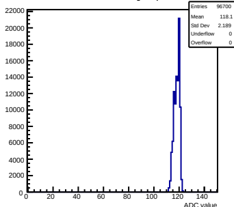
Pedestals mcm62-5612-refV0-g0-s0-p1 ch 94 test1
