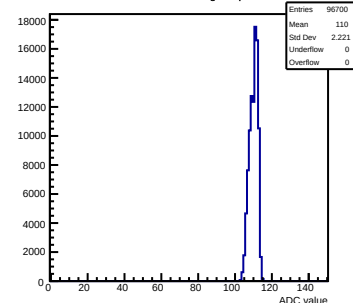
Pedestals mcm62-5612-refV0-g0-s0-p1 ch 92 test1
