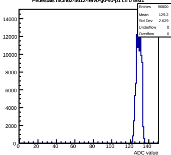
Pedestals mcm62-5612-refv0-g0-s0-p1 ch 0 test1
