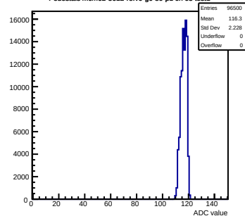
Pedestals mcm62-5612-refV0-g0-s0-p1 ch 63 test1
