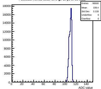
Pedestals mcm62-5612-refV0-g0-s0-p1 ch 61 test1
