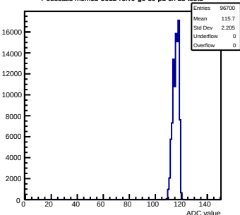
Pedestals mcm62-5612-refv0-g0-s0-p1 ch 28 test1
