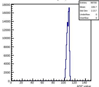
Pedestals mcm62-5612-refV0-g0-s0-p1 ch 89 test1
