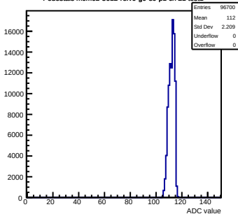
Pedestals mcm62-5612-refv0-g0-s0-p1 ch 21 test1
