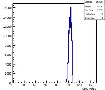
Pedestals mcm62-5612-refV0-g0-s0-p1 ch 83 test1
