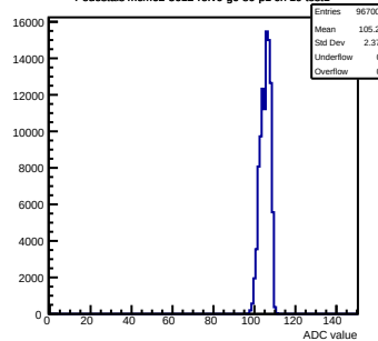
Pedestals mcm62-5612-refv0-g0-s0-p1 ch 19 test1
