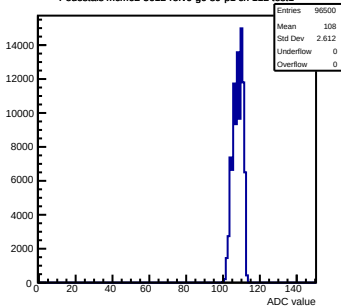
Pedestals mcm62-5612-refv0-g0-s0-p1 ch 112 test1
