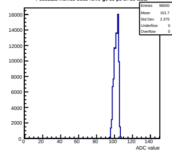
Pedestals mcm62-5612-refV0-g0-s0-p1 ch 56 test1
