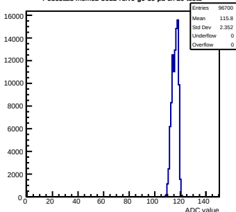
Pedestals mcm62-5612-refv0-g0-s0-p1 ch 29 test1
