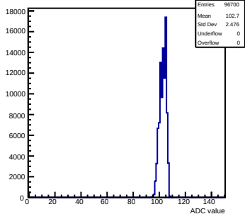
Pedestals mcm62-5612-refV0-g0-s0-p1 ch 81 test1
