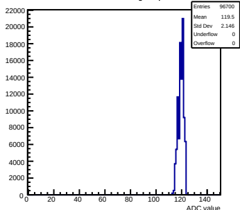
Pedestals mcm62-5612-refV0-g0-s0-p1 ch 93 test1
