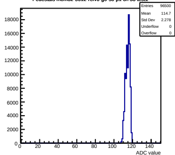
Pedestals mcm62-5612-refV0-g0-s0-p1 ch 53 test1
