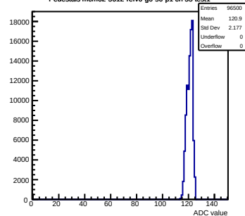
Pedestals mcm62-5612-refV0-g0-s0-p1 ch 55 test1
