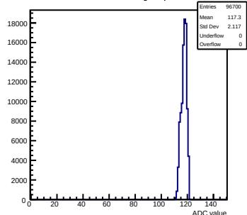
Pedestals mcm62-5612-refV0-g0-s0-p1 ch 91 test1
