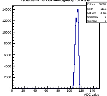
Pedestals mcm62-5612-refv0-g0-s0-p1 ch 6 test1
