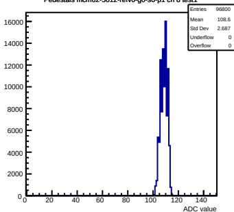
Pedestals mcm62-5612-refv0-g0-s0-p1 ch 8 test1
