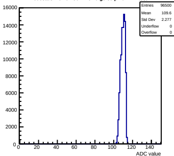
Pedestals mcm62-5612-refv0-g0-s0-p1 ch 122 test1
