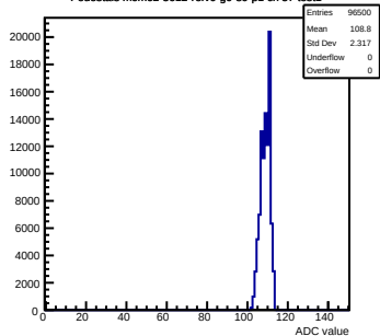
Pedestals mcm62-5612-refV0-g0-s0-p1 ch 57 test1
