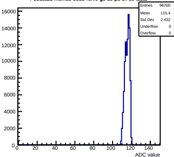
Pedestals mcm62-5612-refv0-g0-s0-p1 ch 20 test1
