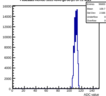
Pedestals mcm62-5612-refv0-g0-s0-p1 ch 11 test1
