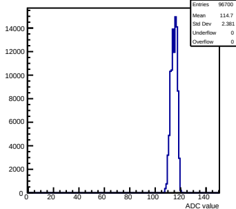
Pedestals mcm62-5612-refV0-g0-s0-p1 ch 82 test1
