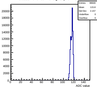
Pedestals mcm62-5612-refv0-g0-s0-p1 ch 125 test1
