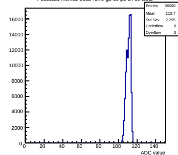
Pedestals mcm62-5612-refV0-g0-s0-p1 ch 60 test1
