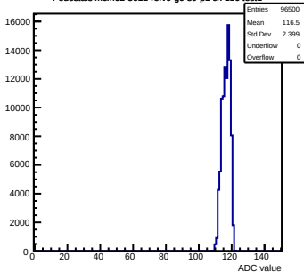
Pedestals mcm62-5612-refv0-g0-s0-p1 ch 116 test1
