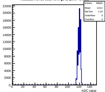
Pedestals mcm62-5612-refV0-g0-s0-p1 ch 49 test1
