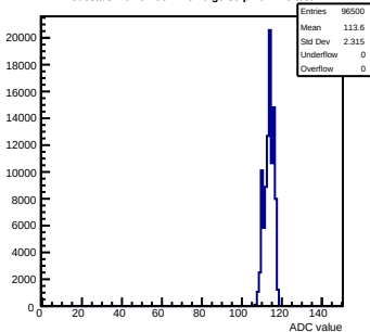
Pedestals mcm62-5612-refv0-g0-s0-p1 ch 126 test1
