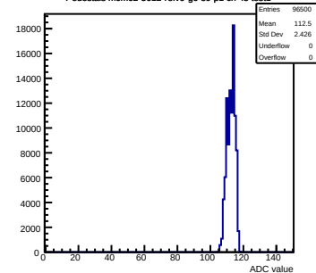
Pedestals mcm62-5612-refV0-g0-s0-p1 ch 48 test1
