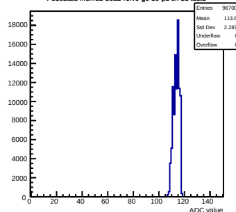
Pedestals mcm62-5612-refv0-g0-s0-p1 ch 31 test1
