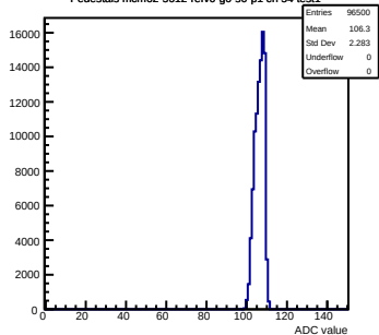
Pedestals mcm62-5612-refV0-g0-s0-p1 ch 54 test1
