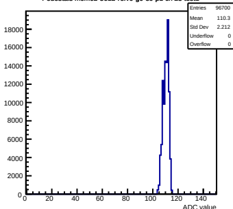
Pedestals mcm62-5612-refv0-g0-s0-p1 ch 25 test1
