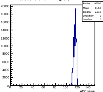
Pedestals mcm62-5612-refv0-g0-s0-p1 ch 24 test1
