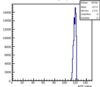
Pedestals mcm62-5612-refV0-g0-s0-p1 ch 95 test1
