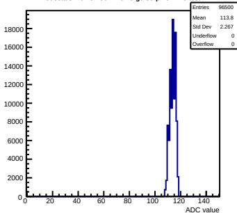
Pedestals mcm62-5612-refv0-g0-s0-p1 ch 120 test1
