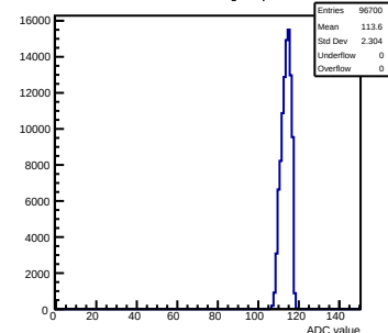
Pedestals mcm62-5612-refV0-g0-s0-p1 ch 88 test1
