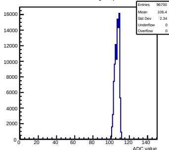
Pedestals mcm62-5612-refV0-g0-s0-p1 ch 90 test1
