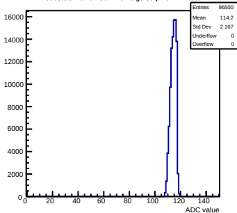
Pedestals mcm62-5612-refv0-g0-s0-p1 ch 121 test1
