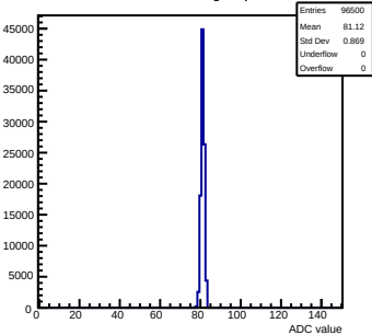
Pedestals mcm62-5612-refv1-g0-s0-p1 ch 60 test1
