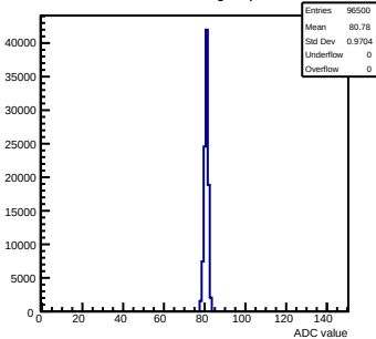
Pedestals mcm62-5612-refv1-g0-s0-p1 ch 62 test1
