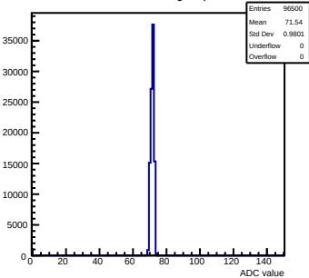
Pedestals mcm62-5612-refv1-g0-s0-p1 ch 56 test1
