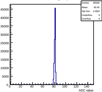
Pedestals mcm62-5612-refv1-g0-s0-p1 ch 59 test1
