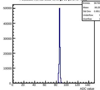
Pedestals mcm62-5612-rfv1-g0-s0-p1 ch 87 test1
