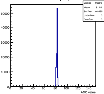
Pedestals mcm62-5612-refv1-g0-s0-p1 ch 52 test1
