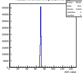
Pedestals mcm62-5612-rfv1-g0-s0-p1 ch 85 test1
