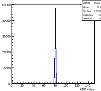
Pedestals mcm62-5612-refv1-g0-s0-p1 ch 57 test1
