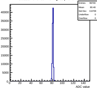
Pedestals mcm62-5612-rfv1-g0-s0-p1 ch 92 test1
