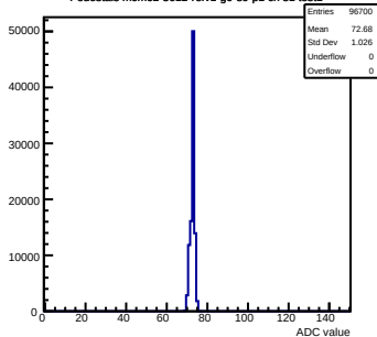
Pedestals mcm62-5612-rfv1-g0-s0-p1 ch 81 test1
