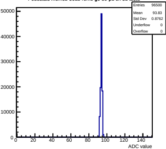
Pedestals mcm62-5612-refv1-g0-s0-p1 ch 51 test1
