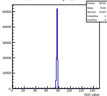
Pedestals mcm62-5612-rfv1-g0-s0-p1 ch 89 test1
