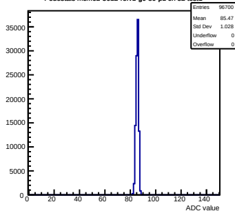
Pedestals mcm62-5612-rfv1-g0-s0-p1 ch 82 test1
