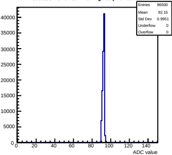
Pedestals mcm62-5612-refv1-g0-s0-p1 ch 55 test1
