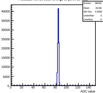
Pedestals mcm62-5612-refv1-g0-s0-p1 ch 50 test1
