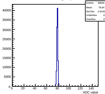
Pedestals mcm62-5612-refv1-g0-s0-p1 ch 61 test1
