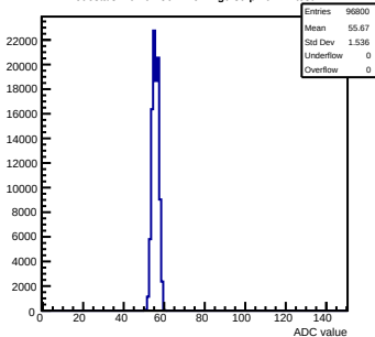
Pedestals mcm62-5612-refv2-g0-s0-p1 ch 12 test1
