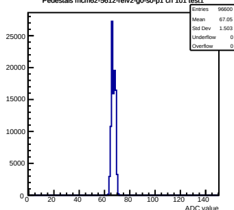
Pedestals mcm62-5612-refv2-g0-s0-p1 ch 101 test1
