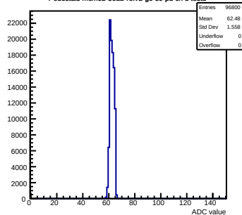
Pedestals mcm62-5612-refv2-g0-s0-p1 ch 3 test1
