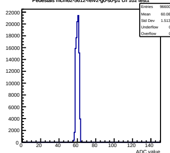
Pedestals mcm62-5612-refv2-g0-s0-p1 ch 102 test1
