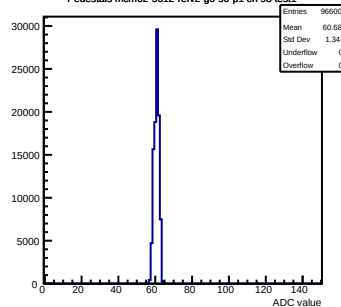
Pedestals mcm62-5612-refv2-g0-s0-p1 ch 98 test1
