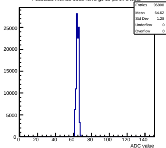
Pedestals mcm62-5612-refv2-g0-s0-p1 ch 2 test1
