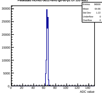
Pedestals mcm62-5612-refv2-g0-s0-p1 ch 120 test1
