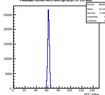
Pedestals mcm62-5612-refv2-g0-s0-p1 ch 110 test1
