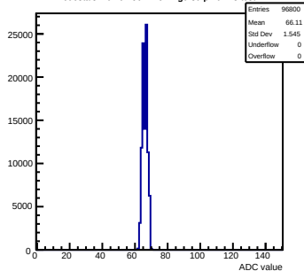
Pedestals mcm62-5612-refv2-g0-s0-p1 ch 13 test1
