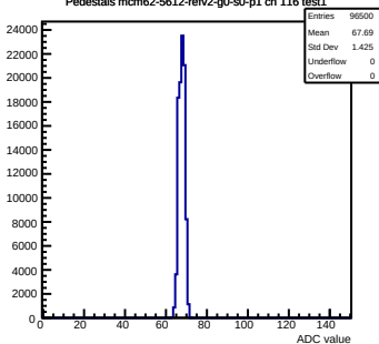
Pedestals mcm62-5612-refv2-g0-s0-p1 ch 116 test1
