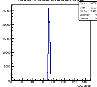
Pedestals mcm62-5612-refv2-g0-s0-p1 ch 97 test1
