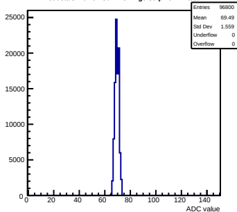
Pedestals mcm62-5612-refv2-g0-s0-p1 ch 14 test1
