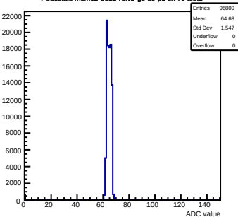
Pedestals mcm62-5612-refv2-g0-s0-p1 ch 76 test1
