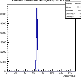
Pedestals mcm62-5612-refv2-g0-s0-p1 ch 121 test1
