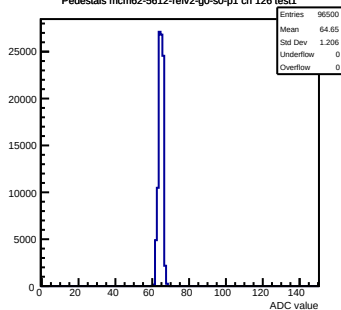
Pedestals mcm62-5612-refv2-g0-s0-p1 ch 126 test1
