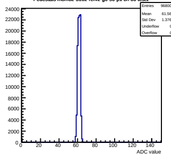
Pedestals mcm62-5612-refv2-g0-s0-p1 ch 66 test1
