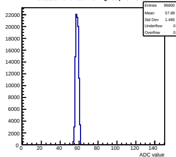
Pedestals mcm62-5612-refv2-g0-s0-p1 ch 15 test1
