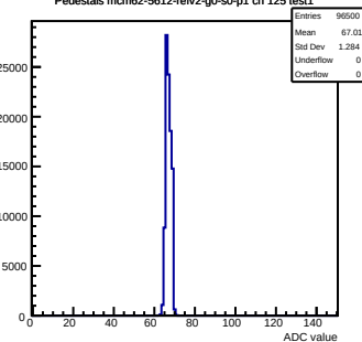
Pedestals mcm62-5612-refv2-g0-s0-p1 ch 125 test1
