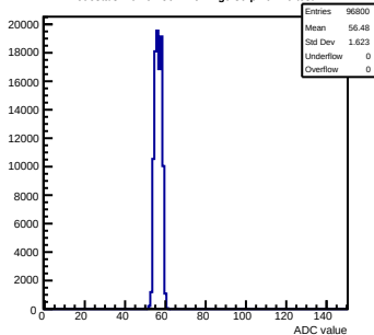
Pedestals mcm62-5612-refv2-g0-s0-p1 ch 10 test1
