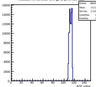
Pedestals mcm62-5612-refv6-g0-s0-p1 ch 106 test1
