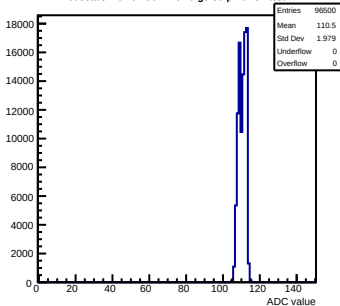
Pedestals mcm62-5612- rev6-g0-s0-p1 ch 57 test1
