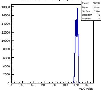
Pedestals mcm62-5612-rlfv6-g0-s0-p1 ch 14 test1
