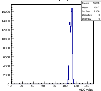
Pedestals mcm62-5612-rlfv6-g0-s0-p1 ch 15 test1
