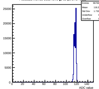
Pedestals mcm62-5612-refv6-g0-s0-p1 ch 87 test1
