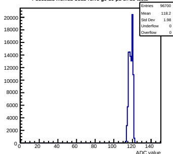
Pedestals mcm62-5612- rfv6-g0-s0-p1 ch 29 test1
