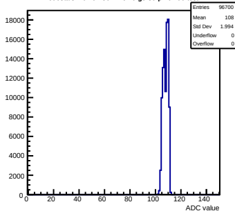
Pedestals mcm62-5612-refv6-g0-s0-p1 ch 90 test1
