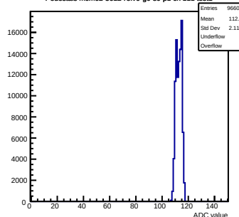
Pedestals mcm62-5612-refv6-g0-s0-p1 ch 111 test1
