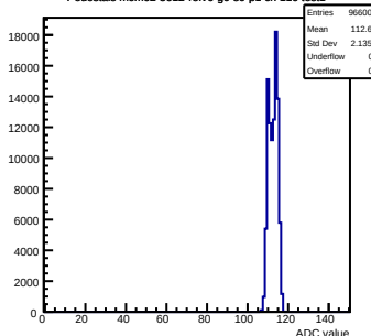
Pedestals mcm62-5612-refv6-g0-s0-p1 ch 110 test1
