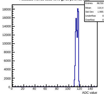
Pedestals mcm62-5612- rfv6-g0-s0-p1 ch 22 test1
