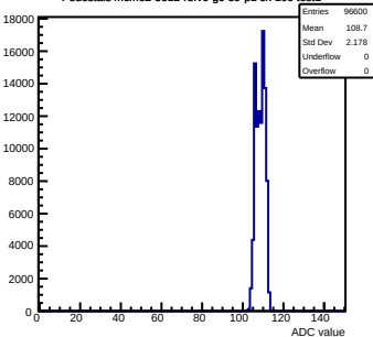
Pedestals mcm62-5612-refv6-g0-s0-p1 ch 96 test1
