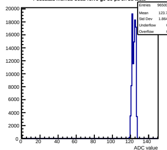
Pedestals mcm62-5612- rev6-g0-s0-p1 ch 51 test1
