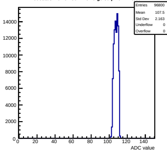
Pedestals mcm62-5612-rlfv6-g0-s0-p1 ch 12 test1
