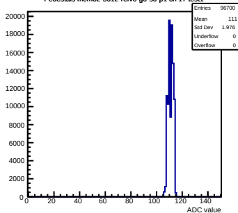
Pedestals mcm62-5612- rfv6-g0-s0-p1 ch 17 test1
