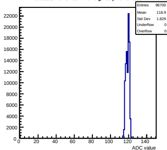
Pedestals mcm62-5612-refv6-g0-s0-p1 ch 94 test1
