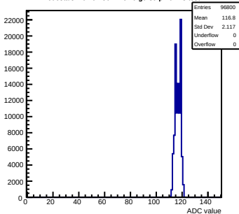
Pedestals mcm62-5612-rlfv6-g0-s0-p1 ch 13 test1
