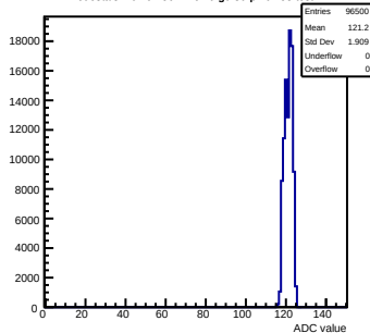
Pedestals mcm62-5612- rev6-g0-s0-p1 ch 58 test1
