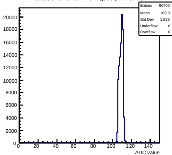
Pedestals mcm62-5612-refv6-g0-s0-p1 ch 89 test1
