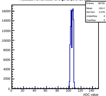
Pedestals mcm62-5612-refv6-g0-s0-p1 ch 81 test1
