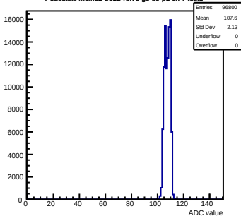
Pedestals mcm62-5612-rlfv6-g0-s0-p1 ch 7 test1
