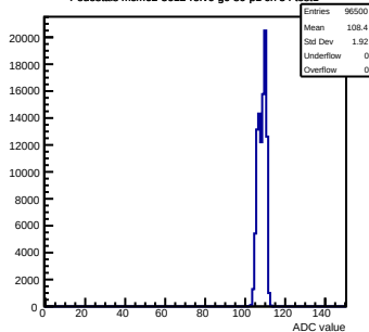
Pedestals mcm62-5612- rev6-g0-s0-p1 ch 54 test1
