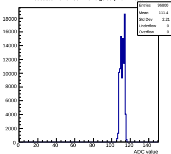
Pedestals mcm62-5612-rlfv6-g0-s0-p1 ch 11 test1
