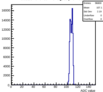
Pedestals mcm62-5612-rlfv6-g0-s0-p1 ch 10 test1
