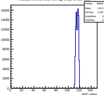
Pedestals mcm62-5612-refv6-g0-s0-p1 ch 105 test1
