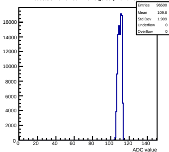
Pedestals mcm62-5612- rev6-g0-s0-p1 ch 61 test1
