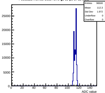
Pedestals mcm62-5612- rev6-g0-s0-p1 ch 52 test1
