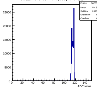
Pedestals mcm62-5612- rfv6-g0-s0-p1 ch 31 test1
