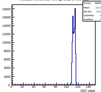
Pedestals mcm62-5612-refv6-g0-s0-p1 ch 102 test1
