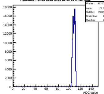
Pedestals mcm62-5612- rfv6-g0-s0-p1 ch 19 test1
