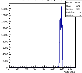
Pedestals mcm62-5612-refv6-g0-s0-p1 ch 84 test1
