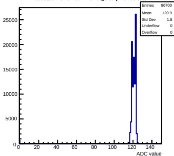
Pedestals mcm62-5612-refv6-g0-s0-p1 ch 93 test1
