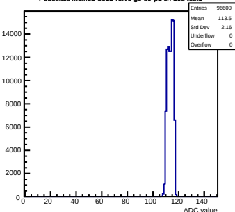
Pedestals mcm62-5612-refv6-g0-s0-p1 ch 104 test1
