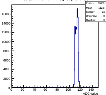
Pedestals mcm62-5612-rlfv6-g0-s0-p1 ch 6 test1
