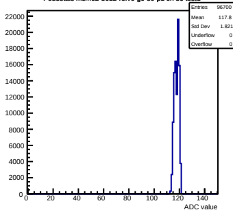
Pedestals mcm62-5612-refv6-g0-s0-p1 ch 86 test1
