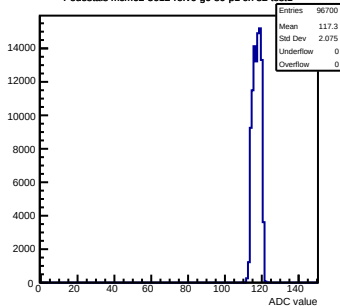
Pedestals mcm62-5612-refv6-g0-s0-p1 ch 82 test1
