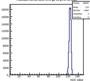
Pedestals mcm63-3611-refV0-g0-s0-p1 ch 98 test1
