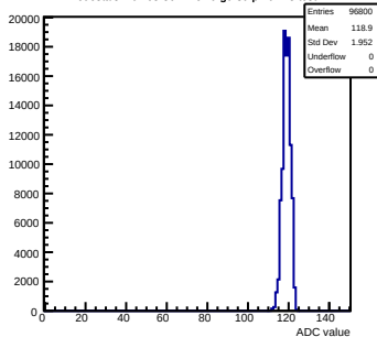
Pedestals mcm63-3611-refV0-g0-s0-p1 ch 73 test1
