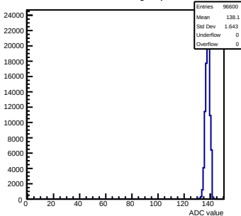
Pedestals mcm63-3611-refV0-g0-s0-p1 ch 46 test1
