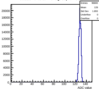
Pedestals mcm63-3611-refV0-g0-s0-p1 ch 78 test1
