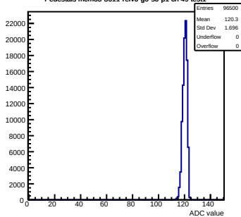
Pedestals mcm63-3611-refV0-g0-s0-p1 ch 49 test1
