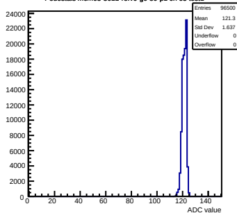
Pedestals mcm63-3611-refV0-g0-s0-p1 ch 63 test1
