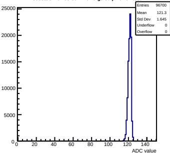
Pedestals mcm63-3611- \text{rev0-g0-s0-p1} ch 92 test1
