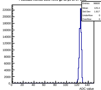
Pedestals mcm63-3611-refV0-g0-s0-p1 ch 97 test1
