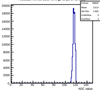
Pedestals mcm63-3611-refV0-g0-s0-p1 ch 68 test1
