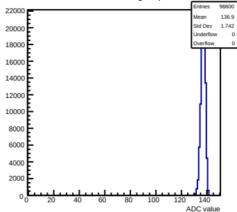
Pedestals mcm63-3611-refV0-g0-s0-p1 ch 45 test1
