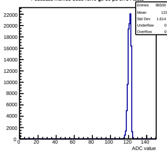
Pedestals mcm63-3611-refV0-g0-s0-p1 ch 54 test1
