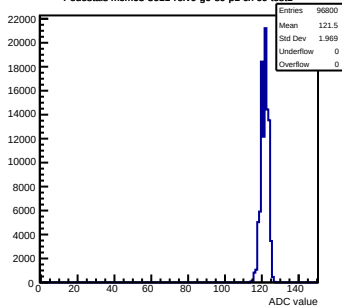
Pedestals mcm63-3611-refV0-g0-s0-p1 ch 69 test1
