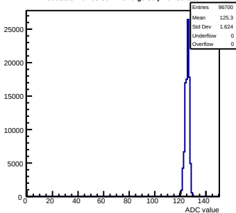
Pedestals mcm63-3611- \text{rev0-g0-s0-p1} ch 89 test1
