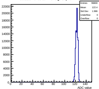
Pedestals mcm63-3611-refV0-g0-s0-p1 ch 72 test1
