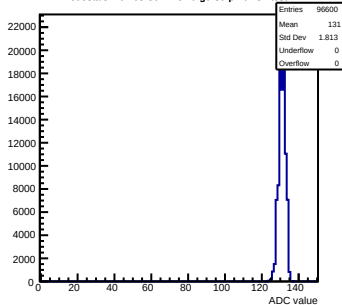
Pedestals mcm63-3611-refV0-g0-s0-p1 ch 37 test1
