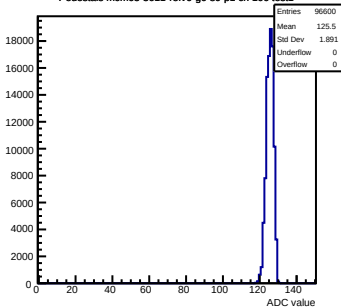
Pedestals mcm63-3611-refV0-g0-s0-p1 ch 106 test1
