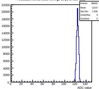
Pedestals mcm63-3611-refV0-g0-s0-p1 ch 110 test1
