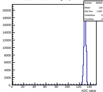
Pedestals mcm63-3611-refV0-g0-s0-p1 ch 35 test1
