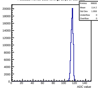
Pedestals mcm63-3611-refV0-g0-s0-p1 ch 105 test1
