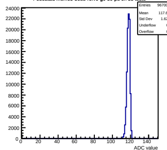
Pedestals mcm63-3611- \text{rev0-g0-s0-p1} ch 83 test1
