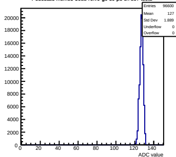
Pedestals mcm63-3611-refV0-g0-s0-p1 ch 107 test1
