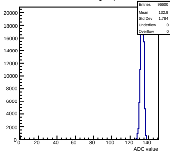
Pedestals mcm63-3611-refV0-g0-s0-p1 ch 33 test1
