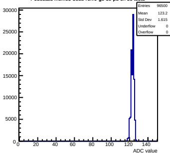
Pedestals mcm63-3611-refV0-g0-s0-p1 ch 56 test1
