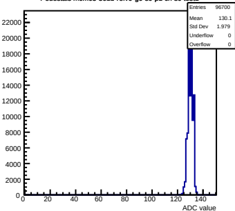
Pedestals mcm63-3611- \text{rev0-g0-s0-p1} ch 80 test1
