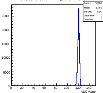
Pedestals mcm63-3611- \text{rev0-g0-s0-p1} ch 85 test1
