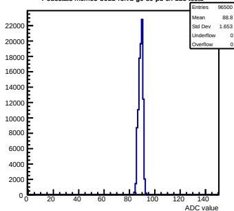
Pedestals mcm63-3611-refv1-g0-s0-p1 ch 118 test1
