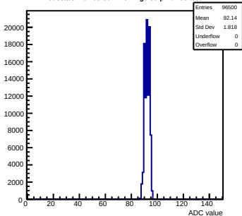
Pedestals mcm63-3611-refv1-g0-s0-p1 ch 56 test1
