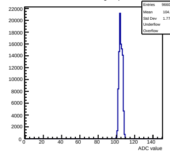
Pedestals mcm63-3611-refv1-g0-s0-p1 ch 47 test1
