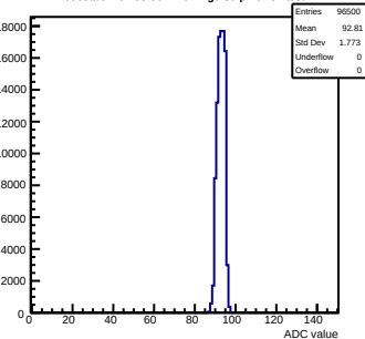
Pedestals mcm63-3611-refv1-g0-s0-p1 ch 57 test1
