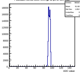
Pedestals mcm63-3611-refv1-g0-s0-p1 ch 114 test1
