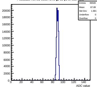
Pedestals mcm63-3611-refv1-g0-s0-p1 ch 119 test1
