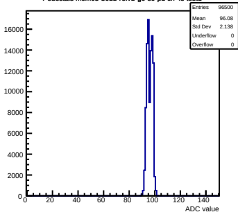
Pedestals mcm63-3611-refv1-g0-s0-p1 ch 48 test1
