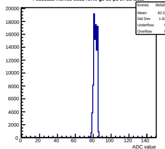
Pedestals mcm63-3611-refv1-g0-s0-p1 ch 51 test1
