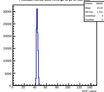
Pedestals mcm63-3611-refv3-g0-s0-p1 ch 103 test1
