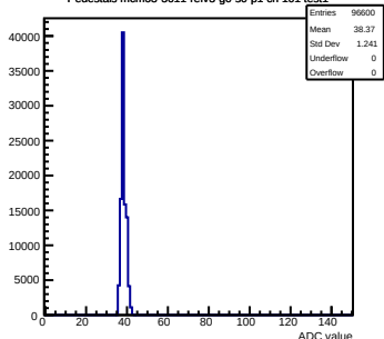
Pedestals mcm63-3611-refv3-g0-s0-p1 ch 101 test1
