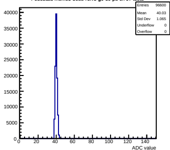
Pedestals mcm63-3611-refv3-g0-s0-p1 ch 97 test1
