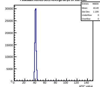
Pedestals mcm63-3611-refv3-g0-s0-p1 ch 108 test1
