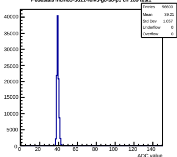
Pedestals mcm63-3611-refv3-g0-s0-p1 ch 109 test1
