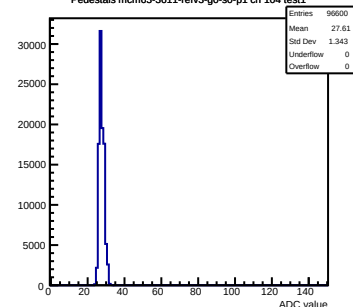
Pedestals mcm63-3611-refv3-g0-s0-p1 ch 104 test1
