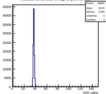
Pedestals mcm63-3611-refv3-g0-s0-p1 ch 98 test1
