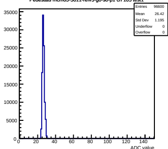
Pedestals mcm63-3611-refv3-g0-s0-p1 ch 105 test1
