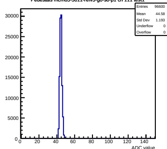
Pedestals mcm63-3611-refv3-g0-s0-p1 ch 111 test1
