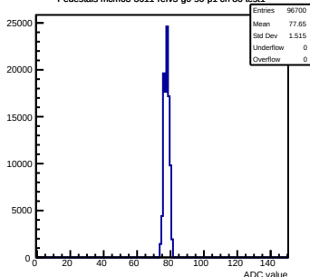
Pedestals mcm63-3611-refV5-g0-s0-p1 ch 86 test1
