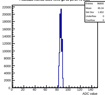
Pedestals mcm63-3611-refV5-g0-s0-p1 ch 70 test1
