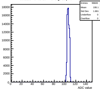
Pedestals mcm63-3611- rev5-g0-s0-p1 ch 44 test1
