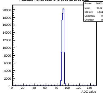
Pedestals mcm63-3611-refV5-g0-s0-p1 ch 55 test1
