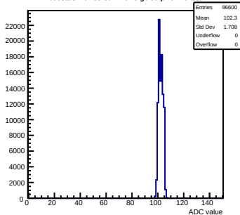
Pedestals mcm63-3611- rev5-g0-s0-p1 ch 46 test1
