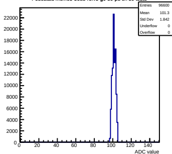
Pedestals mcm63-3611- rev5-g0-s0-p1 ch 39 test1
