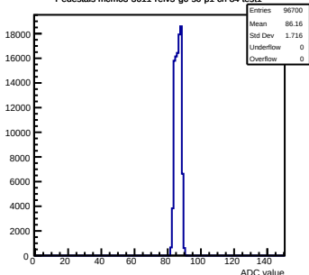
Pedestals mcm63-3611-refV5-g0-s0-p1 ch 84 test1
