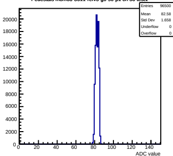
Pedestals mcm63-3611-refV5-g0-s0-p1 ch 50 test1
