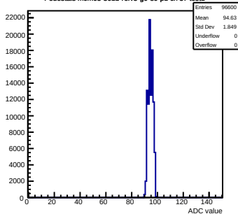
Pedestals mcm63-3611- rev5-g0-s0-p1 ch 37 test1
