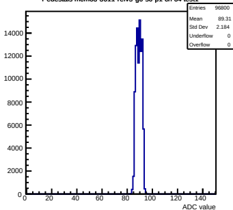
Pedestals mcm63-3611-refV5-g0-s0-p1 ch 64 test1
