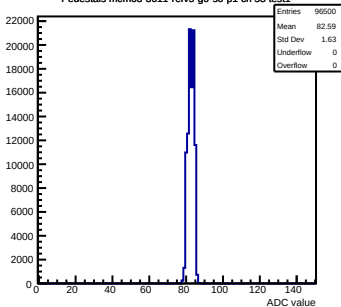
Pedestals mcm63-3611-refV5-g0-s0-p1 ch 53 test1
