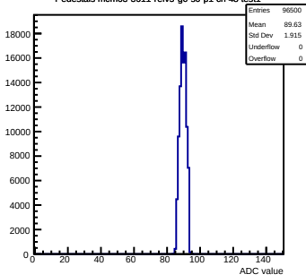
Pedestals mcm63-3611-refV5-g0-s0-p1 ch 48 test1
