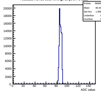
Pedestals mcm63-3611-refV5-g0-s0-p1 ch 75 test1
