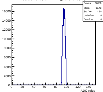
Pedestals mcm63-3611- rev5-g0-s0-p1 ch 35 test1
