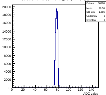
Pedestals mcm63-3611-refV5-g0-s0-p1 ch 82 test1
