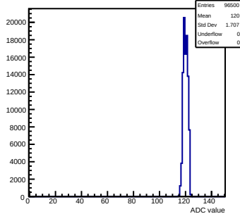
Pedestals mcm70-5012-refV0-g0-s0-p1 ch 57 test1
