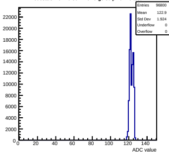
Pedestals mcm70-5012-refV0-g0-s0-p1 ch 76 test1
