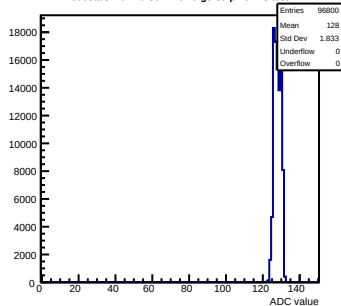
Pedestals mcm70-5012-refV0-g0-s0-p1 ch 73 test1
