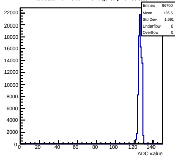
Pedestals mcm70-5012-refV0-g0-s0-p1 ch 89 test1
