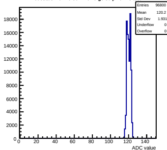
Pedestals mcm70-5012-refV0-g0-s0-p1 ch 78 test1
