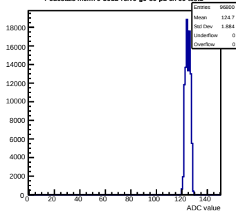
Pedestals mcm70-5012-refV0-g0-s0-p1 ch 69 test1
