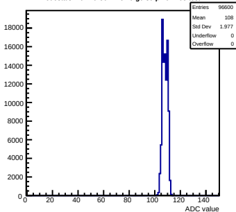
Pedestals mcm70-5012-refV0-g0-s0-p1 ch 105 test1
