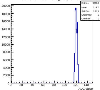
Pedestals mcm70-5012-refV0-g0-s0-p1 ch 46 test1
