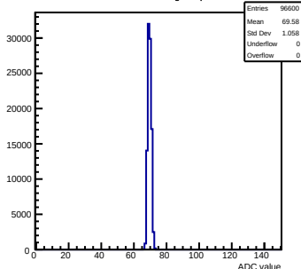
Pedestals mcm70-5012-refv2-g0-s0-p1 ch 110 test1
