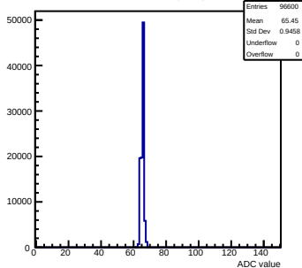
Pedestals mcm70-5012-refv2-g0-s0-p1 ch 97 test1
