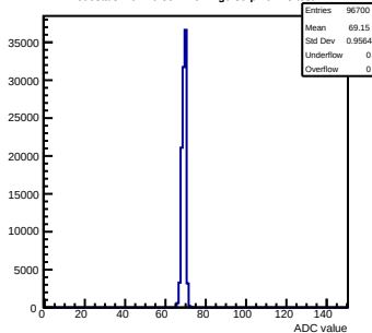
Pedestals mcm70-5012-refv2-g0-s0-p1 ch 18 test1
