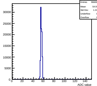
Pedestals mcm70-5012-refv2-g0-s0-p1 ch 99 test1
