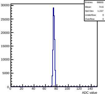
Pedestals mcm70-5012-refv2-g0-s0-p1 ch 100 test1
