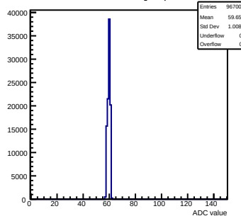
Pedestals mcm70-5012-refv2-g0-s0-p1 ch 27 test1
