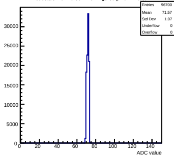
Pedestals mcm70-5012-refv2-g0-s0-p1 ch 21 test1
