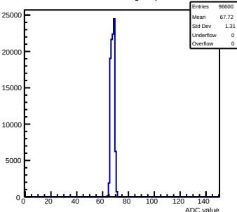
Pedestals mcm70-5012-refv2-g0-s0-p1 ch 104 test1
