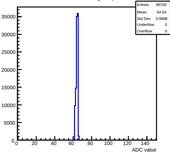
Pedestals mcm70-5012-refv2-g0-s0-p1 ch 28 test1
