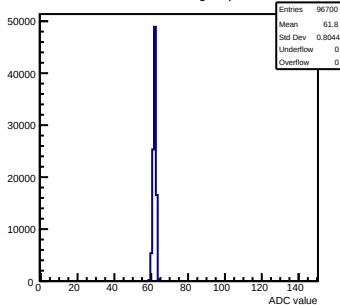
Pedestals mcm70-5012-refv2-g0-s0-p1 ch 30 test1
