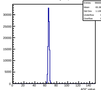
Pedestals mcm70-5012-refv2-g0-s0-p1 ch 107 test1
