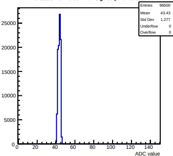
Pedestals mcm70-5012-refv3-g0-s0-p1 ch 56 test1
