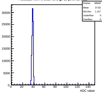
Pedestals mcm70-5012-refv3-g0-s0-p1 ch 53 test1
