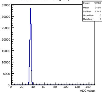
Pedestals mcm70-5012-refv3-g0-s0-p1 ch 57 test1
