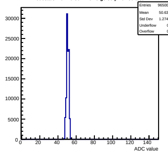
Pedestals mcm70-5012-refv3-g0-s0-p1 ch 59 test1
