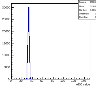
Pedestals mcm70-5012-refv3-g0-s0-p1 ch 41 test1
