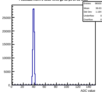
Pedestals mcm70-5012-refv3-g0-s0-p1 ch 50 test1
