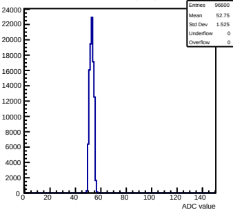
Pedestals mcm70-5012-refv3-g0-s0-p1 ch 36 test1
