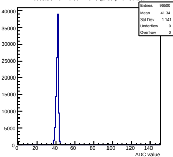
Pedestals mcm70-5012-refv3-g0-s0-p1 ch 60 test1
