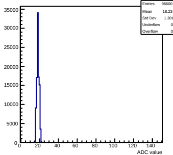
Pedestals mcm70-5012-refv3-g0-s0-p1 ch 37 test1
