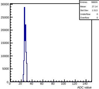
Pedestals mcm70-5012-refv3-g0-s0-p1 ch 40 test1
