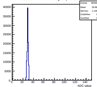
Pedestals mcm70-5012-refv3-g0-s0-p1 ch 63 test1
