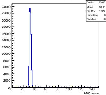
Pedestals mcm70-5012-refv3-g0-s0-p1 ch 38 test1
