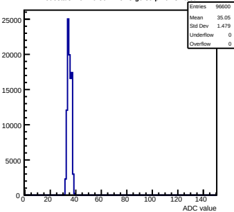
Pedestals mcm70-5012-refv3-g0-s0-p1 ch 32 test1
