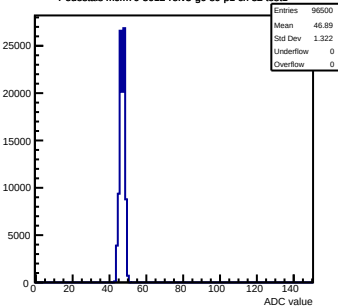
Pedestals mcm70-5012-refv3-g0-s0-p1 ch 52 test1
