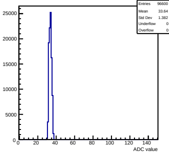
Pedestals mcm70-5012-refv3-g0-s0-p1 ch 46 test1
