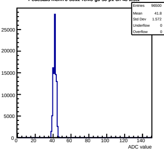
Pedestals mcm70-5012-refv3-g0-s0-p1 ch 48 test1
