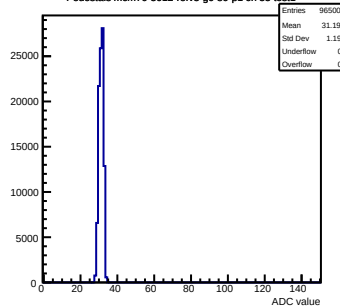
Pedestals mcm70-5012-refv3-g0-s0-p1 ch 55 test1
