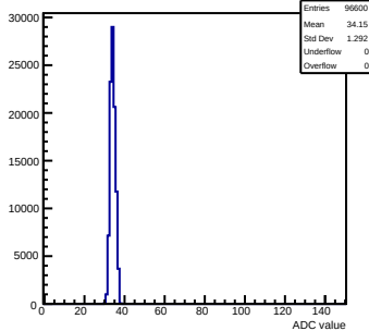
Pedestals mcm70-5012-refv3-g0-s0-p1 ch 45 test1
