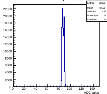
Pedestals mcm70-5012-refV5-g0-s0-p1 ch 35 test1
