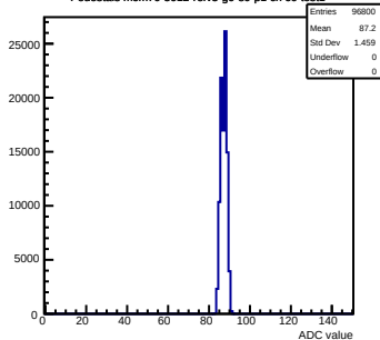
Pedestals mcm70-5012-refv5-g0-s0-p1 ch 69 test1
