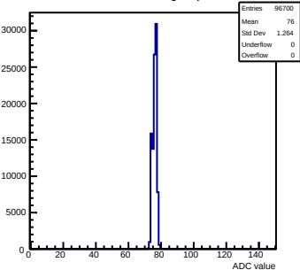
Pedestals mcm70-5012-rvF5-g0-s0-p1 ch 27 test1
