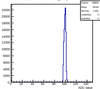
Pedestals mcm70-5012-refV5-g0-s0-p1 ch 36 test1
