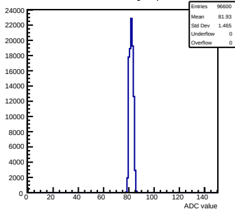
Pedestals mcm70-5012-refV5-g0-s0-p1 ch 46 test1
