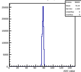
Pedestals mcm70-5012-refV5-g0-s0-p1 ch 42 test1
