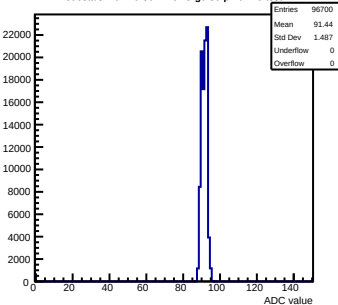
Pedestals mcm70-5012-rvF5-g0-s0-p1 ch 20 test1
