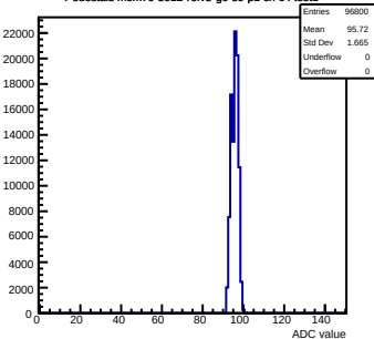
Pedestals mcm70-5012-refv5-g0-s0-p1 ch 64 test1
