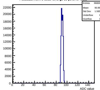
Pedestals mcm70-5012-refv5-g0-s0-p1 ch 67 test1
