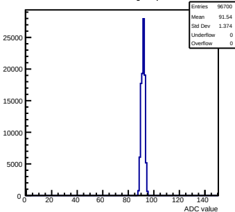
Pedestals mcm70-5012-rvF5-g0-s0-p1 ch 26 test1
