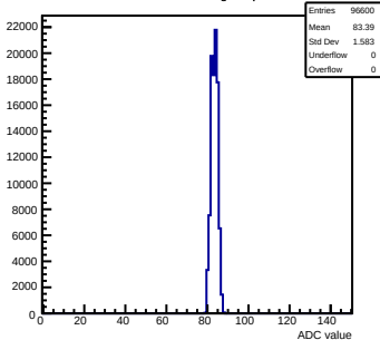
Pedestals mcm70-5012-refV5-g0-s0-p1 ch 44 test1
