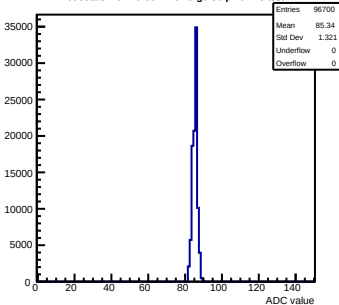
Pedestals mcm70-5012-rvF5-g0-s0-p1 ch 18 test1
