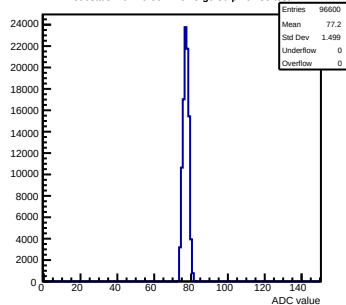
Pedestals mcm70-5012-refV5-g0-s0-p1 ch 39 test1
