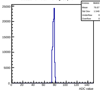
Pedestals mcm70-5012-refv5-g0-s0-p1 ch 74 test1
