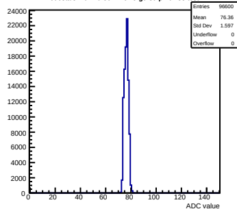
Pedestals mcm70-5012-refV5-g0-s0-p1 ch 33 test1
