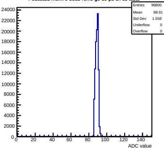
Pedestals mcm70-5012-refv5-g0-s0-p1 ch 68 test1
