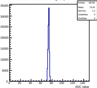
Pedestals mcm70-5012-rvF5-g0-s0-p1 ch 19 test1
