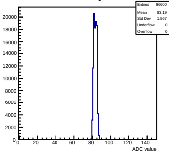
Pedestals mcm70-5012-refV5-g0-s0-p1 ch 32 test1
