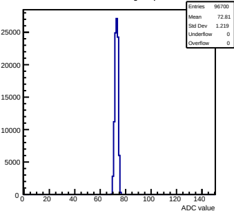
Pedestals mcm70-5012-rvF5-g0-s0-p1 ch 31 test1
