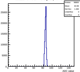
Pedestals mcm70-5012-refv5-g0-s0-p1 ch 76 test1
