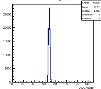
Pedestals mcm70-5012-refV5-g0-s0-p1 ch 37 test1
