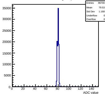
Pedestals mcm70-5012-rvF5-g0-s0-p1 ch 25 test1
