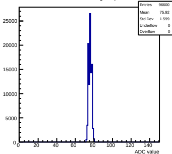
Pedestals mcm70-5012-refV5-g0-s0-p1 ch 40 test1
