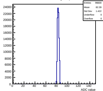
Pedestals mcm70-5012-refV5-g0-s0-p1 ch 45 test1
