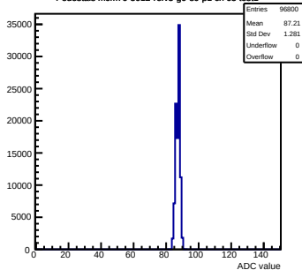
Pedestals mcm70-5012-refv5-g0-s0-p1 ch 65 test1
