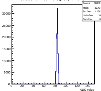
Pedestals mcm70-5012-refv5-g0-s0-p1 ch 66 test1
