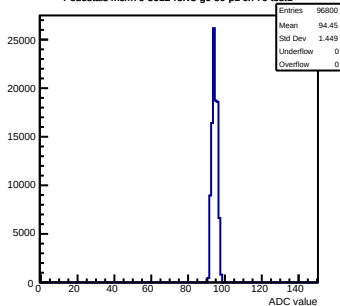
Pedestals mcm70-5012-refv5-g0-s0-p1 ch 70 test1
