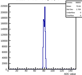
Pedestals mcm70-5012-refv5-g0-s0-p1 ch 72 test1
