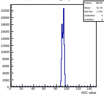
Pedestals mcm70-5012-rvF5-g0-s0-p1 ch 16 test1
