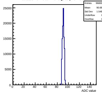
Pedestals mcm70-5012-refv5-g0-s0-p1 ch 79 test1
