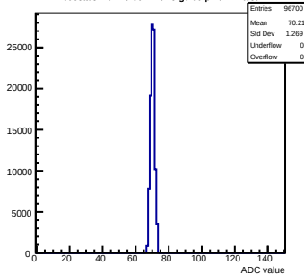
Pedestals mcm70-5012-rvF5-g0-s0-p1 ch 17 test1
