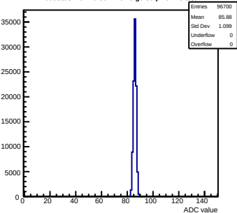
Pedestals mcm70-5012-rvF5-g0-s0-p1 ch 23 test1
