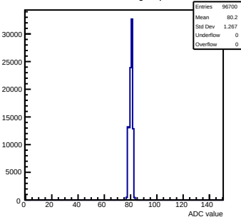
Pedestals mcm70-5012-rvF5-g0-s0-p1 ch 28 test1
