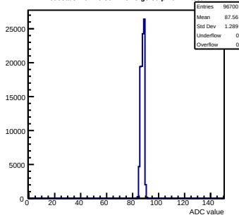
Pedestals mcm70-5012-rvF5-g0-s0-p1 ch 21 test1
