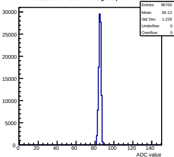
Pedestals mcm70-5012-rvF5-g0-s0-p1 ch 22 test1
