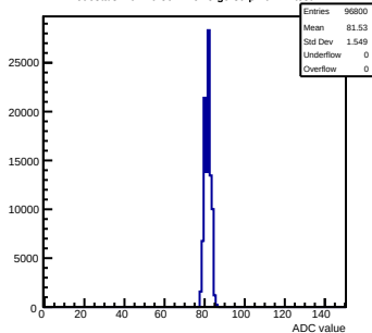
Pedestals mcm70-5012-refv5-g0-s0-p1 ch 77 test1
