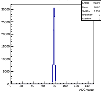
Pedestals mcm70-5012-rvF5-g0-s0-p1 ch 30 test1
