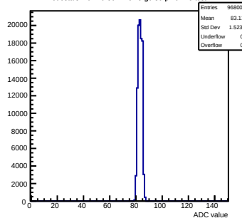
Pedestals mcm70-5012-refv5-g0-s0-p1 ch 75 test1
