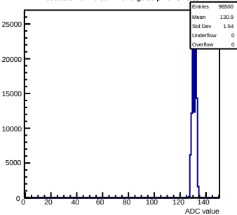
Pedestals mcm70-5012- refv6-g0-s0-p1 ch 52 test1
