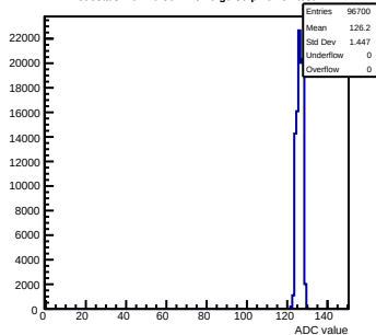
Pedestals mcm70-5012- rev6-g0-s0-p1 ch 94 test1
