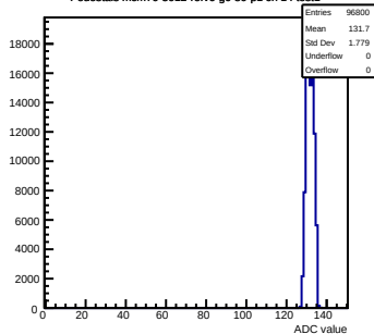
Pedestals mcm70-5012-rlv6-g0-s0-p1 ch 14 test1
