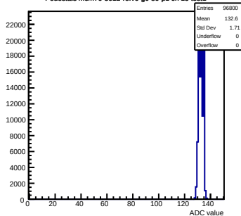
Pedestals mcm70-5012-rlv6-g0-s0-p1 ch 15 test1
