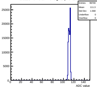
Pedestals mcm70-5012- rev6-g0-s0-p1 ch 88 test1
