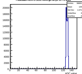
Pedestals mcm70-5012-refv6-g0-s0-p1 ch 73 test1
