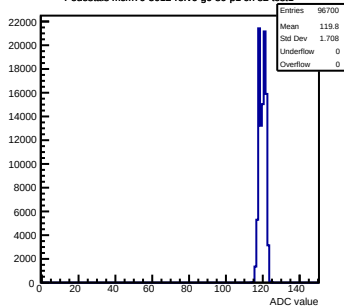
Pedestals mcm70-5012- rev6-g0-s0-p1 ch 82 test1
