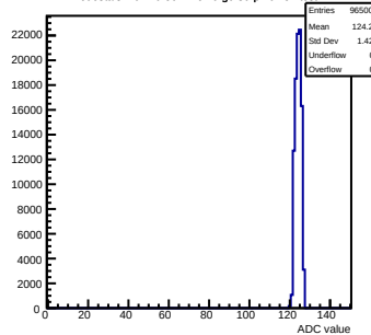
Pedestals mcm70-5012- refv6-g0-s0-p1 ch 54 test1
