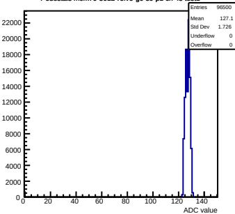
Pedestals mcm70-5012- refv6-g0-s0-p1 ch 48 test1
