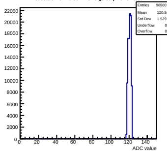
Pedestals mcm70-5012- refv6-g0-s0-p1 ch 57 test1
