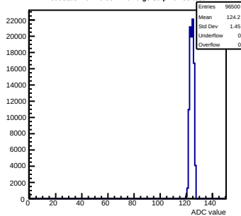
Pedestals mcm70-5012- refv6-g0-s0-p1 ch 53 test1
