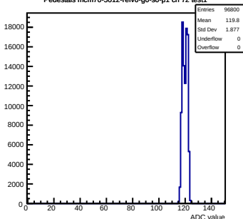
Pedestals mcm70-5012-refv6-g0-s0-p1 ch 72 test1
