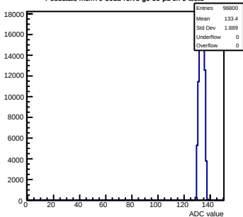
Pedestals mcm70-5012-rlv6-g0-s0-p1 ch 8 test1
