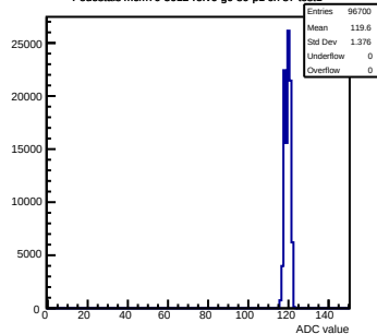
Pedestals mcm70-5012- rev6-g0-s0-p1 ch 87 test1
