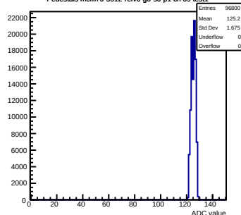
Pedestals mcm70-5012-refv6-g0-s0-p1 ch 69 test1
