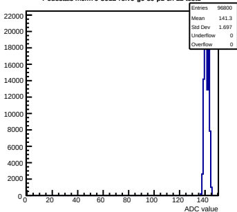
Pedestals mcm70-5012-rlv6-g0-s0-p1 ch 12 test1
