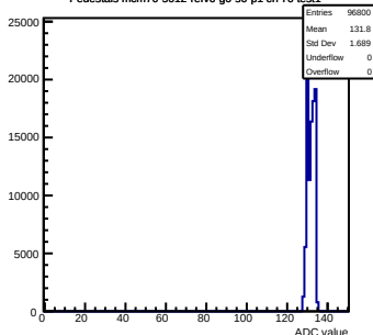
Pedestals mcm70-5012-refv6-g0-s0-p1 ch 70 test1
