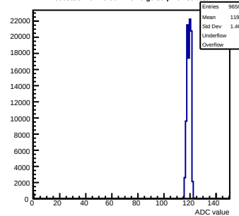
Pedestals mcm70-5012- refv6-g0-s0-p1 ch 55 test1
