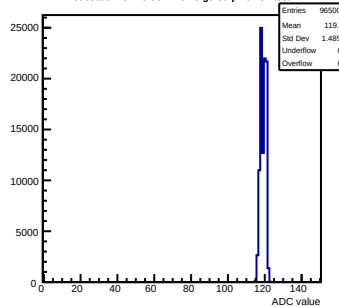
Pedestals mcm70-5012- refv6-g0-s0-p1 ch 62 test1
