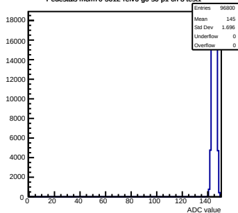
Pedestals mcm70-5012-rlv6-g0-s0-p1 ch 3 test1
