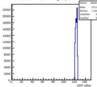
Pedestals mcm70-5012- refv6-g0-s0-p1 ch 61 test1
