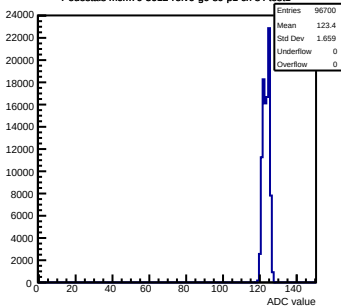
Pedestals mcm70-5012- rev6-g0-s0-p1 ch 84 test1
