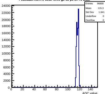
Pedestals mcm70-5012-refv6-g0-s0-p1 ch 71 test1
