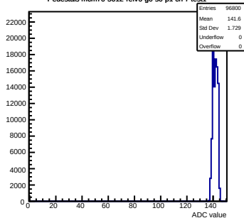
Pedestals mcm70-5012-rlv6-g0-s0-p1 ch 7 test1
