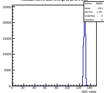
Pedestals mcm70-5012-rlv6-g0-s0-p1 ch 1 test1
