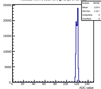
Pedestals mcm70-5012- rev6-g0-s0-p1 ch 85 test1
