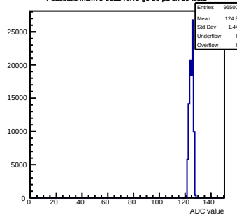
Pedestals mcm70-5012- refv6-g0-s0-p1 ch 50 test1
