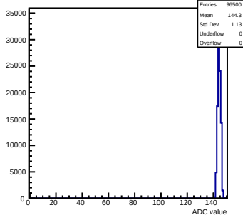
Pedestals mcm71-6A16-refV0-g0-s0-p1 ch 118 test1
