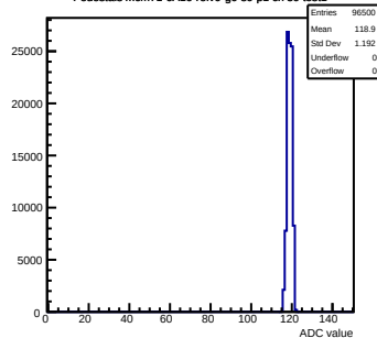
Pedestals mcm71-6A16-refV0-g0-s0-p1 ch 59 test1
