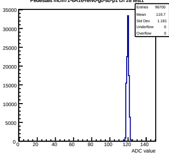
Pedestals mcm71-6A16-refV0-g0-s0-p1 ch 28 test1
