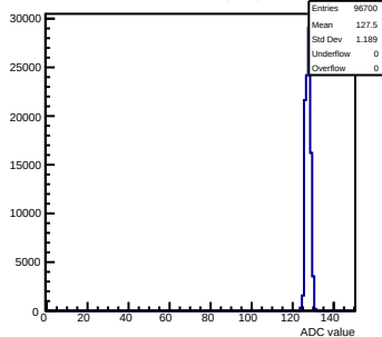
Pedestals mcm71-6A16-refV0-g0-s0-p1 ch 85 test1
