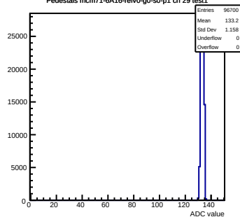
Pedestals mcm71-6A16-refV0-g0-s0-p1 ch 29 test1
