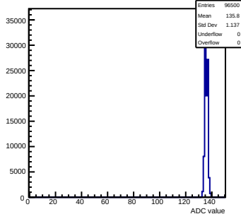
Pedestals mcm71-6A16-refV0-g0-s0-p1 ch 122 test1
