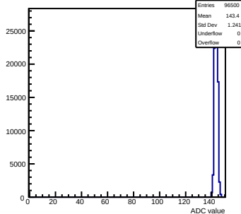
Pedestals mcm71-6A16-refV0-g0-s0-p1 ch 127 test1
