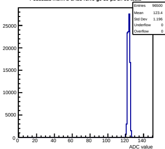
Pedestals mcm71-6A16-refV0-g0-s0-p1 ch 60 test1
