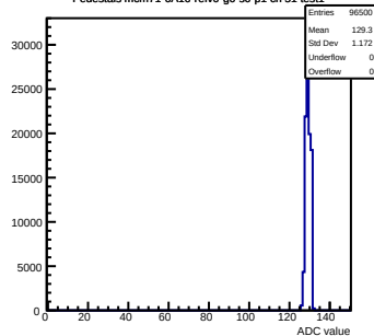
Pedestals mcm71-6A16-refV0-g0-s0-p1 ch 51 test1
