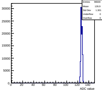
Pedestals mcm71-6A16-refV0-g0-s0-p1 ch 116 test1
