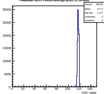
Pedestals mcm71-6A16-refV0-g0-s0-p1 ch 26 test1
