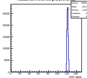
Pedestals mcm71-6A16-refV0-g0-s0-p1 ch 55 test1
