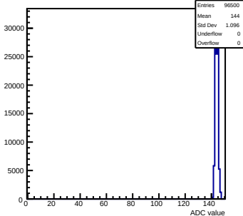
Pedestals mcm71-6A16-refV0-g0-s0-p1 ch 124 test1
