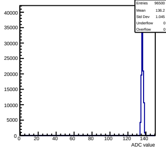
Pedestals mcm71-6A16-refV0-g0-s0-p1 ch 119 test1
