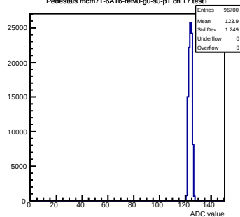
Pedestals mcm71-6A16-refV0-g0-s0-p1 ch 17 test1
