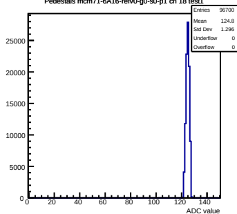
Pedestals mcm71-6A16-refV0-g0-s0-p1 ch 18 test1
