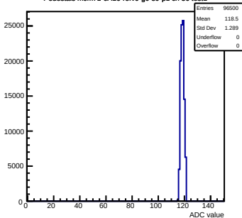
Pedestals mcm71-6A16-refV0-g0-s0-p1 ch 56 test1
