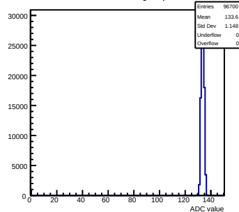
Pedestals mcm71-6A16-refV0-g0-s0-p1 ch 90 test1
