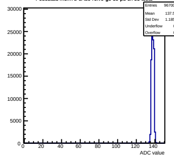
Pedestals mcm71-6A16-refV0-g0-s0-p1 ch 83 test1
