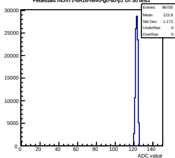
Pedestals mcm71-6A16-refV0-g0-s0-p1 ch 30 test1
