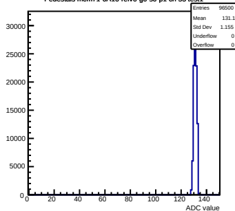
Pedestals mcm71-6A16-refV0-g0-s0-p1 ch 53 test1
