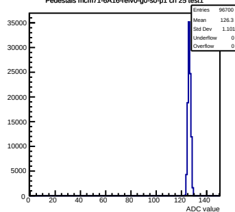
Pedestals mcm71-6A16-refV0-g0-s0-p1 ch 25 test1
