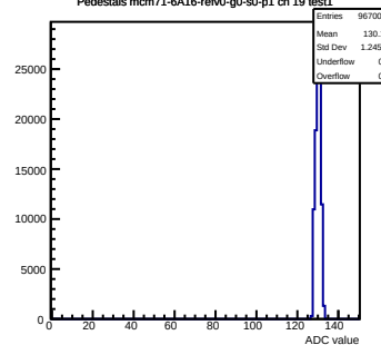
Pedestals mcm71-6A16-refV0-g0-s0-p1 ch 19 test1
