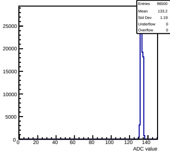
Pedestals mcm71-6A16-refV0-g0-s0-p1 ch 120 test1
