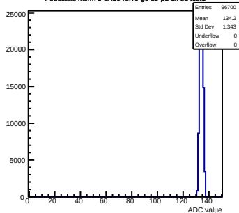
Pedestals mcm71-6A16-refV0-g0-s0-p1 ch 81 test1
