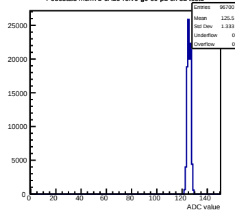
Pedestals mcm71-6A16-refV0-g0-s0-p1 ch 82 test1
