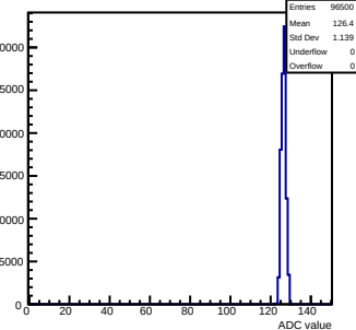
Pedestals mcm71-6A16-refV0-g0-s0-p1 ch 117 test1
