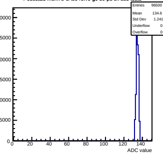
Pedestals mcm71-6A16-refV0-g0-s0-p1 ch 113 test1
