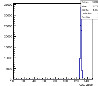
Pedestals mcm71-6A16-refV0-g0-s0-p1 ch 95 test1
