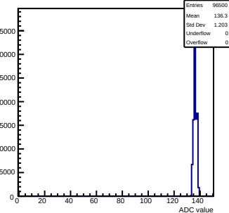
Pedestals mcm71-6A16-refV0-g0-s0-p1 ch 125 test1
