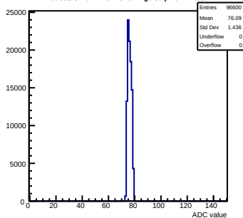
Pedestals mcm71-6A16-refv2-g0-s0-p1 ch 42 test1
