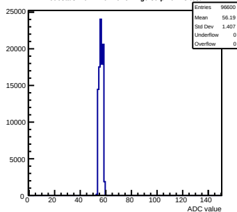
Pedestals mcm71-6A16-refv2-g0-s0-p1 ch 45 test1
