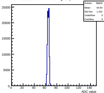
Pedestals mcm71-6A16-refv2-g0-s0-p1 ch 44 test1
