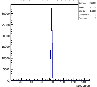
Pedestals mcm71-6A16-refv2-g0-s0-p1 ch 32 test1
