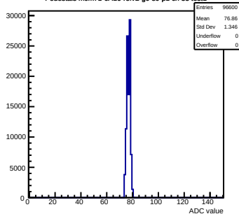
Pedestals mcm71-6A16-refv2-g0-s0-p1 ch 33 test1
