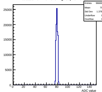
Pedestals mcm71-6A16-refv2-g0-s0-p1 ch 43 test1
