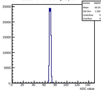
Pedestals mcm71-6A16-refv2-g0-s0-p1 ch 41 test1
