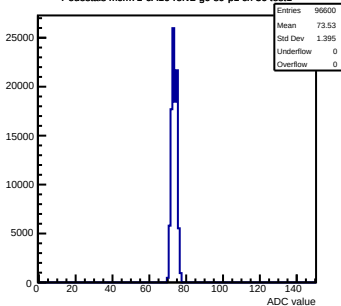
Pedestals mcm71-6A16-refv2-g0-s0-p1 ch 36 test1
