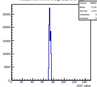
Pedestals mcm71-6A16-refv2-g0-s0-p1 ch 37 test1
