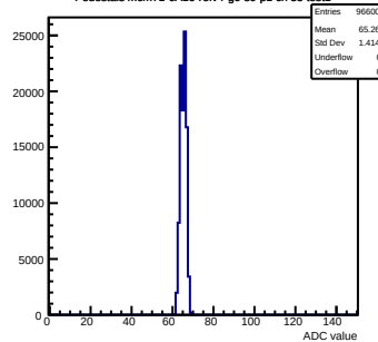
Pedestals mcm71-6A16-refv4-g0-s0-p1 ch 35 test1
