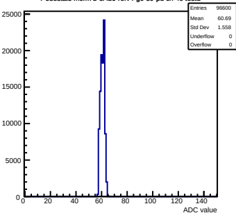
Pedestals mcm71-6A16-refv4-g0-s0-p1 ch 40 test1
