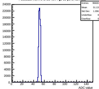
Pedestals mcm71-6A16-refv4-g0-s0-p1 ch 38 test1
