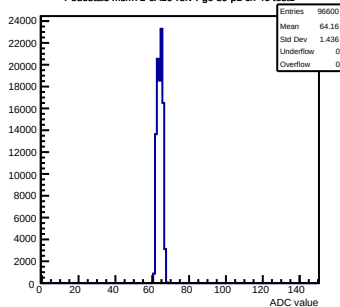
Pedestals mcm71-6A16-refv4-g0-s0-p1 ch 46 test1
