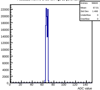
Pedestals mcm71-6A16-refv4-g0-s0-p1 ch 32 test1
